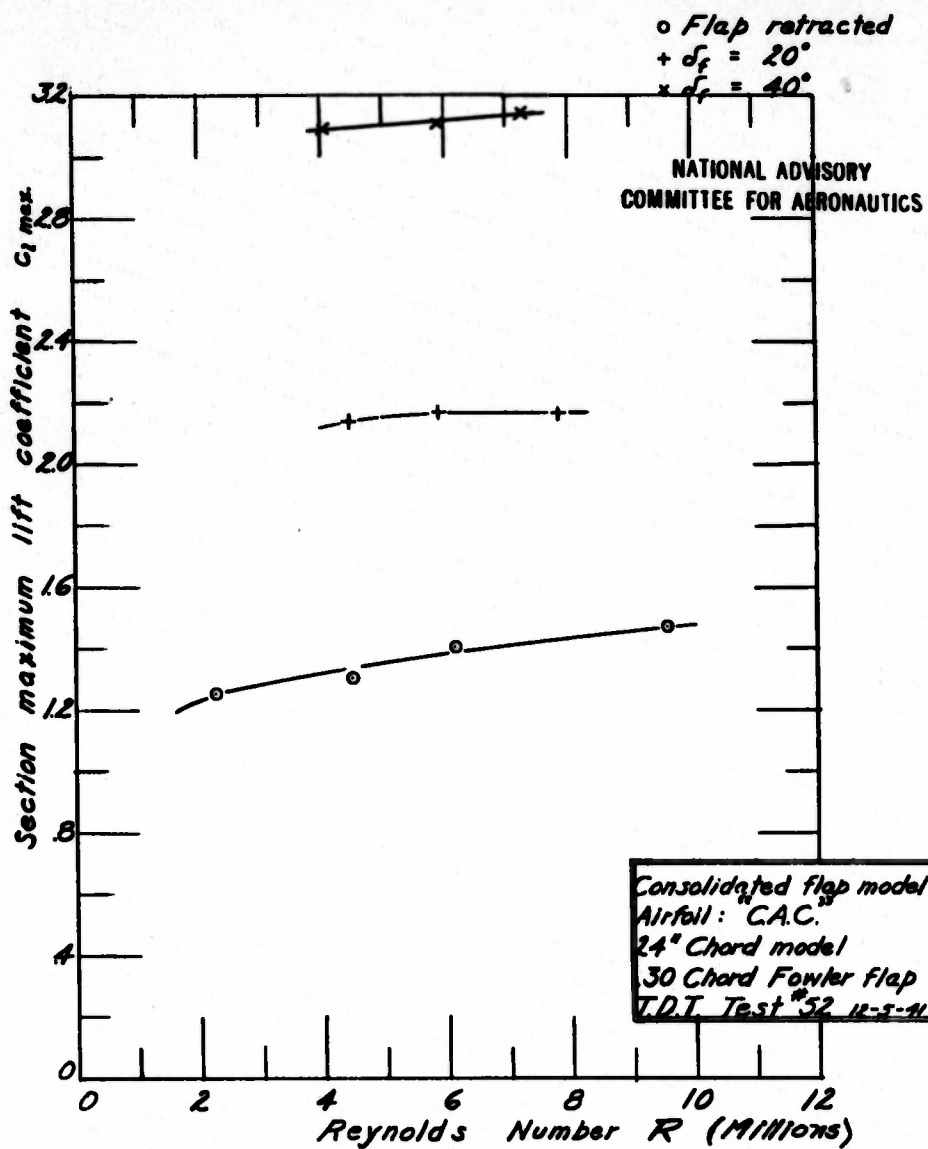
Figure 8 Variation of maximum lift with Reynolds Number
