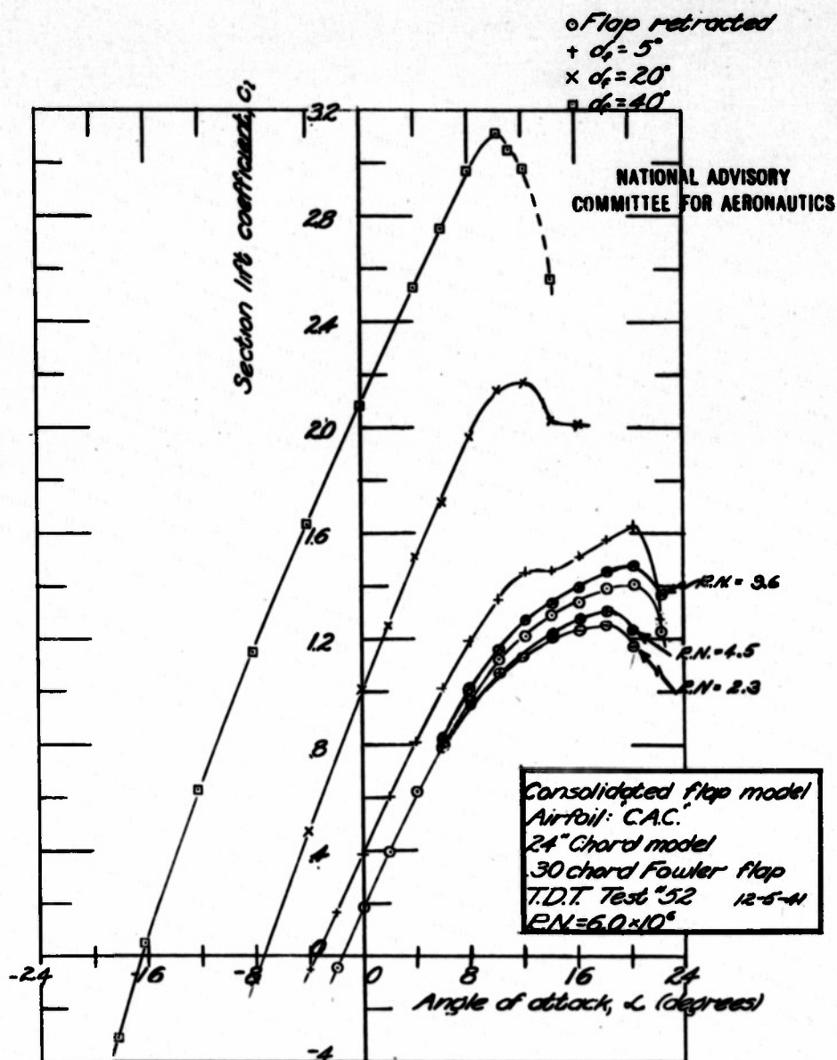
FIG 7.-Variation of section lift coefficient with angle of attack.
