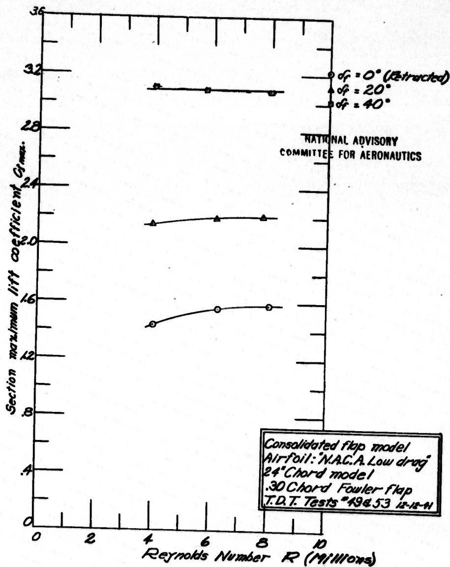
Figure 11.- Variation of maximum lift coefficient with Reynolds Number.
