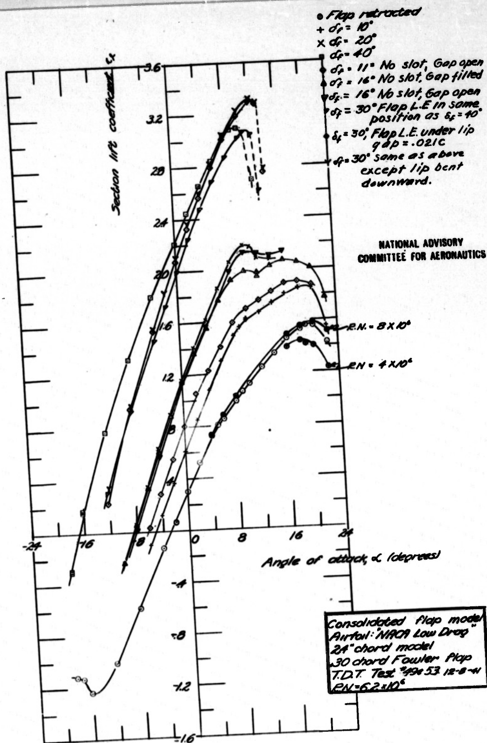
Figure 10.- Variation of section lift coefficient with angle of attack.
