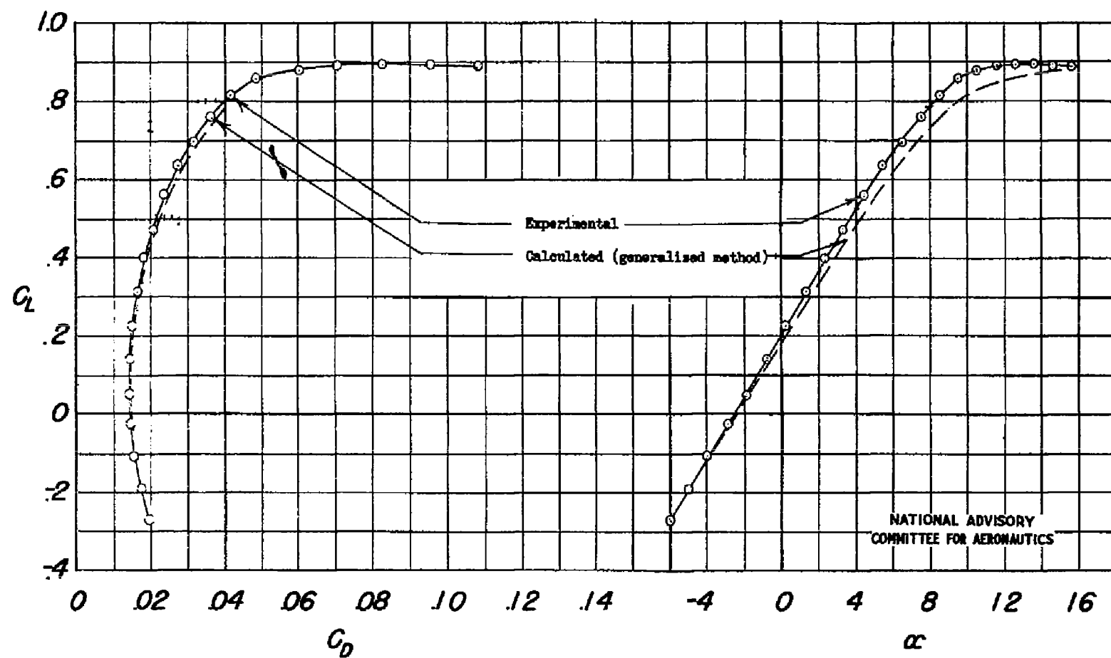
Figure 13.- Experimental and calculated characteristics of wing 2.5-12-44,24 with rough leading edge. R = 3.9 \times 10^6 .
