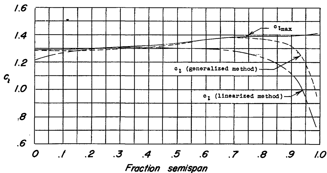
(a) Wing 2.5-12-44,24.
