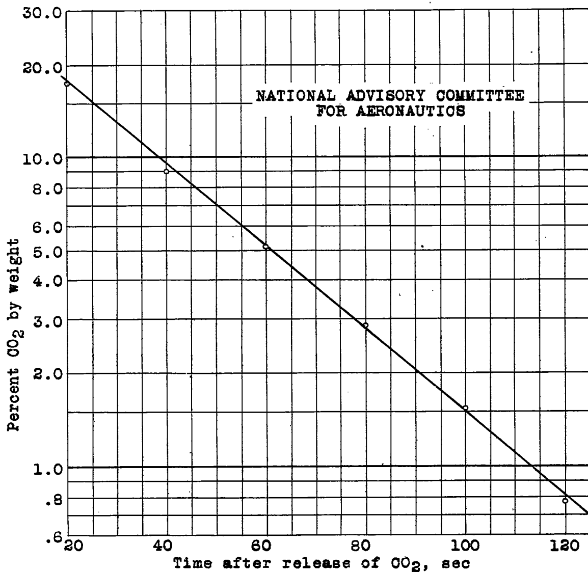
Figure 7.- Variation of the carbon-dioxide concentration by weight with time after a quantity of carbon-dioxide was released in the cabin. Pressure altitude, 6000 feet; indicated airspeed, 70 miles per hour.
