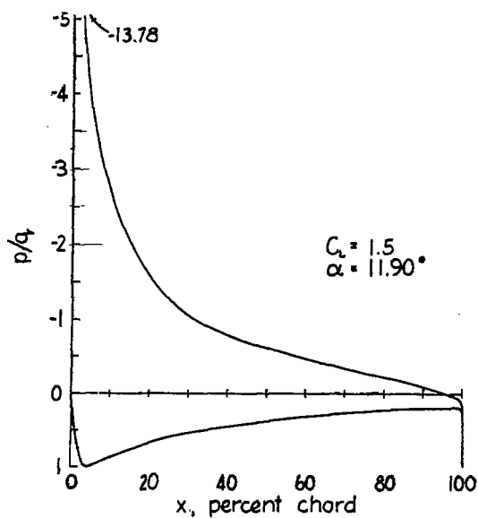
Figure 12.- Shape and pressure distribution for NACA 23006 airfoil.
