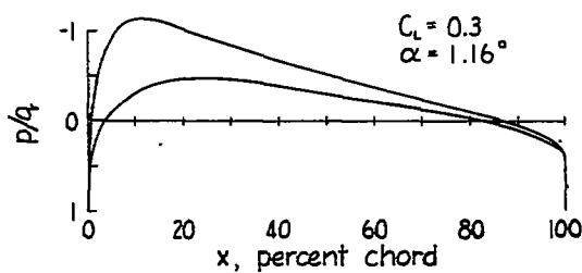
Figure 17.- Shape and pressure distribution for NACA 23021 airfoil.
