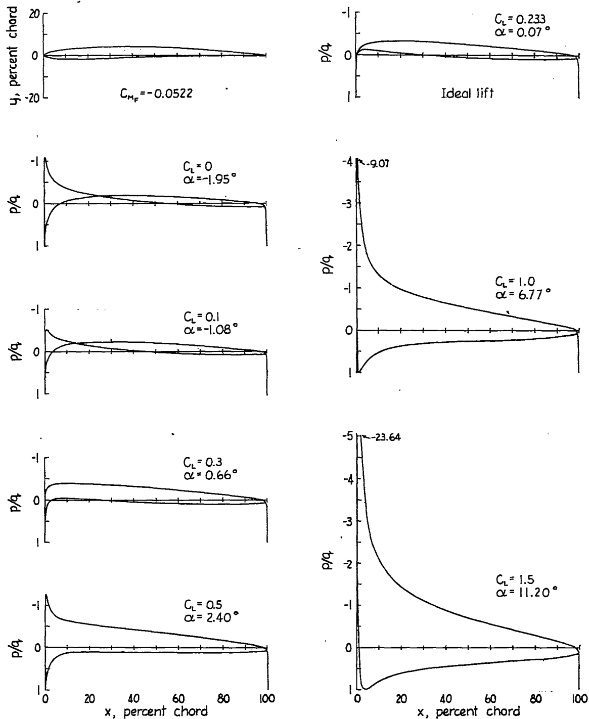
Figure 35.- Shape and pressure distribution for synthetic airfoil; \psi = 0.05 + 0.05 \cos(\psi - 45^\circ) .
