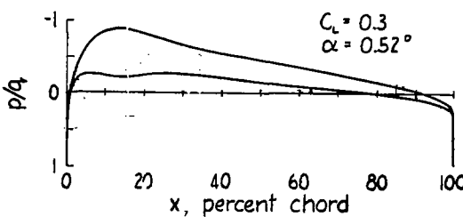
Figure 4.- Shape and pressure distribution for NACA 2215 airfoil.
