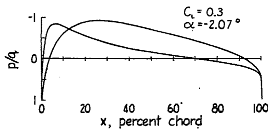
Figure 11.-Shape and pressure distribution for NACA 4421 airfoil.
