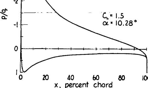
Figure 4.- Shape and pressure distribution for NACA 2215 airfoil.
