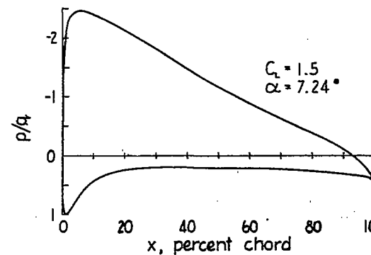
Figure 11.-Shape and pressure distribution for NACA 4421 airfoil.
