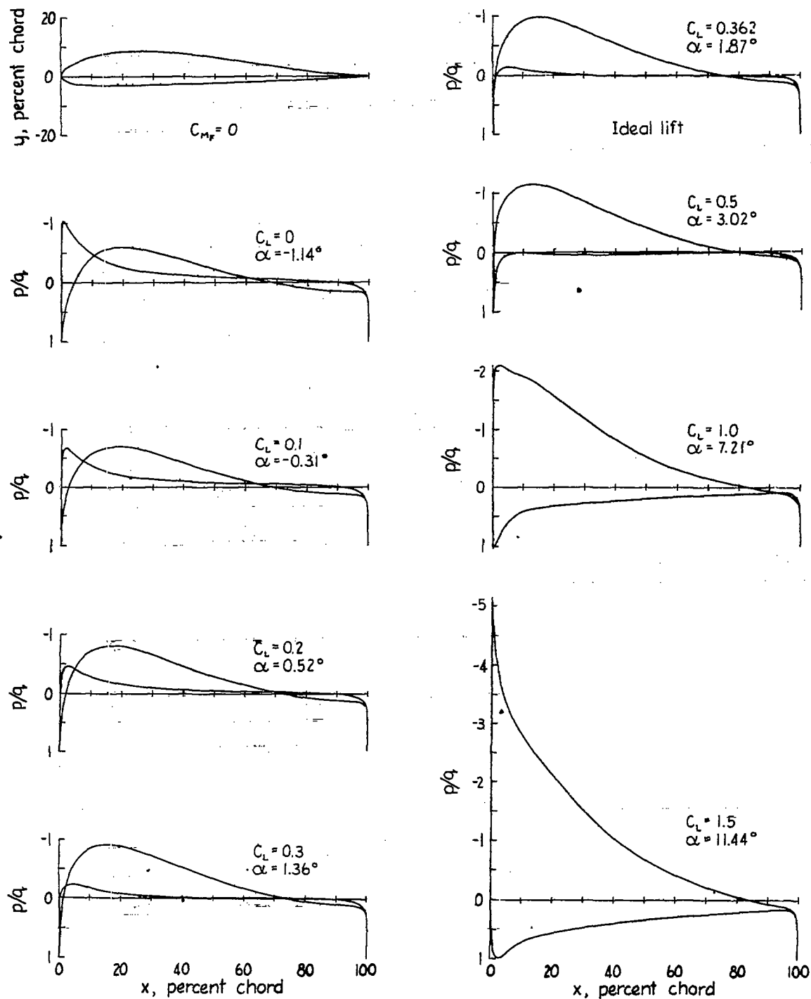
Figure 44.- Shape and pressure distribution for synthetic airfoil; \psi = 0.0996 + 0.1 \cos(\phi - 30^\circ) + 0.0284 \sin 2\phi .
