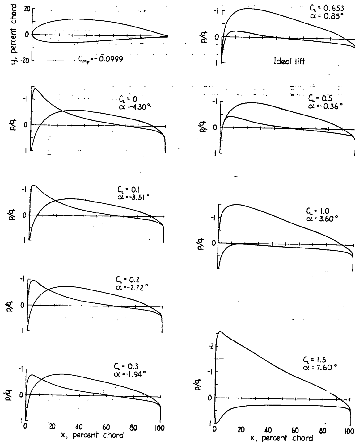
Figure 10.- Shape and pressure distribution for NACA 4418 airfoil.
