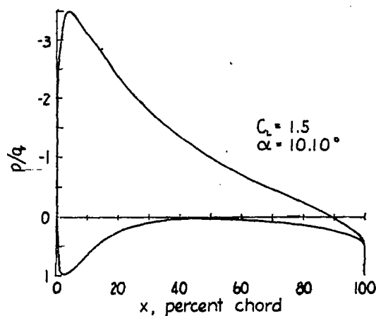
Figure 18.- Shape and pressure distribution for NACA 23025 airfoil.
