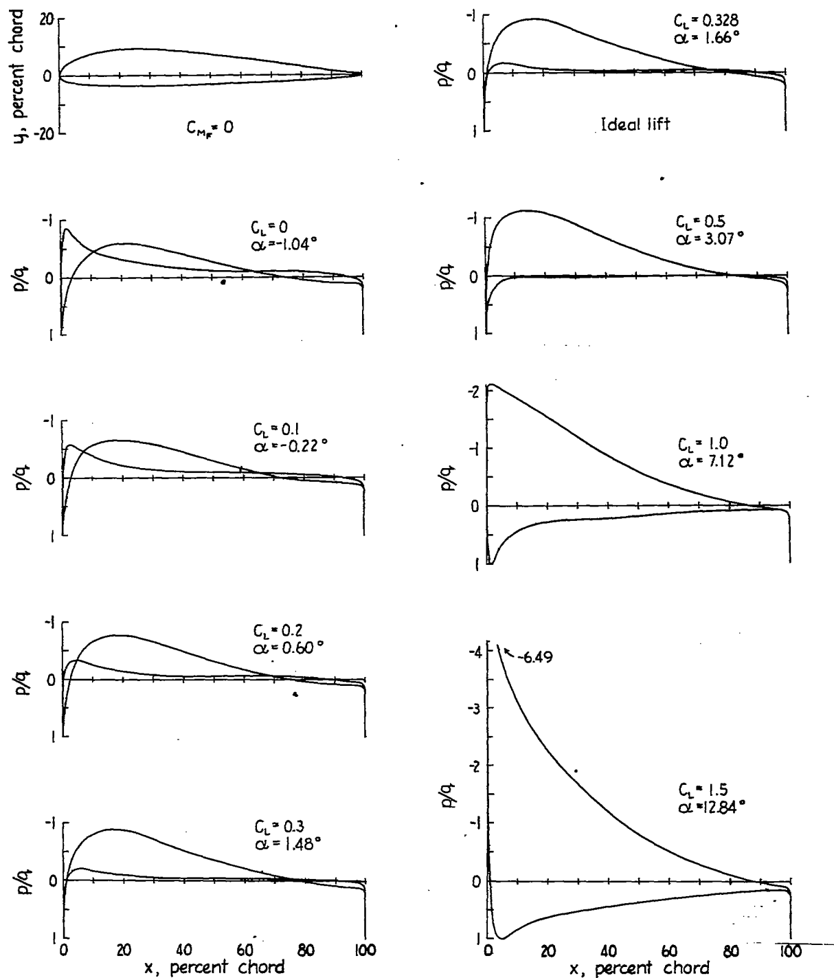
Figure 43.- Shape and pressure distribution for synthetic airfoil;
