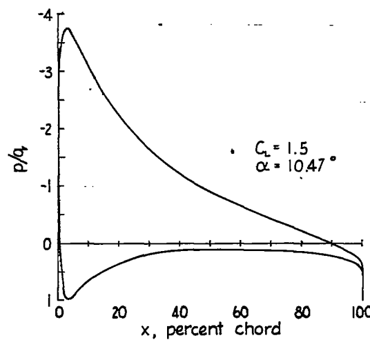
Figure 17.- Shape and pressure distribution for NACA 23021 airfoil.
