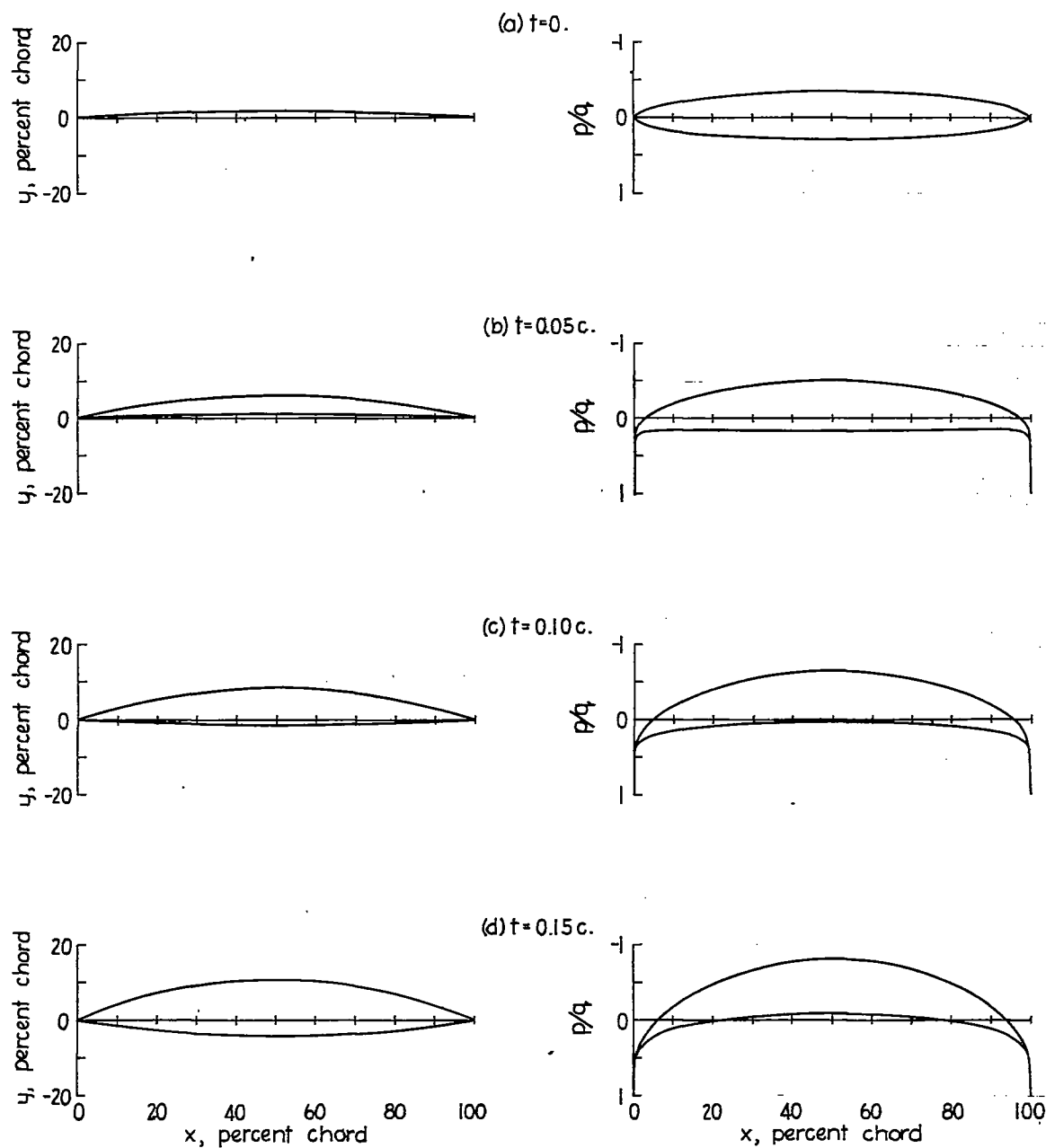
Figure 33.- Shape and pressure distribution for circular-arc airfoils of various thicknesses. C_L=0.5 .
