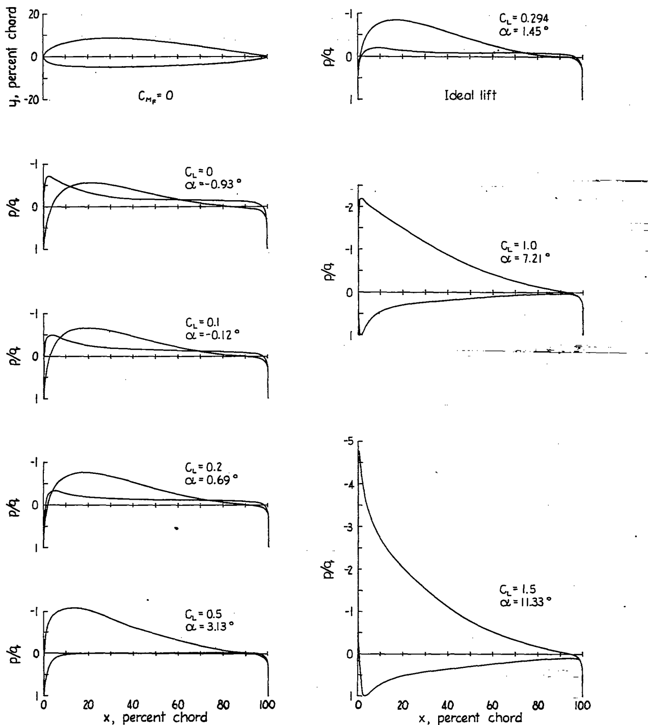
Figure 47.- Shape and pressure distribution for synthetic airfoil;
