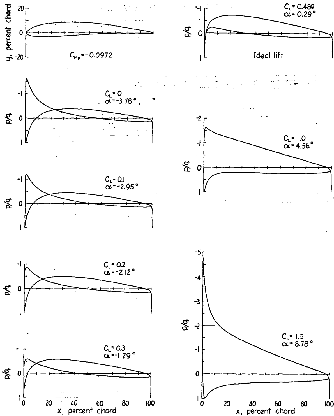
Figure 38.- Shape and pressure distribution for synthetic airfoil; \psi = 0.1 + 0.1 \cos(\psi - 45^\circ) .
