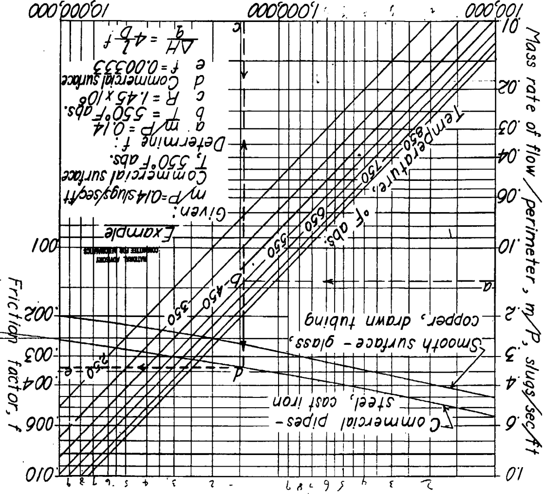
(b) Reynolds number, 100,000 to 10,000,000 Figure 1. - Concluded.
