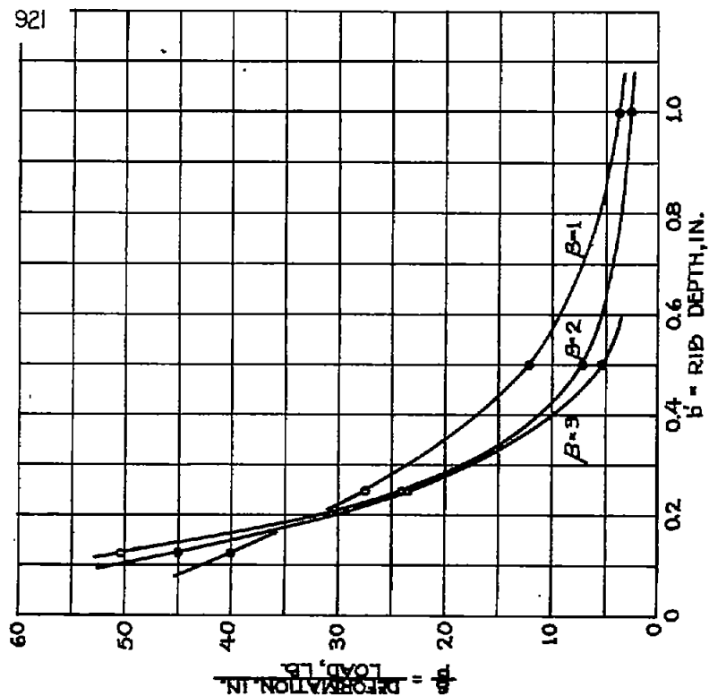
FIG. 9.-RIB BOWING, SPECIMEN 1T, k = 10 \frac{1}{4} IN
