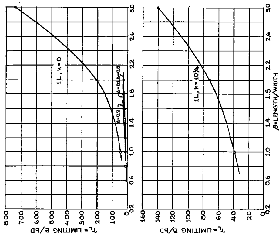
FIG. 16.-DEFORMATION UNDER COMPRESSIVE LOADING
