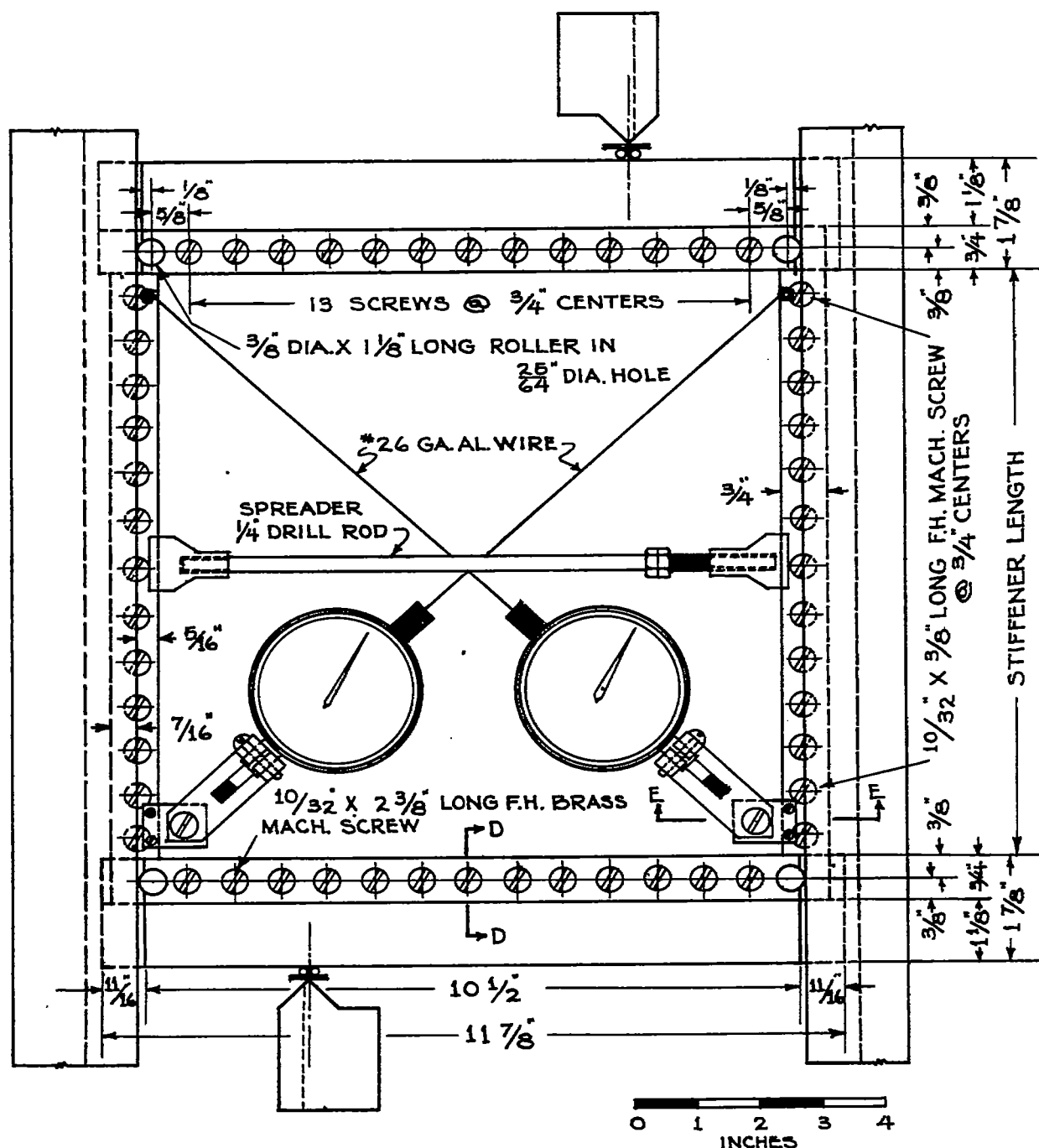
FIG. 3. - MOUNTING OF SHEET PANEL
