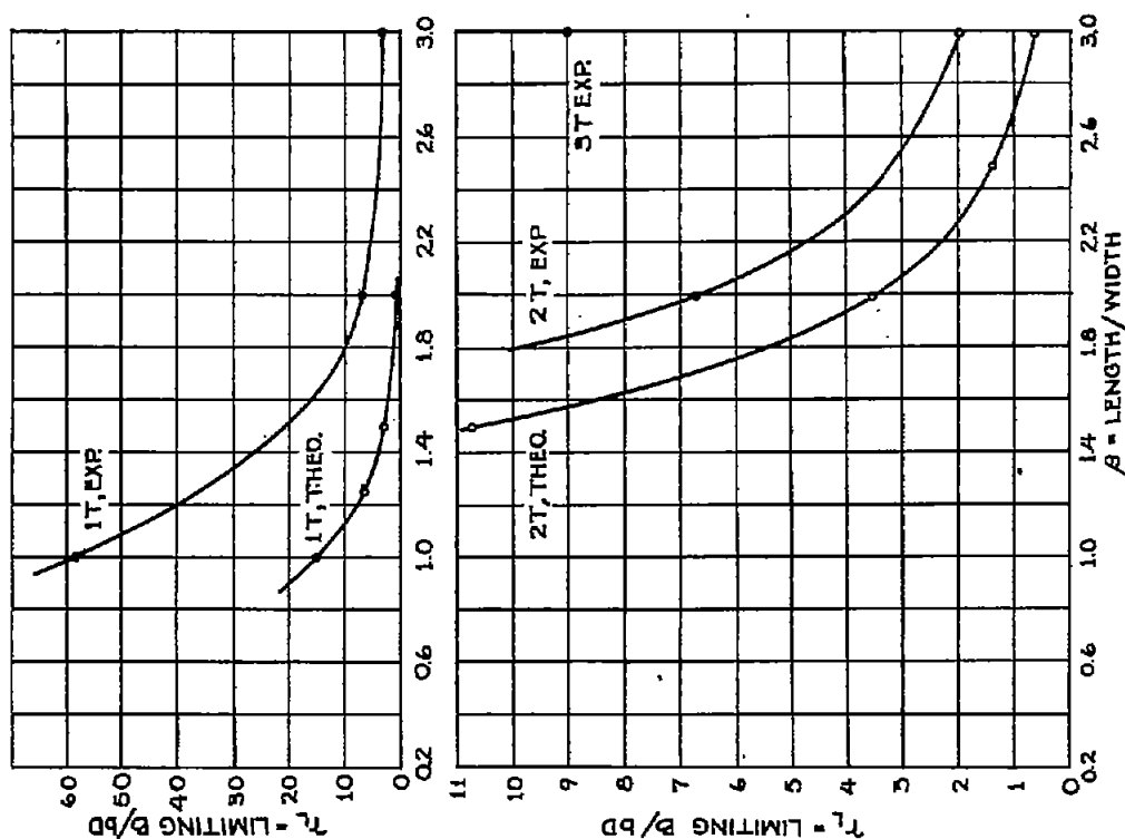
FIG. 15.-DEFORMATION UNDER SHEAR LOADING, k = 10^{-4}
