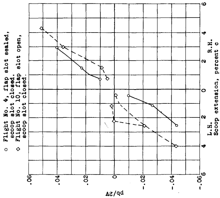
Figure 15.- Rate of roll at 100 mph, ( C_L = 1.57 ) flaps and gear down.
