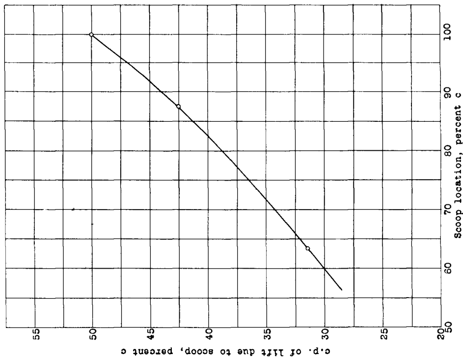
Figure 9.- Center of pressure of scoop lift at \alpha = 0^\circ .
