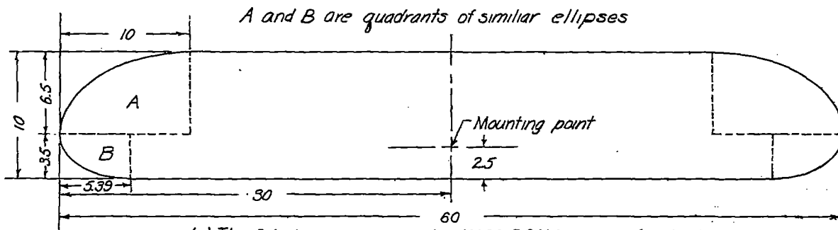
(a) The 5-foot-span rectangular NACA 23012 wing; A = 6.38 .
