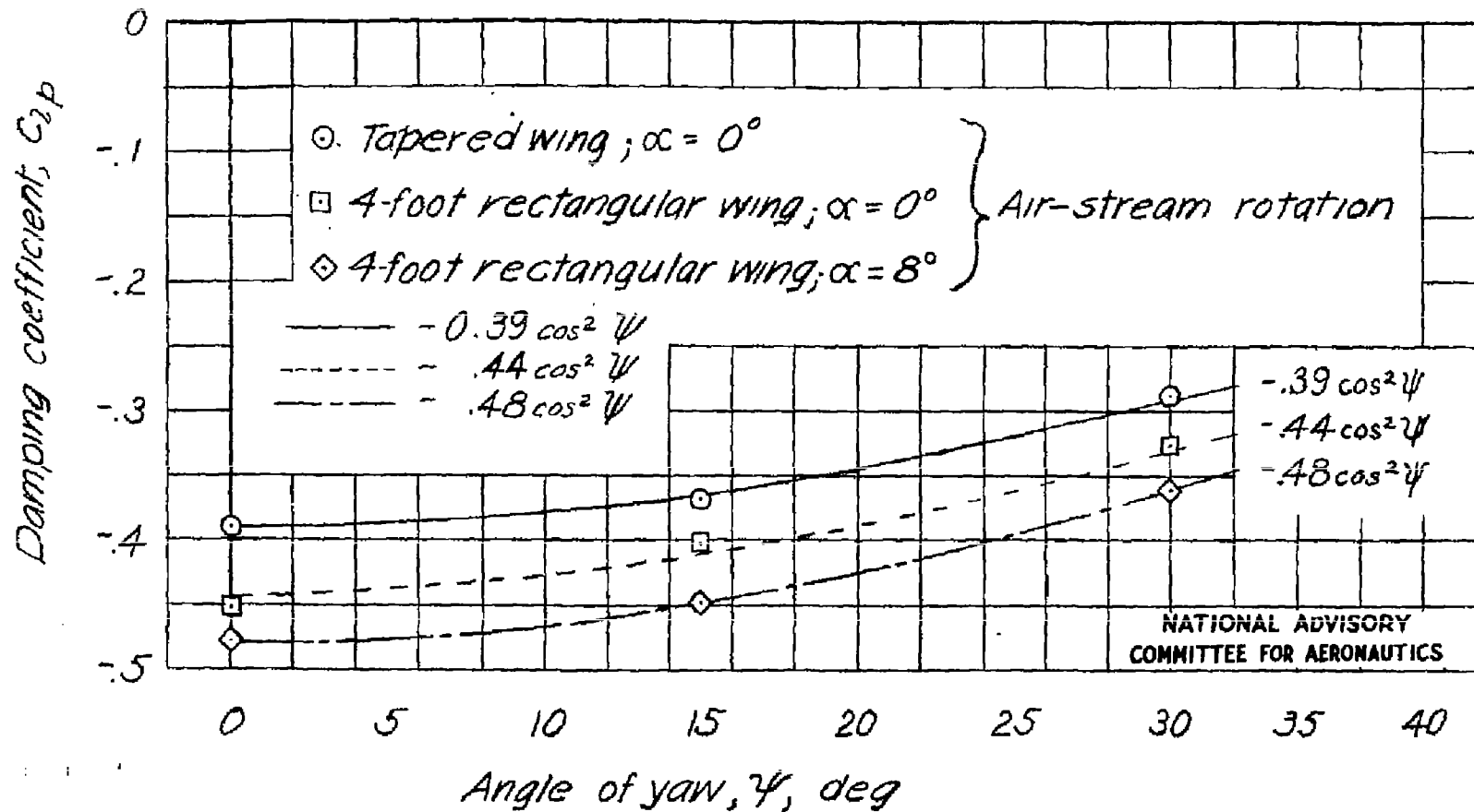
Figure 11.- Variation of damping in roll with angle of yaw.
