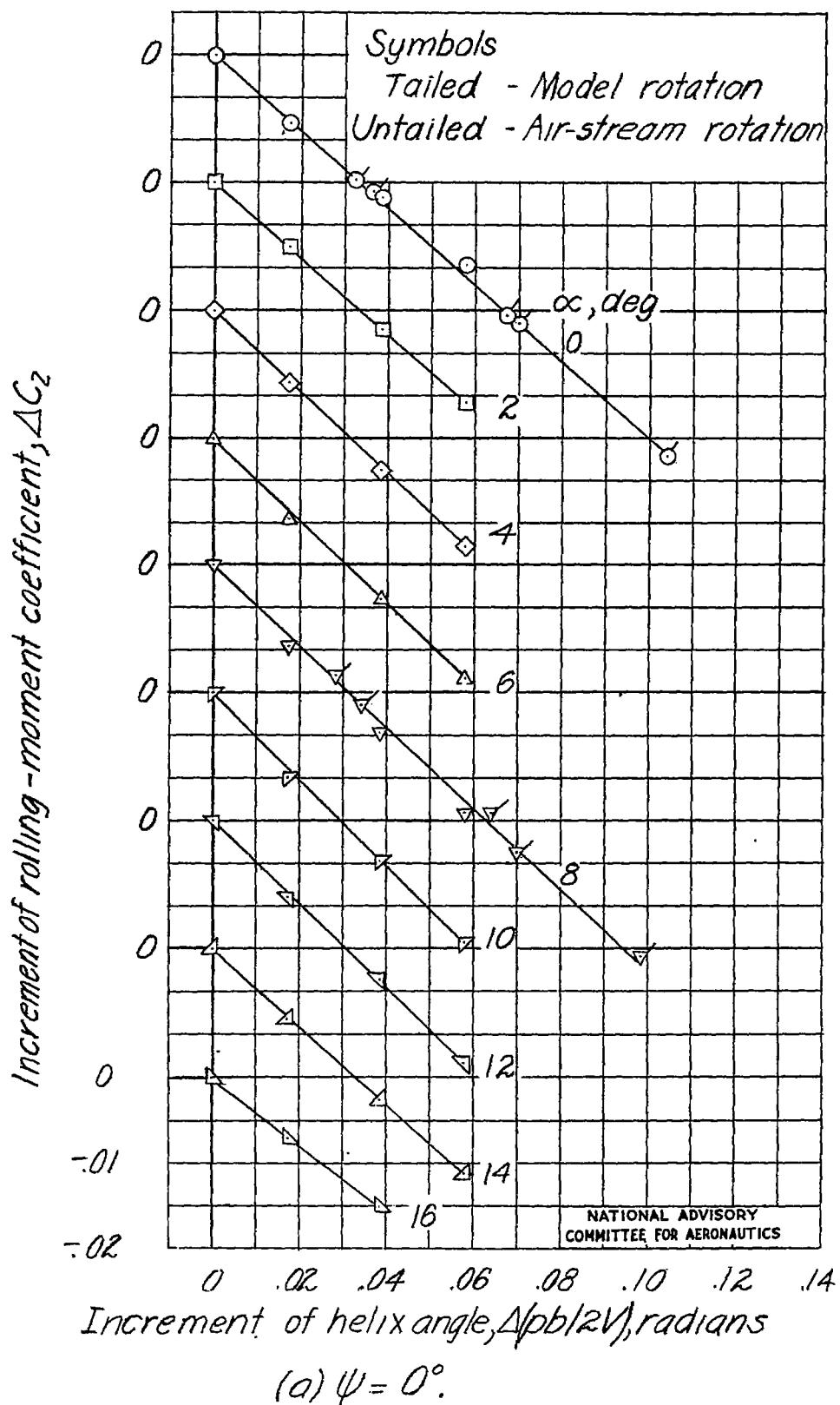
Figure 6.- Variation of rolling-moment coefficient with wing-tip helix angle. Four-foot-span rectangular wing.
