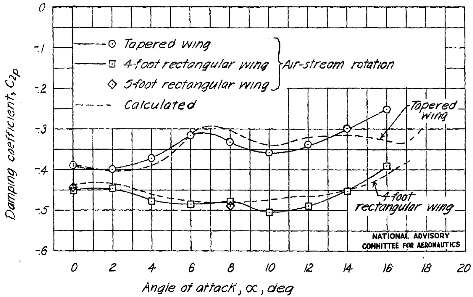
Figure 9.- Variation of damping in roll with angle of attack. \psi = 0^\circ .
