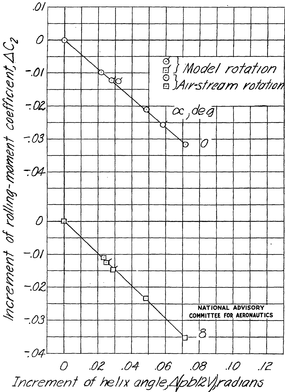
Figure 7.- Variation of rolling-moment coefficient with wing-tip helix angle. Five-foot-span rectangular wing; \psi = 0^\circ .
