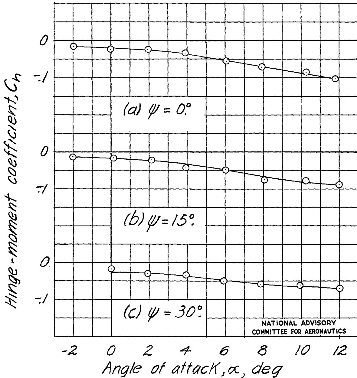
Figure 12.- Variation of aileron hinge-moment coefficient with angle of attack. Tapered wing; \delta_a = 0^\circ ; \frac{pb}{2V} = 0 .
