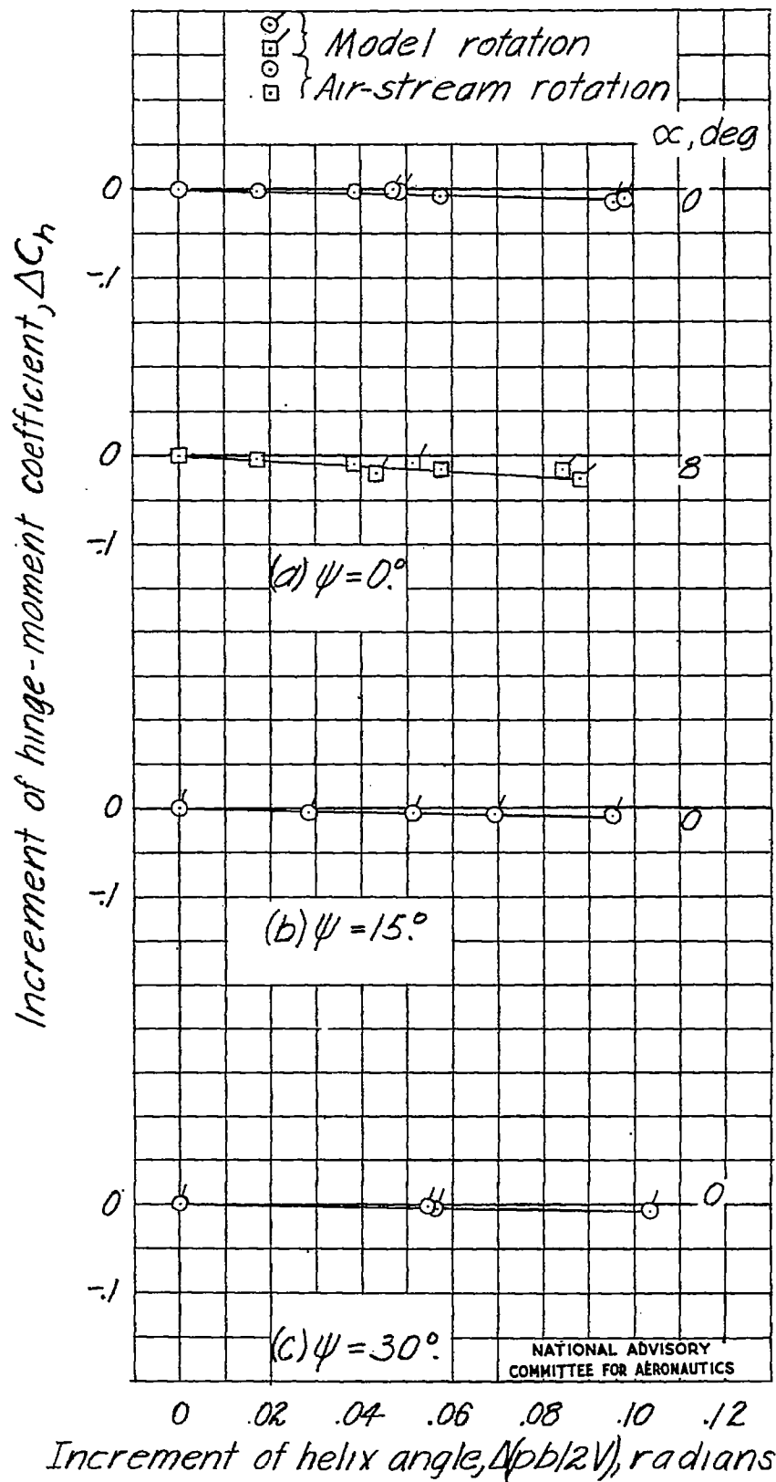
Figure 8.- Variation of aileron hinge-moment coefficient with wing-tip helix angle. Tapered wing; \delta_a = 0^\circ .
