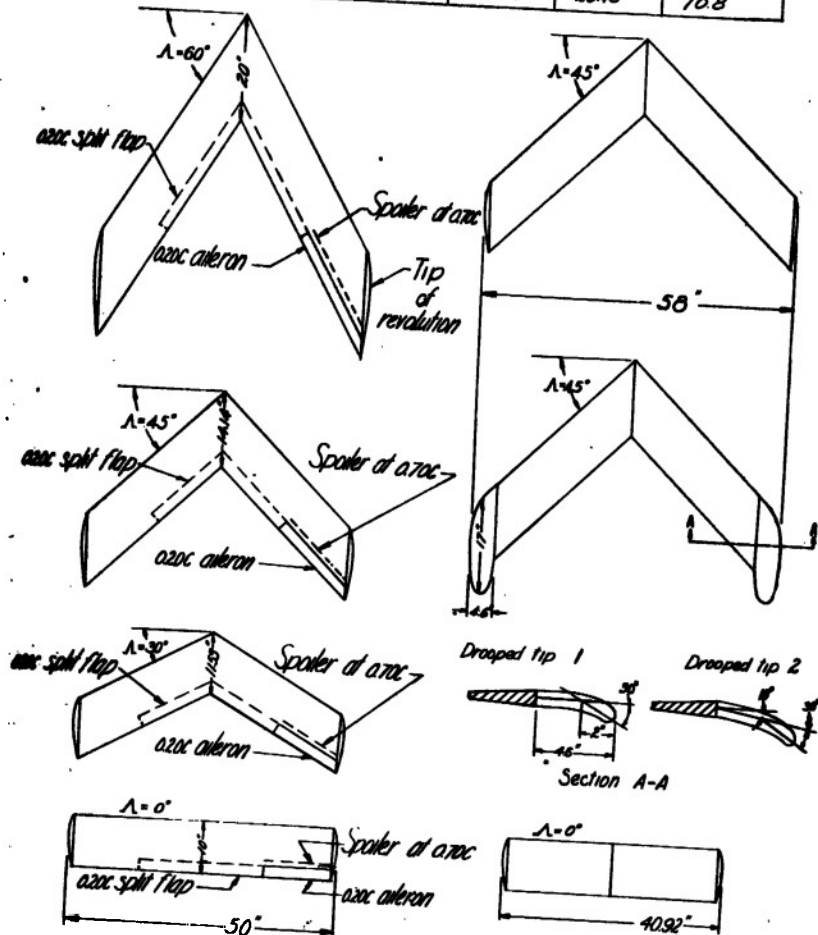
Figure 1.-Plan forms of swept-back wings.
