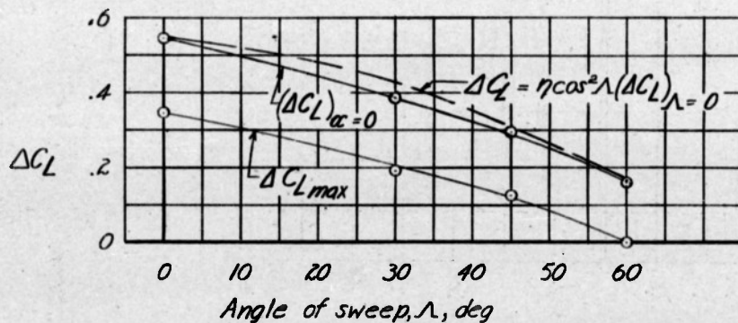
Figure 42.- Variation with sweepback of the estimated and experimental values of \Delta C_L resulting from a split-flap deflection of 60°.
