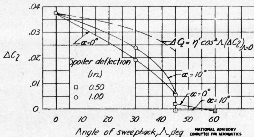
Figure 41.- Variation with sweepback of the estimated and experimental values of \Delta C_z resulting from spoiler deflection.
