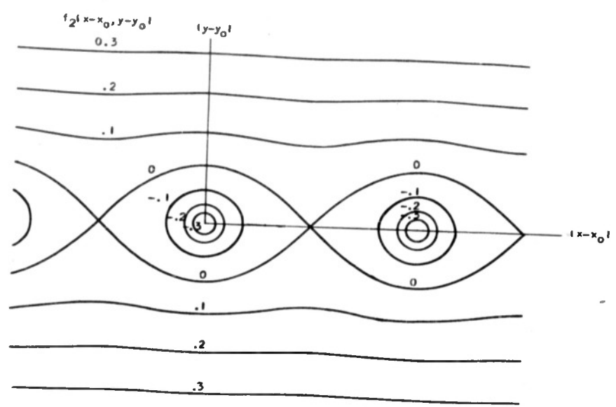
Figure 2. - Plot of curves for constant f_2(x-x_0, y-y_0) .
