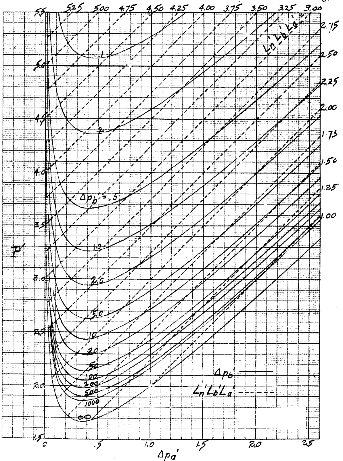
Figure 1 - Generalized selection chart for tubular intercoolers.
