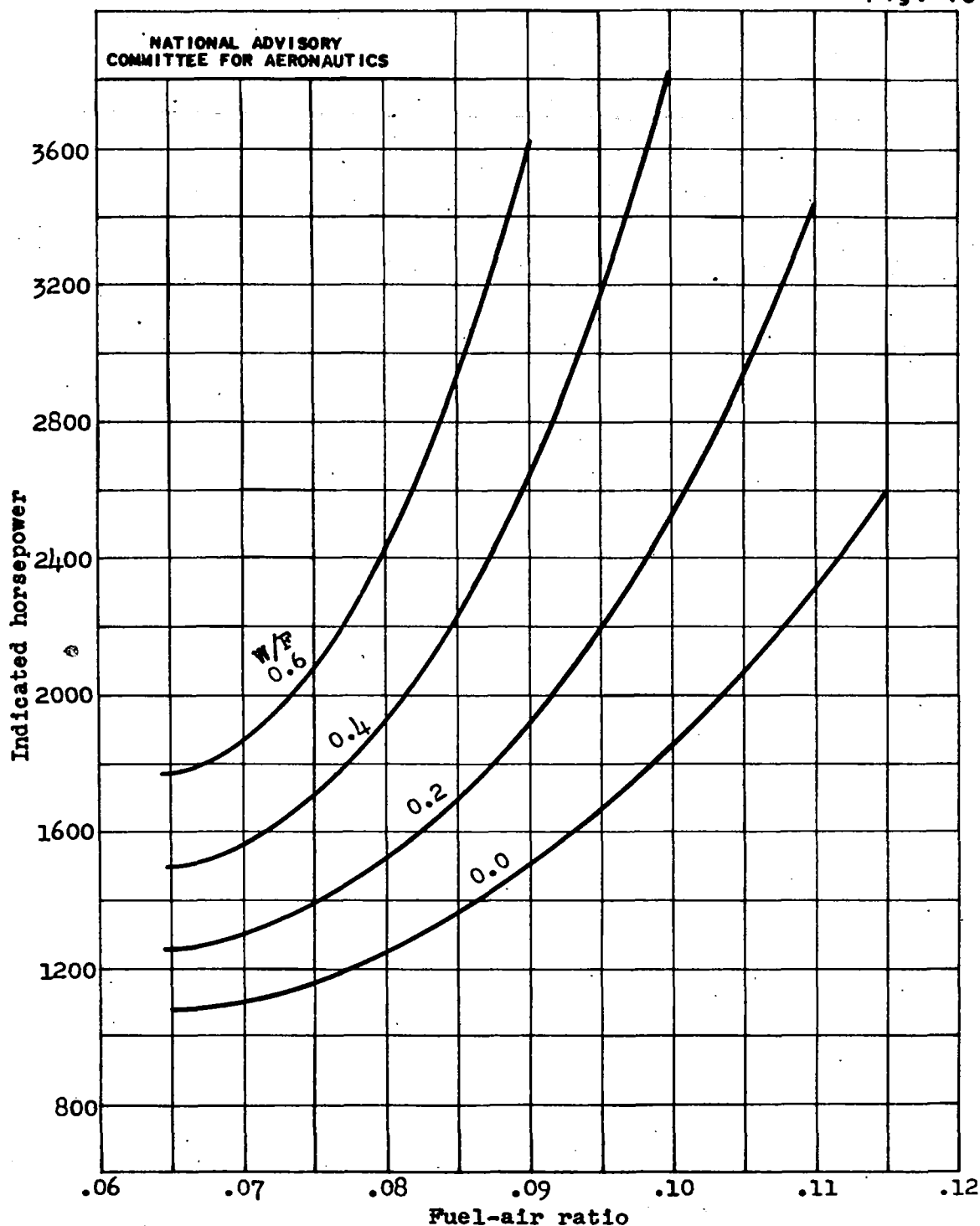
Figure 18. - Relation between fuel-air ratio and temperature-limited horsepower at different water-fuel ratios. Wright R-2600-8 engine; cooling-air pressure drop, 7 inches of water; average rear spark-plug-gasket temperature, 425^{\circ} F; carburetor-air temperature, 90^{\circ} F; cooling-air temperature, 90^{\circ} F; engine speed, 2600 rpm.
