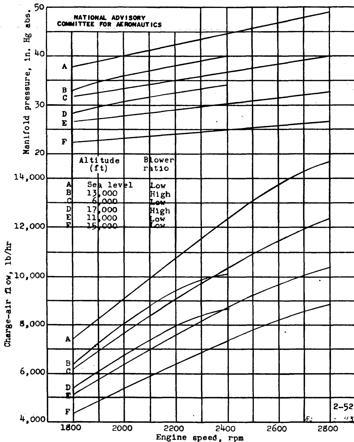
Figure 17. - Capacity of supercharger of Wright R-2600-8 engine in terms of air flow and manifold pressure at standard altitude. Data from Naval Air Materiel Center, Naval Air Experimental Station.
