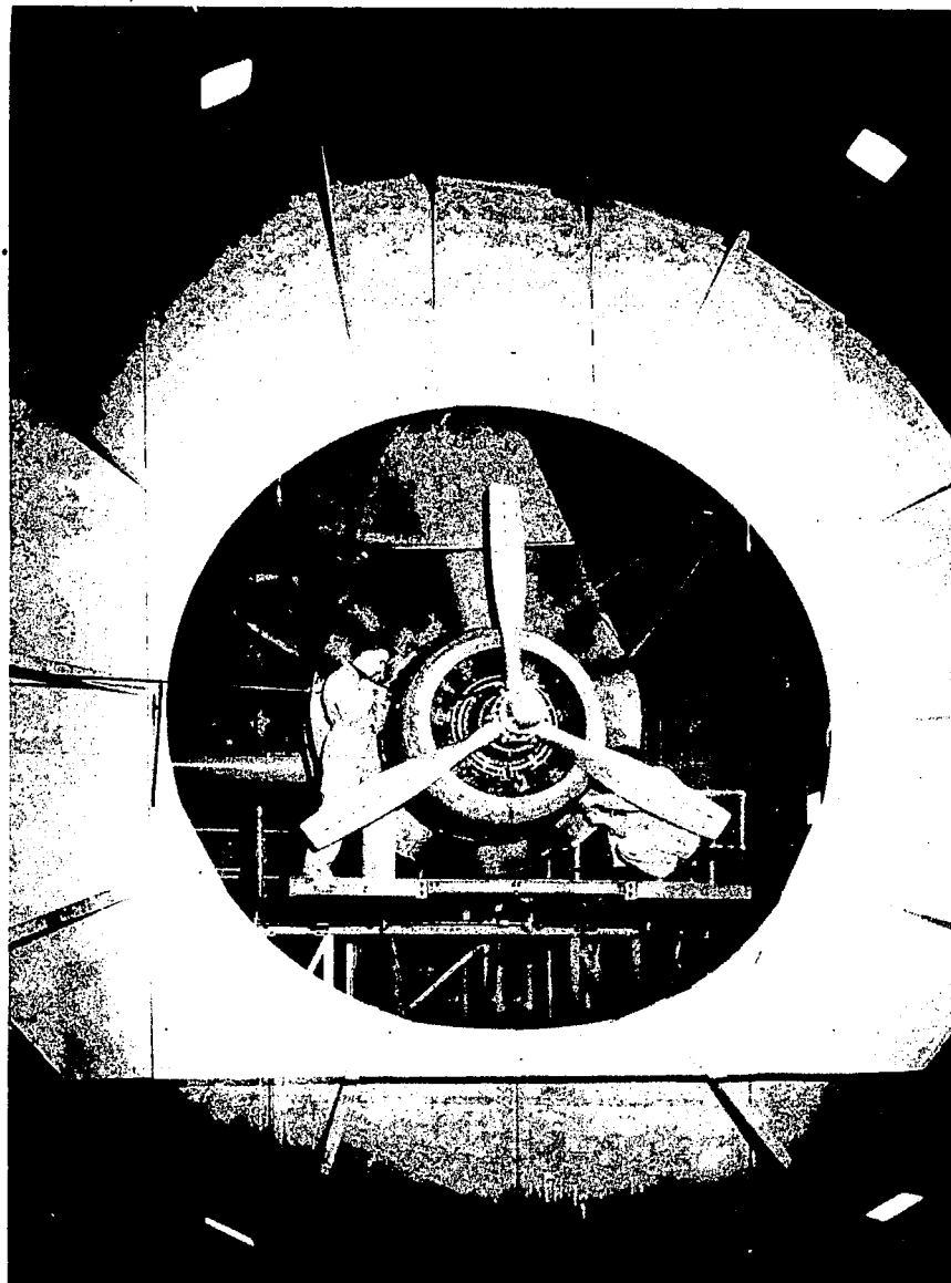
Figure 1. - Front view of Wright R-2600-8 engine installation.
