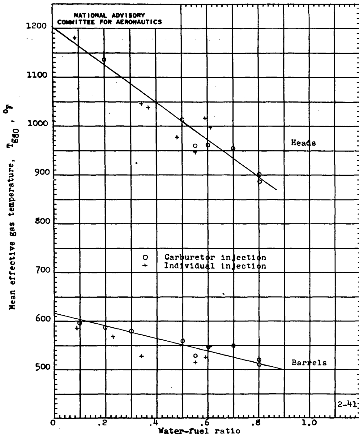
Figure 12. - Variation of mean effective gas temperature T_{g80} with water-fuel ratio for cylinder heads and barrels. Wright R-2600-8 engine.
