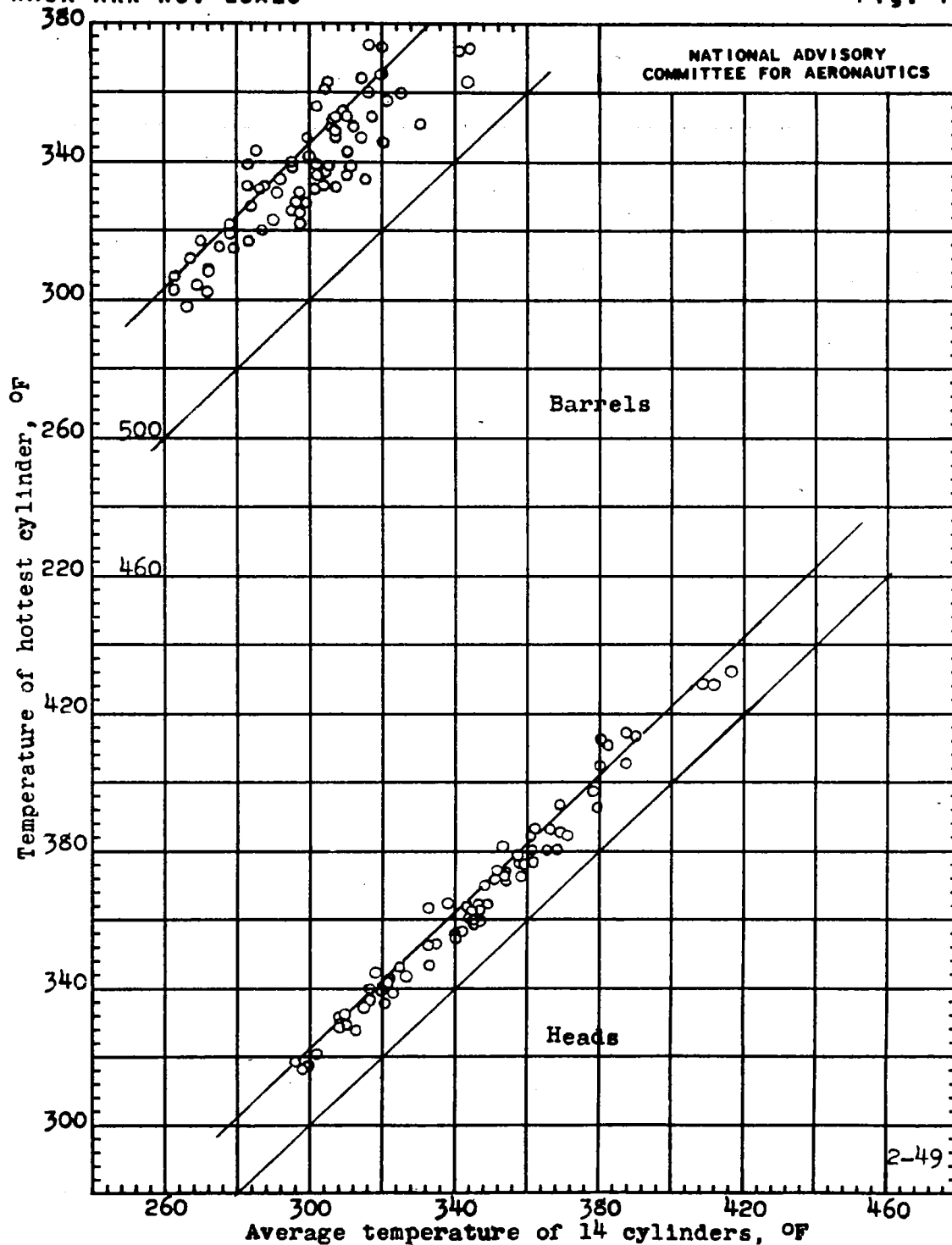
Figure 16.- Variation of hottest cylinder temperatures with average temperatures of 14 cylinders. Wright R-2600-8 engine.
