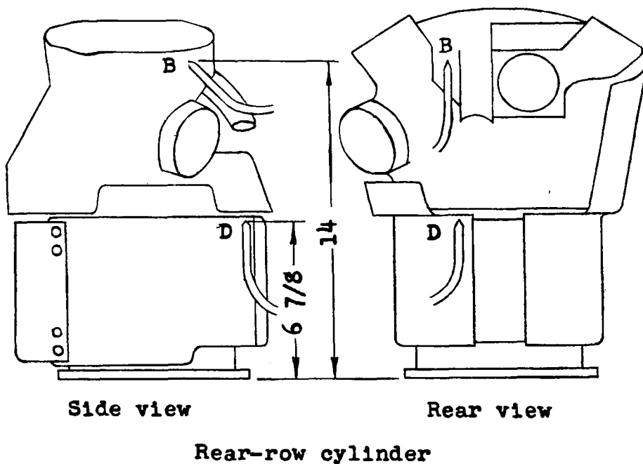
Figure 3. - Location of pressure tubes used in measuring cooling-air pressure drop across Wright R-2600-8 engine. All dimensions in inches.
