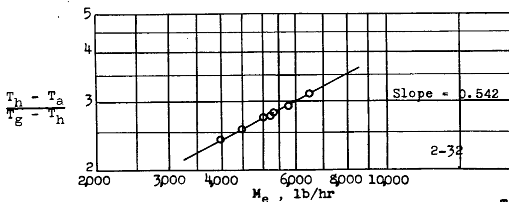
Figure 6. - Variation of cooling-temperature differential \frac{T_h - T_a}{T_g - T_h} with charge-air flow for cylinder heads. \sigma \Delta p , 13.7 inches water; fuel-air ratio, 0.08; Wright R-2600-8 engine.
