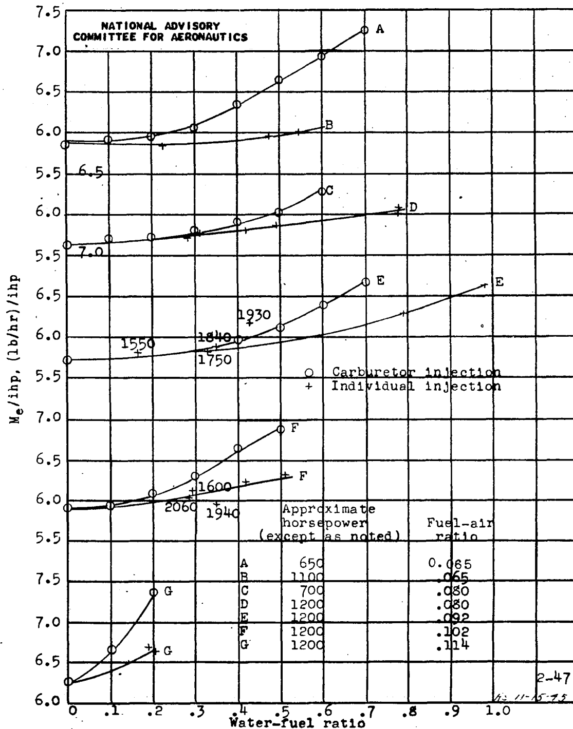
Figure 14. - Variation of indicated specific air consumption M_e/ihp with water-fuel ratio. Wright R-2600-8 engine.
