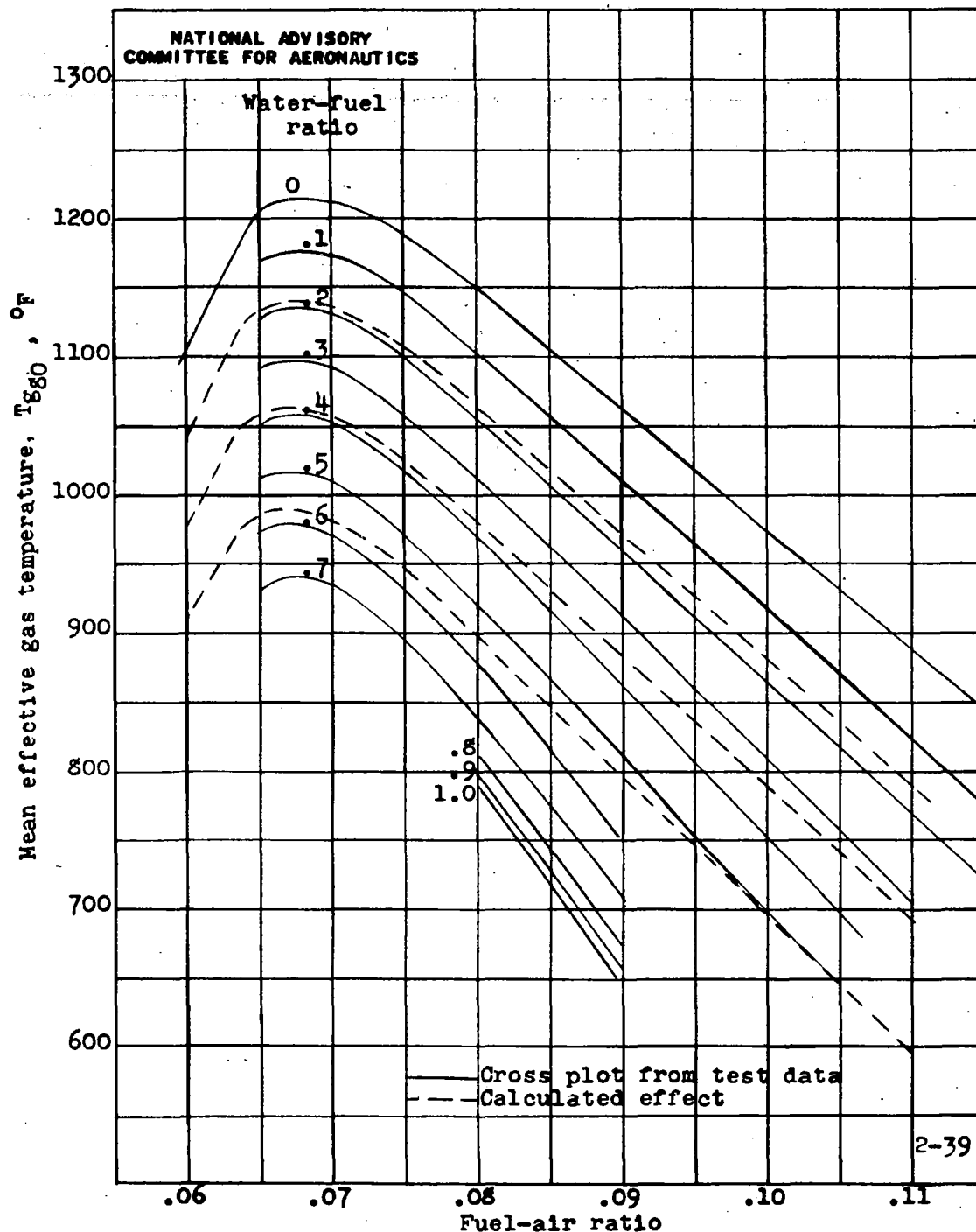
Figure 11. - Variation of mean effective gas temperature T_{Ego} with fuel-air ratio for water-fuel ratios indicated. Wright R-2600-8 engine.
