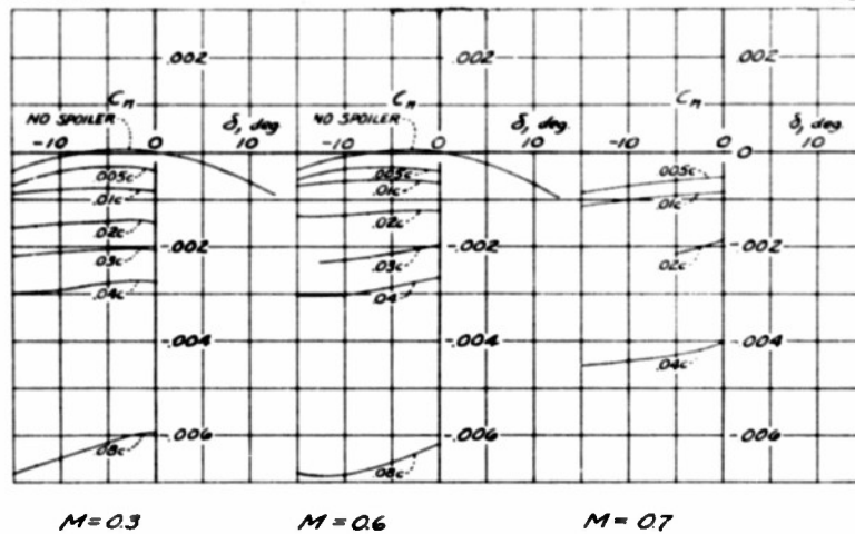
(b). \alpha = 2^\circ . FIGURE 18.- CONTINUED. SPOILER AND AILERON TEST.
