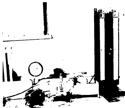
Fig. 9. Apparatus for Pressure Pick-Up Calibration
