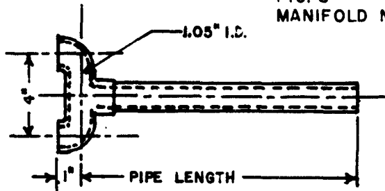
FIG. 4 MANIFOLD NO.2
