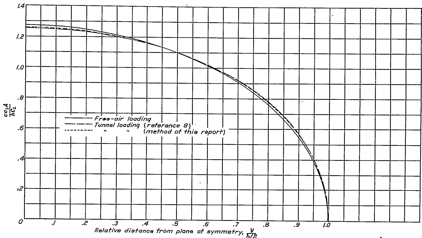
FIGURE 7.—Span load distributions for an elliptical wing in free air and in a closed circular tunnel. Wing span is 0.9 times the tunnel diameter.
