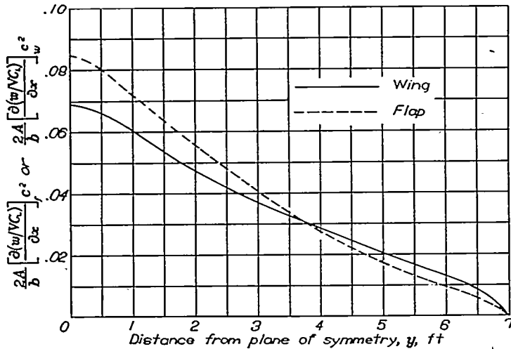
FIGURE 21.—Variation of \frac{2A}{b} \left[ \frac{\partial(w/VCL)}{\partial x} \right]_w c^2 and \frac{2A}{b} \left[ \frac{\partial(w/VCL)}{\partial x} \right]_f c^2 along the semispan of the model used for the illustrative example.
