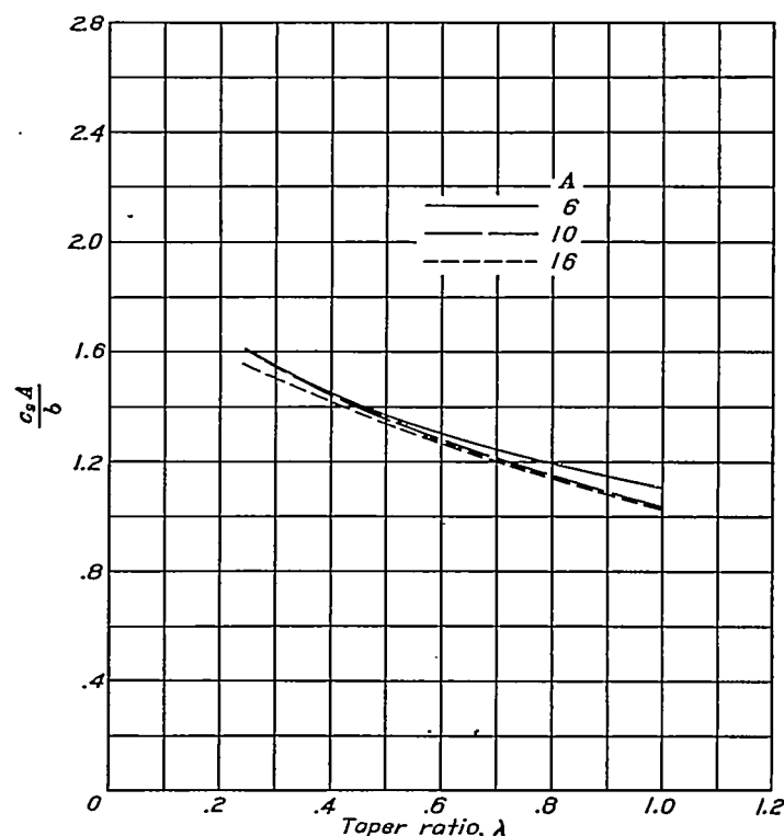
FIGURE 6.—Values of c_l A/b to be used in converting the load parameter cc_1/c_l \alpha of reference 5 to the load parameter cc_1 A/b \alpha .
