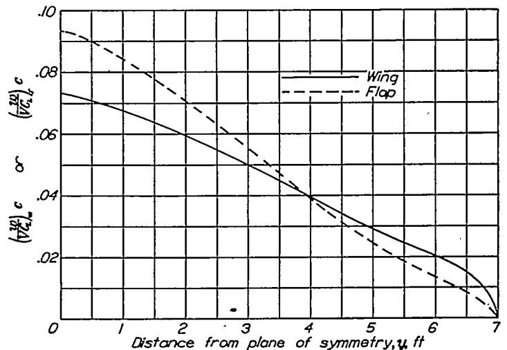
FIGURE 22.—Variation of \left( \frac{w}{VCL} \right) c along the semispan of the model used for the illustrative example.
