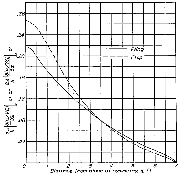
FIGURE 24.—Variation of \frac{2A}{b} \left[ \frac{\partial(w/Vc)}{\partial x} \right]_w and \frac{2A}{b} \left[ \frac{\partial(w/Vc)}{\partial x} \right]_f along the semispan of the model used for the illustrative example.
