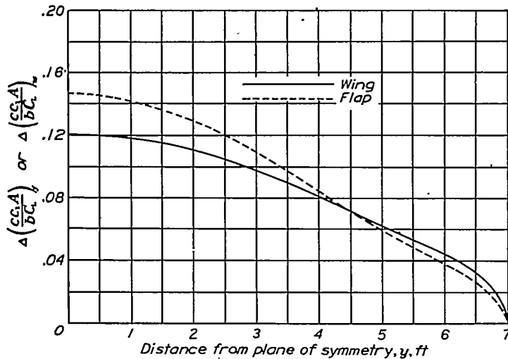
FIGURE 18.—Variation of the boundary-induced increment of load, due to the wing and due to the flap, along the semispan of the model used for the illustrative example.
