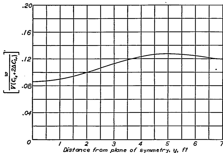
FIGURE 26.—Variation of the boundary-induced upwash angle, due to aileron deflection, along the semispan of the model used for the illustrative example.
