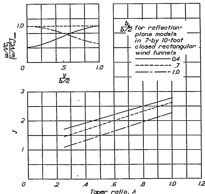
FIGURE 10.—Values of the aerodynamic-induction factor J used to calculate the rolling-moment correction for asymmetrically loaded reflection-plane models for three different variations of boundary-induced upwash angle. These upwash-angle variations correspond closely to those for aileron-span ratios of 0.4, 0.7, and 1.0 for models in 7- by 10-foot closed rectangular wind tunnels.
