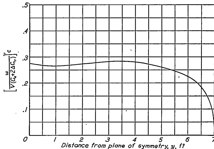
FIGURE 28.—Variation of \left[ \frac{w}{V(C_e + 2\Delta C_e)} \right]'^c along the semispan of the model used for the illustrative example.
