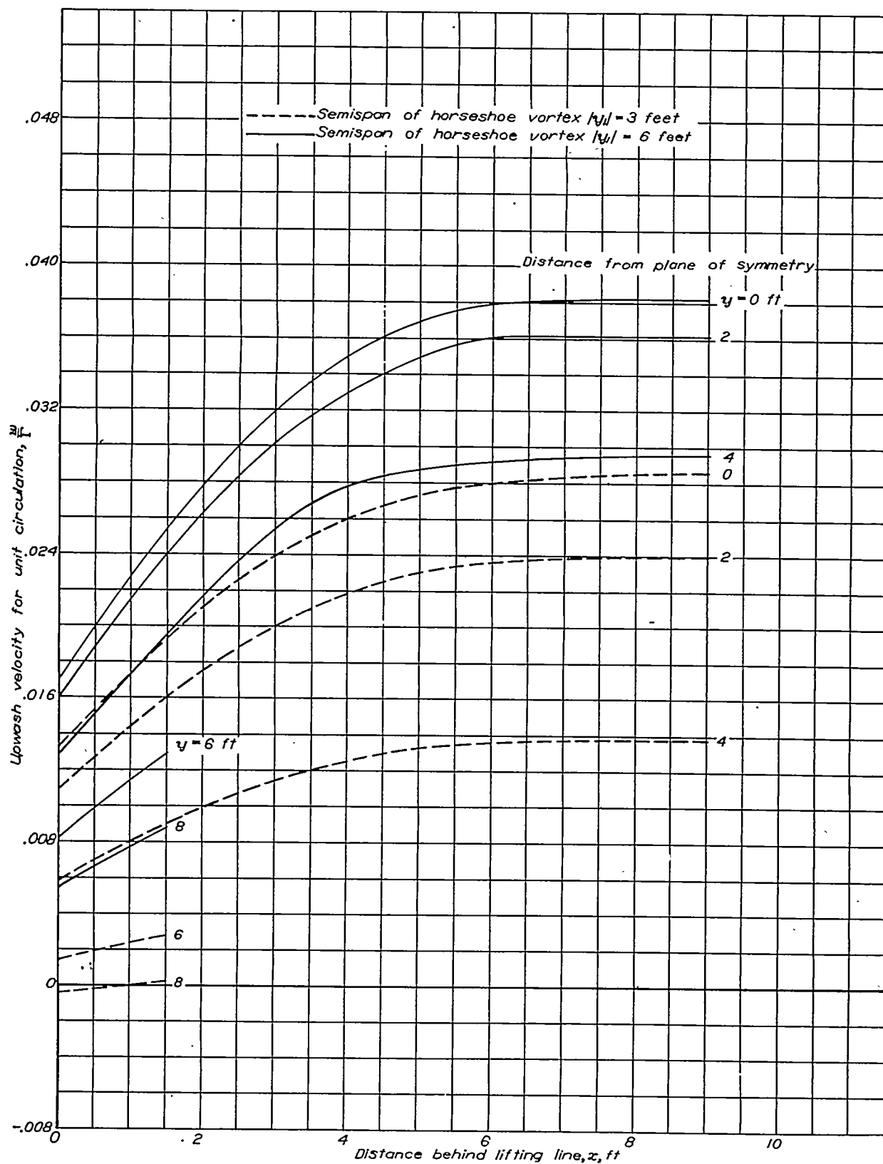
FIGURE 3.—Boundary-induced upwash velocity behind the lifting line for reflection-plane models mounted in 7- by 10-foot closed rectangular wind tunnels. d=0 .
