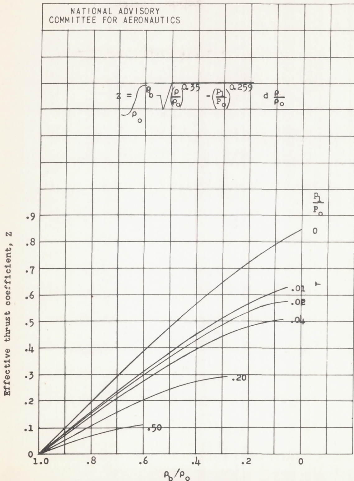
Figure 7.- Values of the effective thrust coefficient Z for a vessel periodically discharging from high pressure.
