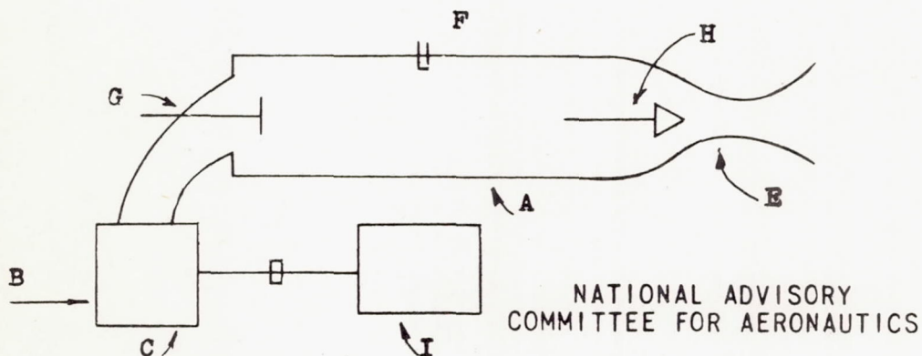
(c) A supercharged explosion jet-propulsion engine.
