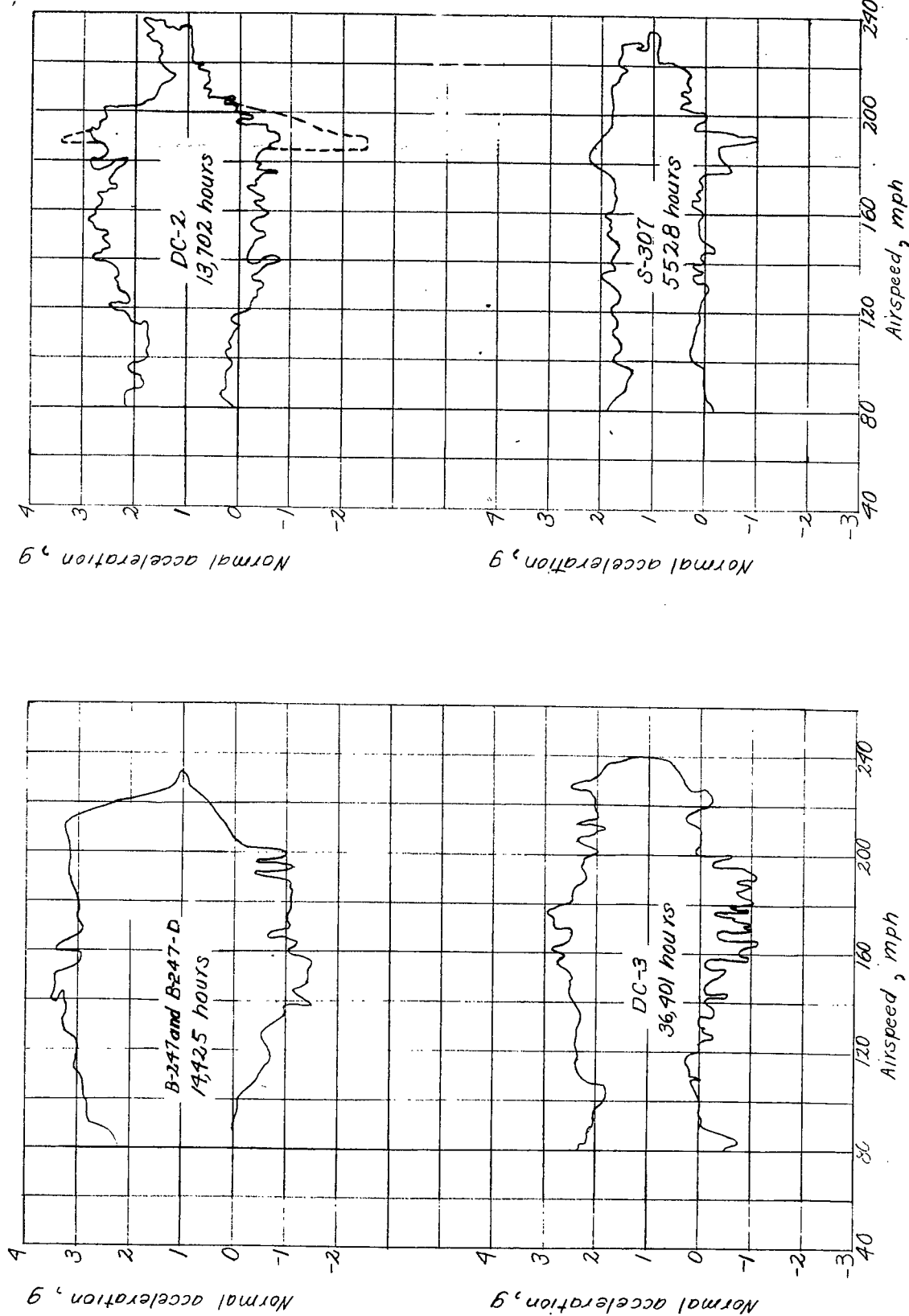
Figure 2.- Composite V-G envelopes for landplanes to April 1942.
