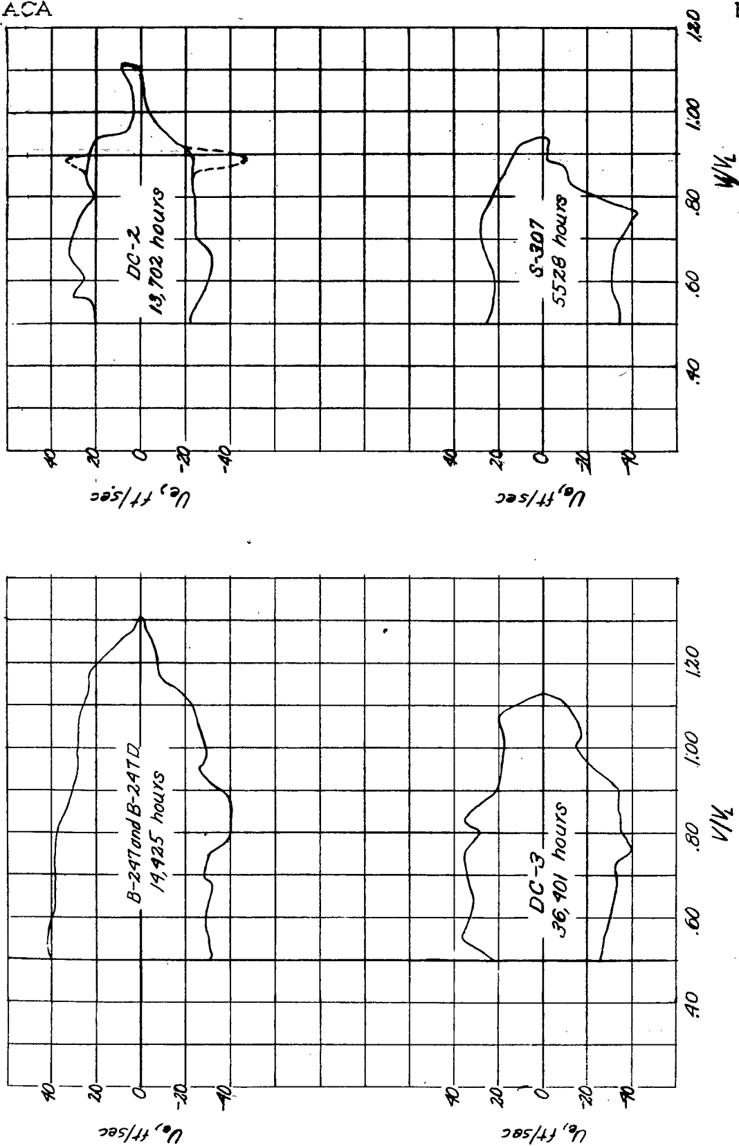
Figure 4.— Maximum effective gust velocities from V-G records for landplanes.
