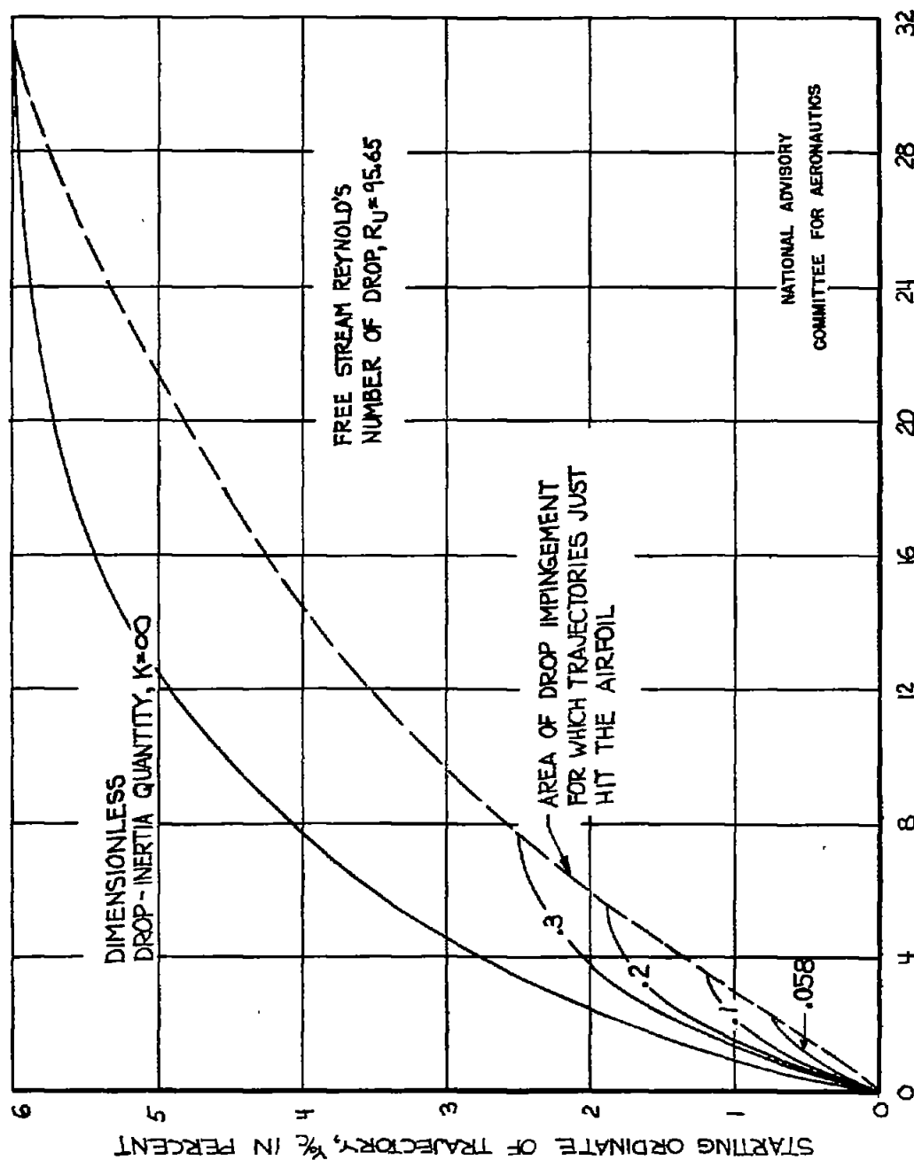
FIGURE 6.- AREA OF DROP INTERCEPTION CORRESPONDING TO DROPS OF DIFFERENT INERTIA FOR A SYMMETRICAL JOUKOWSKI AIRFOIL 12 PERCENT THICK.
