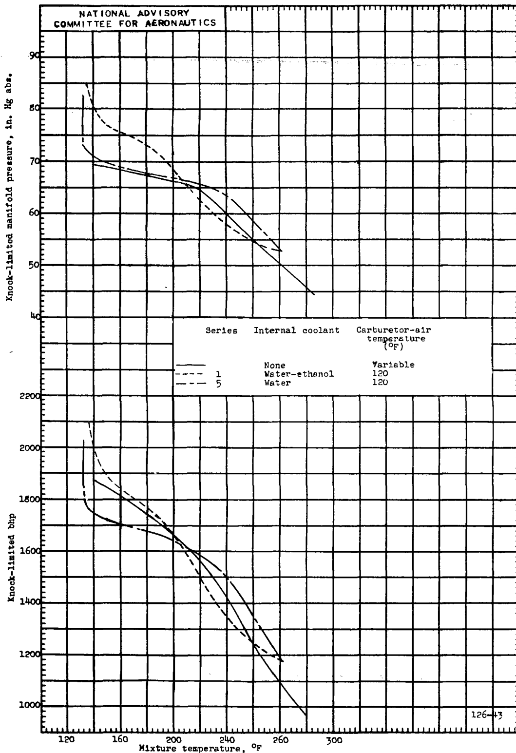
Figure 6. - Effect of mixture temperature on knock-limited performance with and without internal coolants. V-type 12-cylinder liquid-cooled engine; engine speed, 3000 rpm; compression ratio, 6.0; fuel, 28-R; fuel-nozzle internal-coolant injection. Cross plot at a fuel-air ratio of 0.08.
