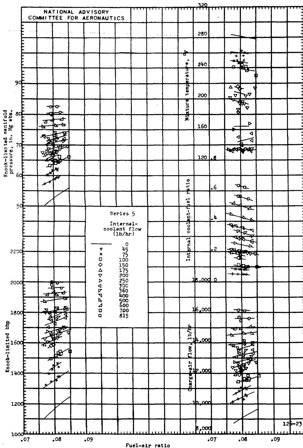
Figure 3. - Knock-limited data with water introduced with fuel through fuel nozzle. V-type 12-cylinder liquid-cooled engine; engine speed, 3000 rpm; compression ratio, 6.0; fuel, 28-R.
