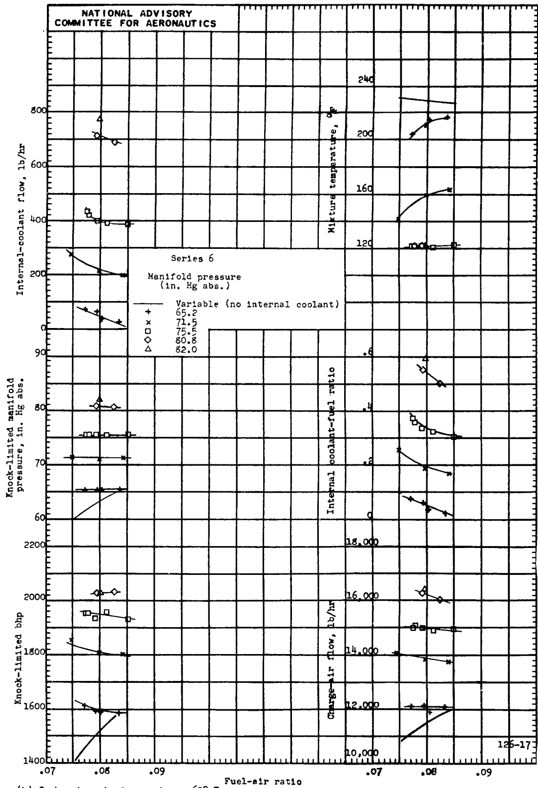
(b) Carburetor-air temperature, 60° F. Figure 3. - Concluded.
