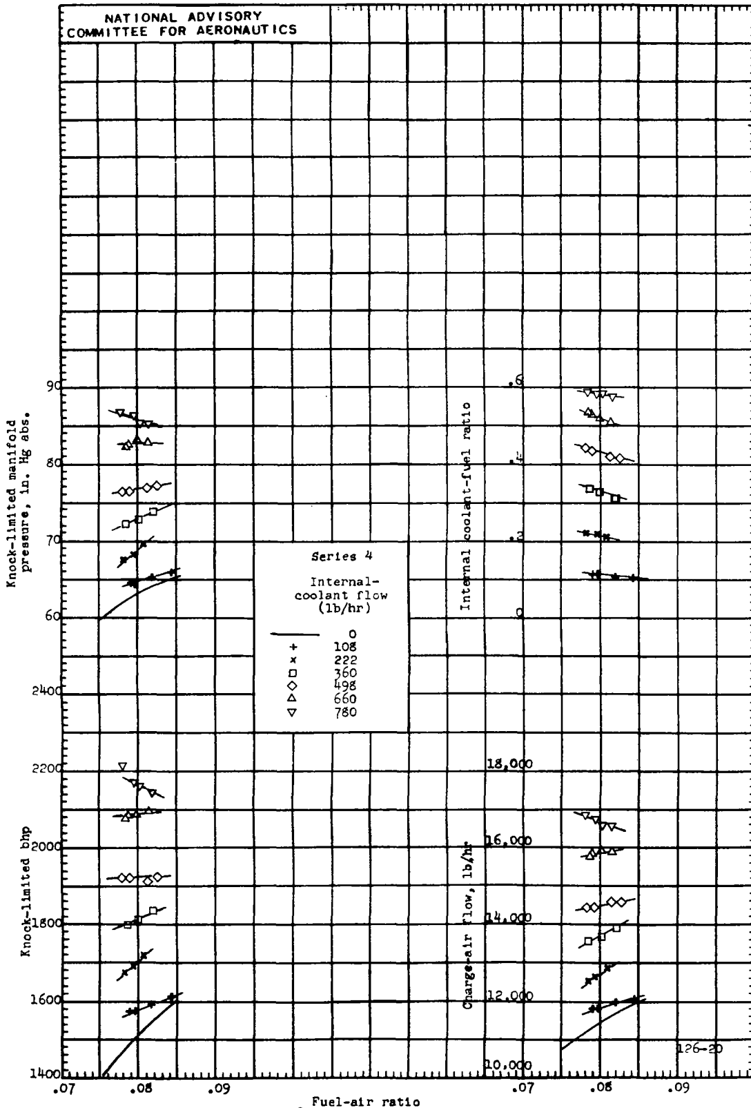
(b) Carburetor-air temperature, 60° F. Figure 2. - Concluded.
