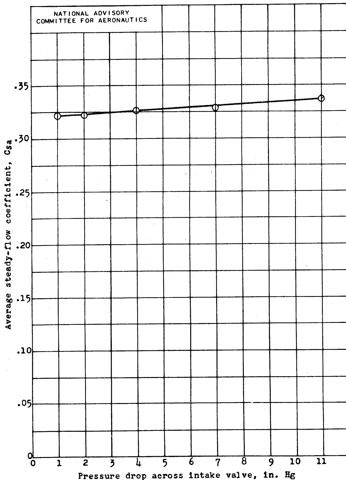
Figure 6. - Change in average steady-flow coefficient, C_{sa} with pressure drop. Upstream air pressure, 29.12 inches mercury absolute; valve diameter, 2.00 inches.
