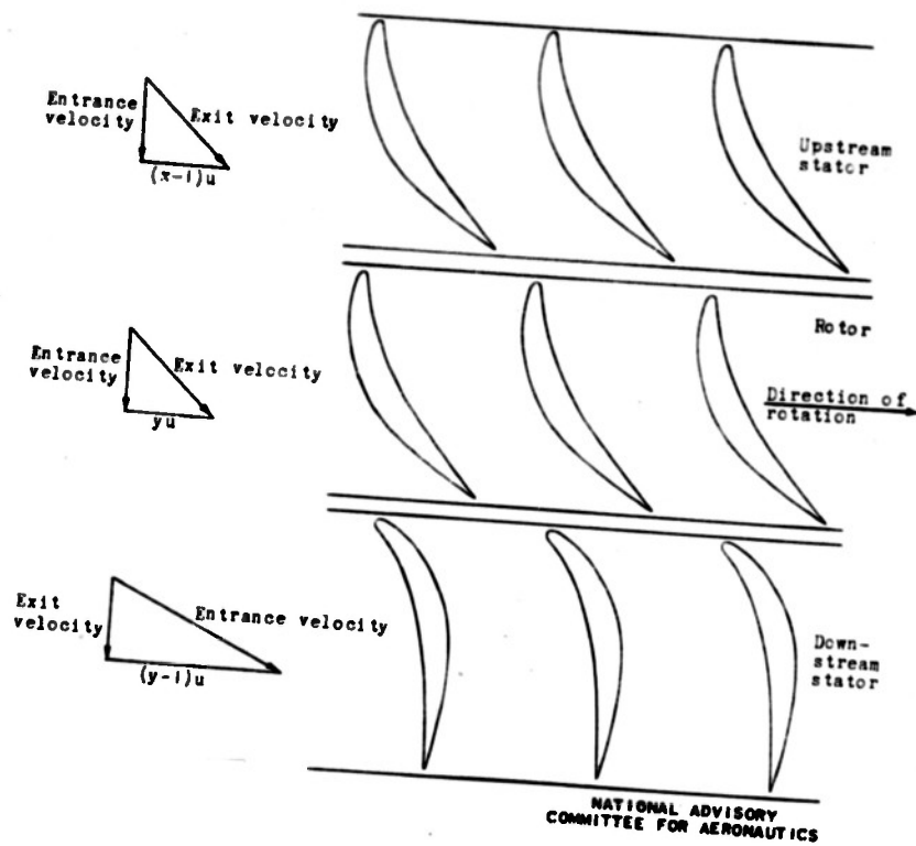
Figure 4. - Fan design for over-all pressure coefficient C_{pf} = 2 with rotor pressure coefficient C_{pr} = -1 . Velocity vectors shown are relative to corresponding blading. Design values: x = 0 ; y = -1 .
