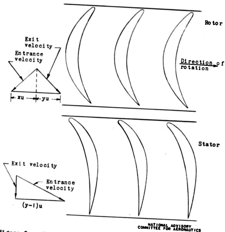
Figure 3. - Fan design for over-all pressure coefficient C_{pf} = 4 with rotor pressure coefficient C_{pr} = 0 . Velocity vectors shown are relative to the corresponding blading. Design values: x = 1 ; y = -1 .
