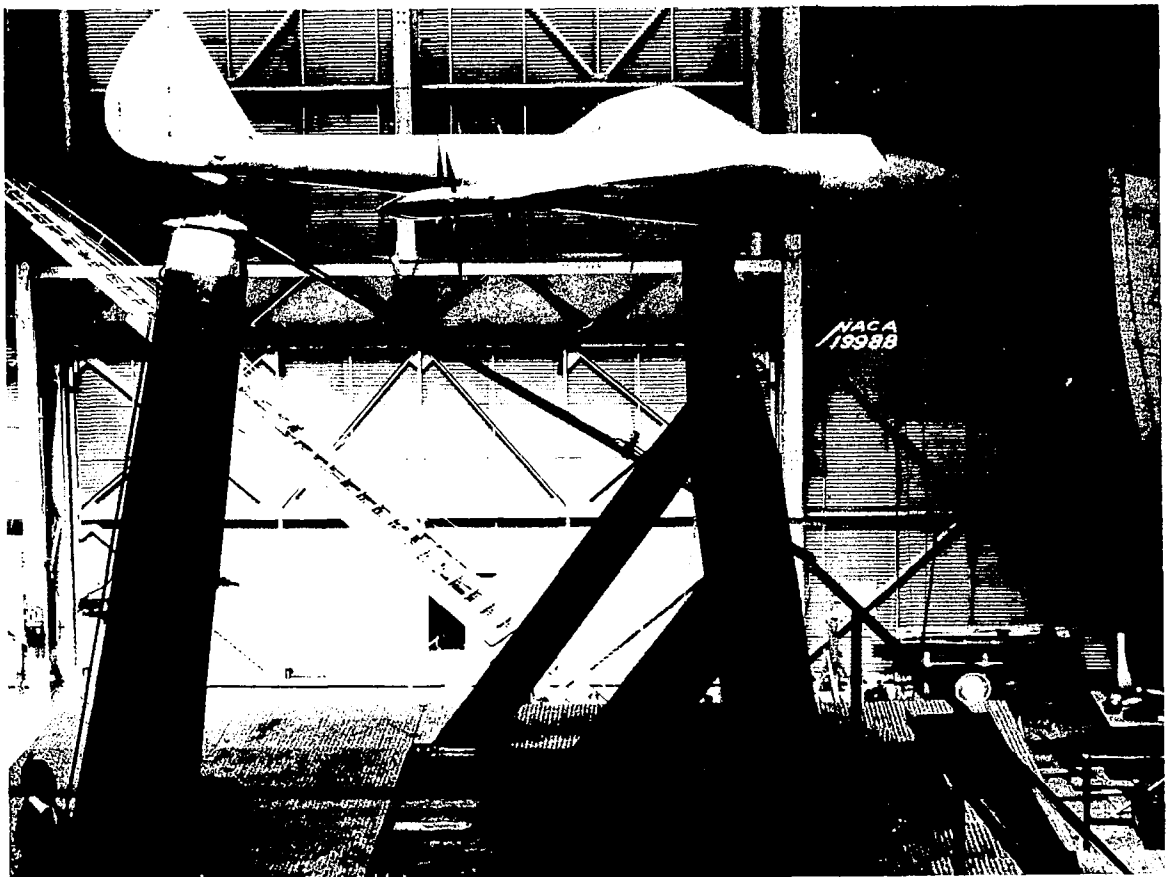
Figure 2.- The four-engine airplane model installed in the full-scale tunnel with conventional propellers and without flap twist.
