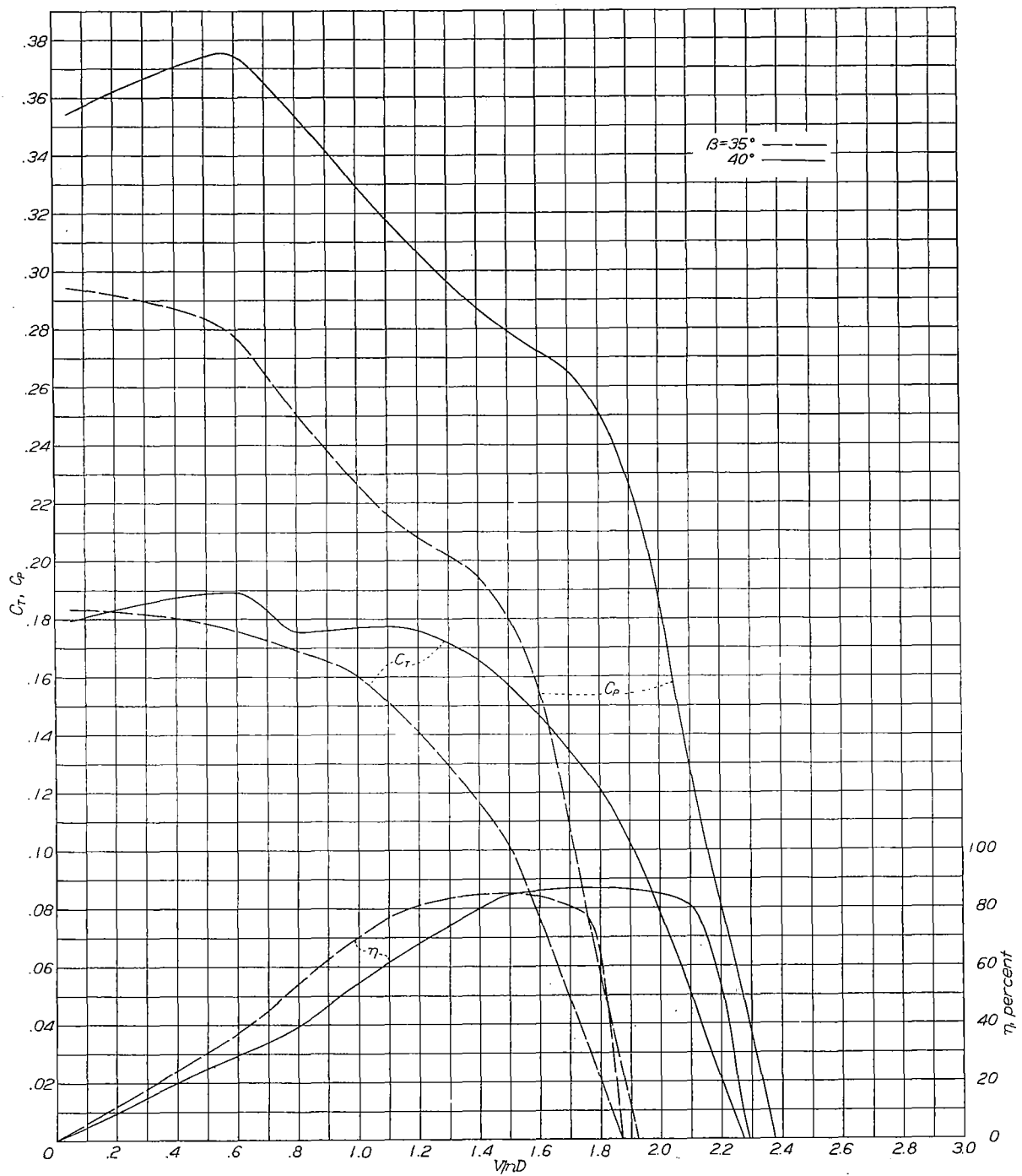
Figure 6.- Propulsive characteristics for the special pusher-design propeller with 0.83 of the basic flap twist.
