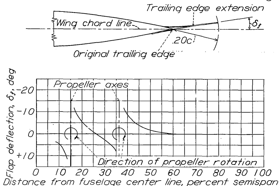
Figure 4.- The trailing-edge deflections for the basic flap twist.
