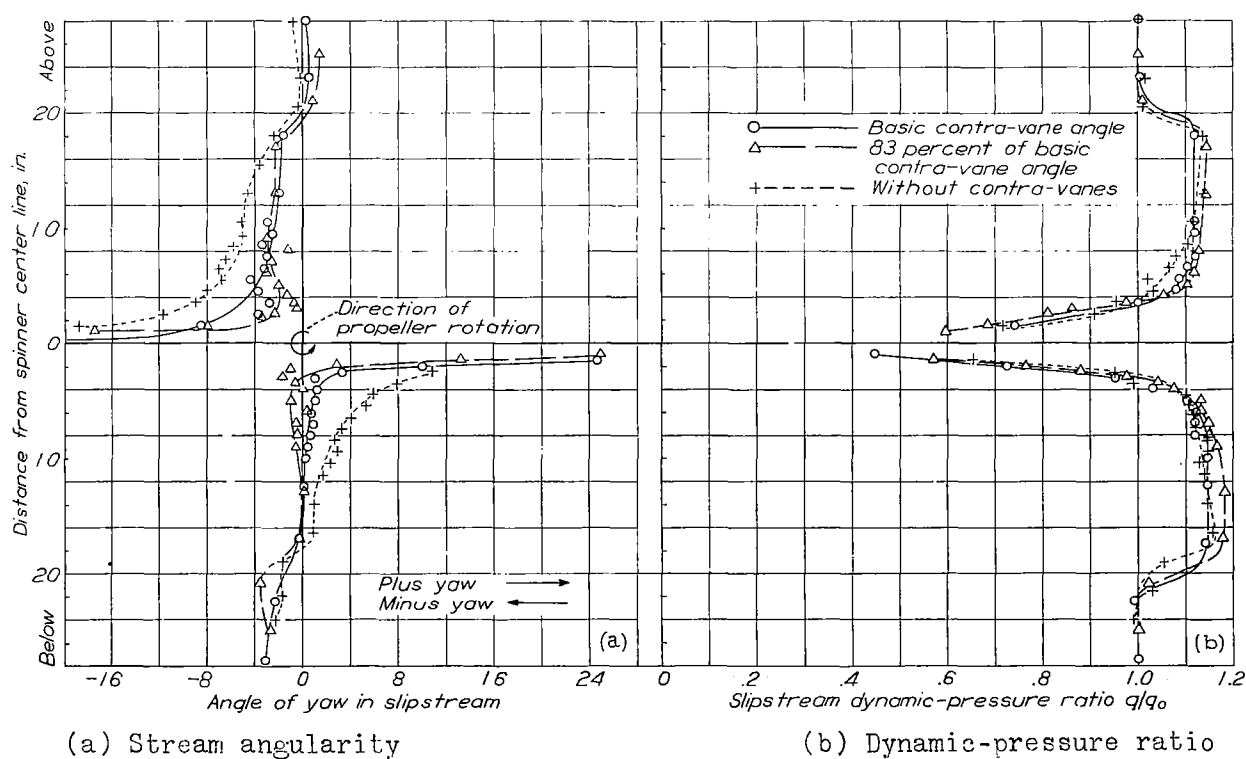
Figure 9.- Surveys of the air flow in the slipstream.
