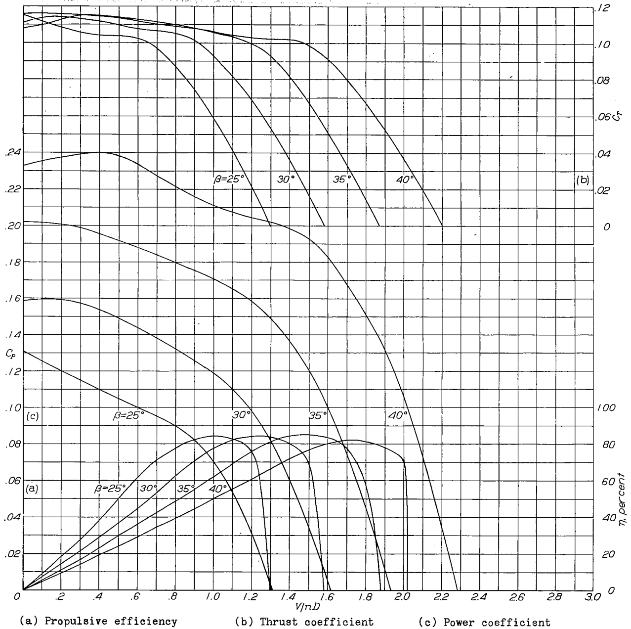
Figure 8.- Propulsive characteristics for the conventional propeller.
