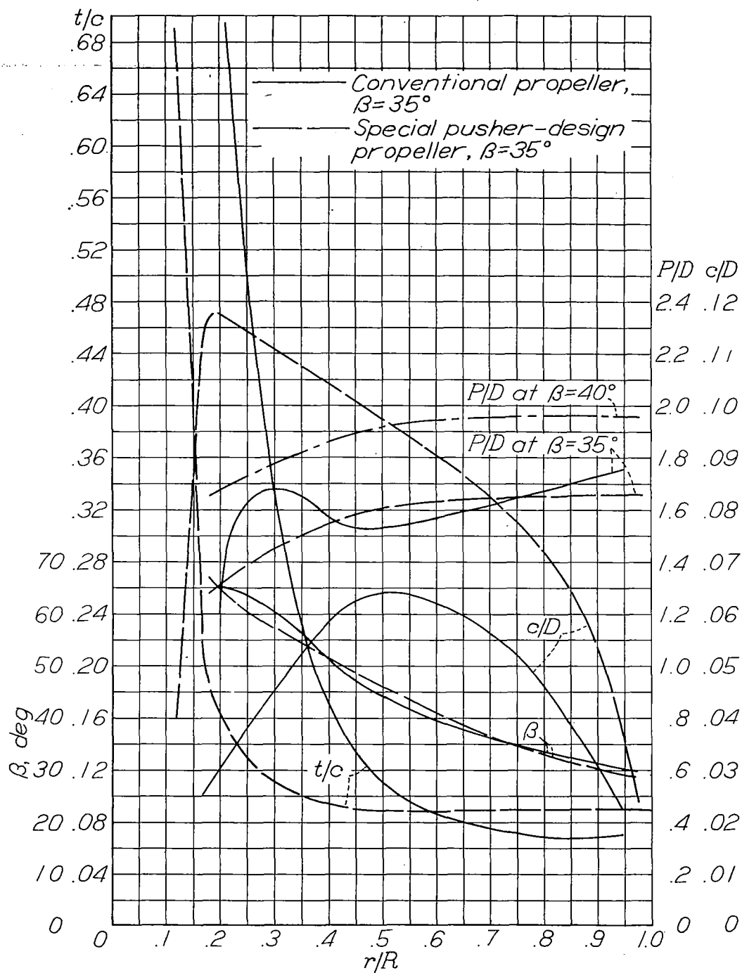
Figure 3.- The blade characteristics for the test propellers.
