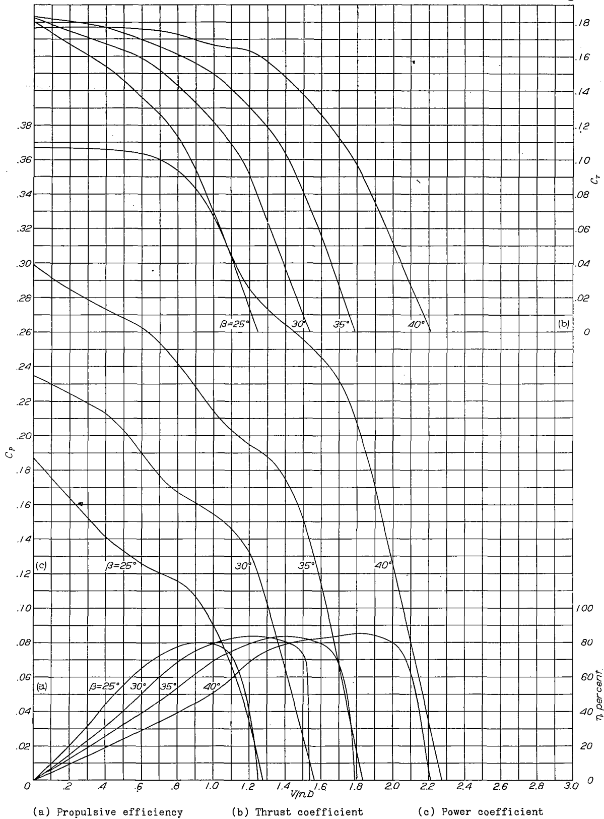
Figure 7.- Propulsive characteristics for the special pusher-design propeller without the twisted flap.
