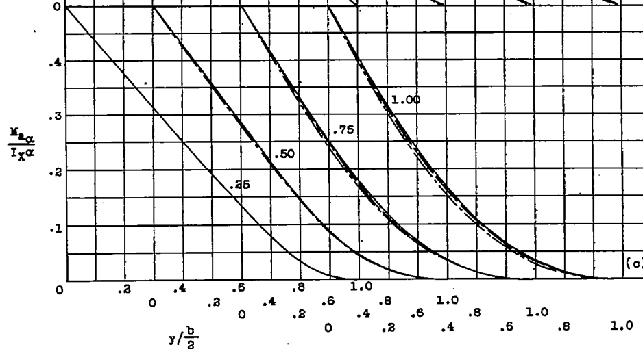
(a) Load \lambda = 2:1
