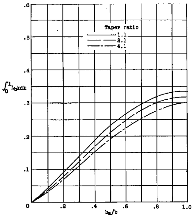
Figure 7.- Angular acceleration factor for ailerons.
