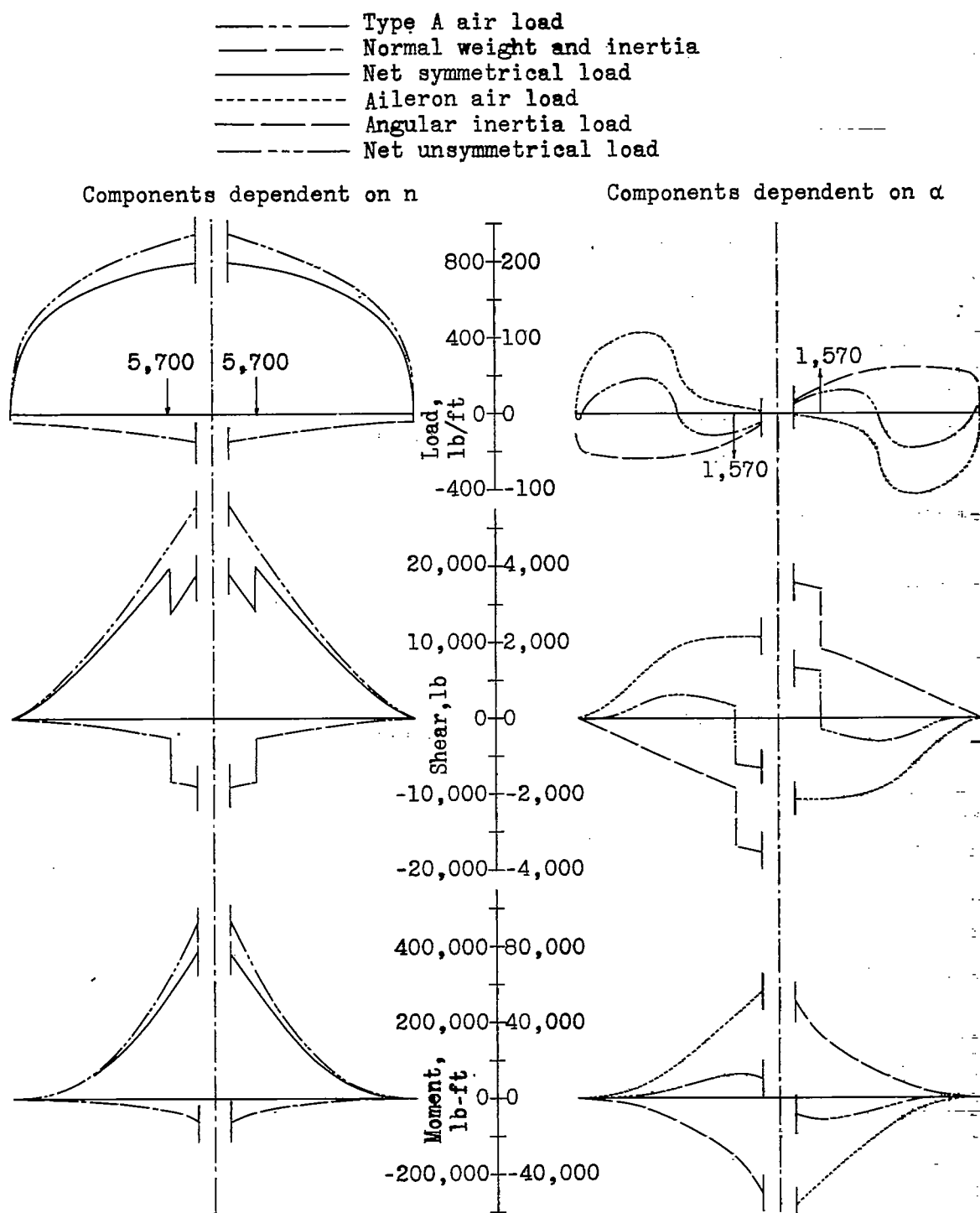
Figure 14.- Component load, shear, and moment distributions for airplane B.
