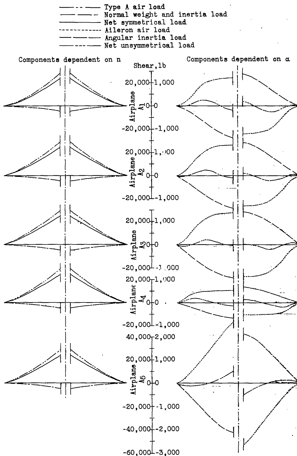
Figure 12.- Shear components for airplanes A 1 to A 5 in flight.
