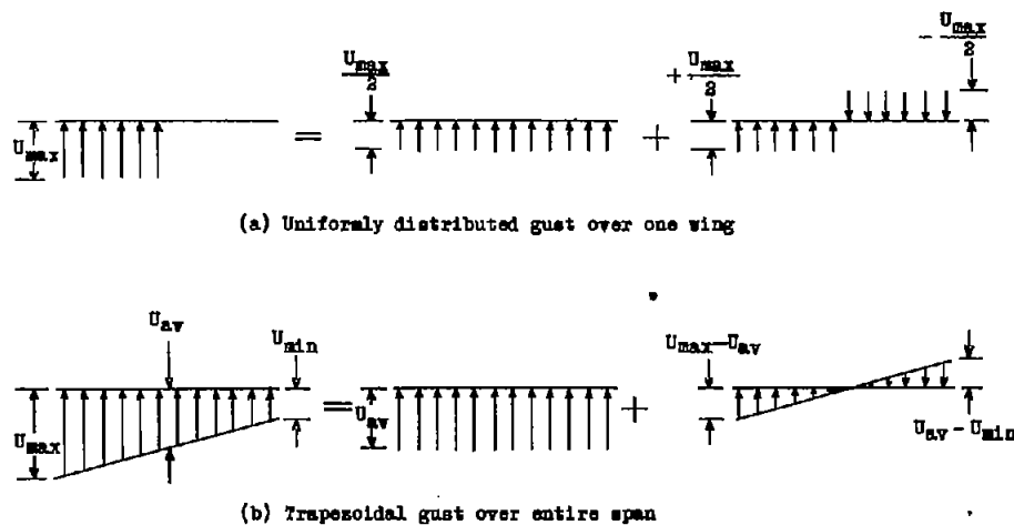
Figure 8.- Elementary gust types.
