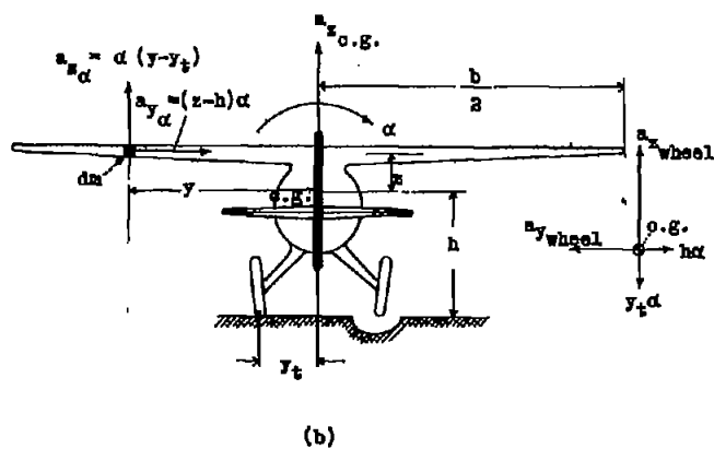
Figure 2.- Accelerations on airplane.
