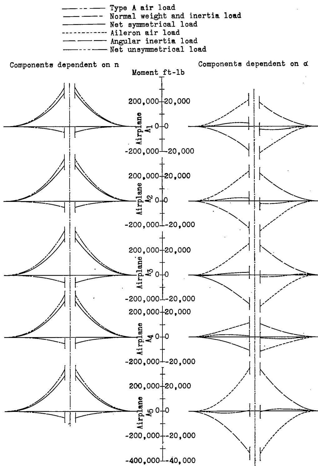
Figure 13.- Moment components for airplanes A 1 to A 5 in flight.
