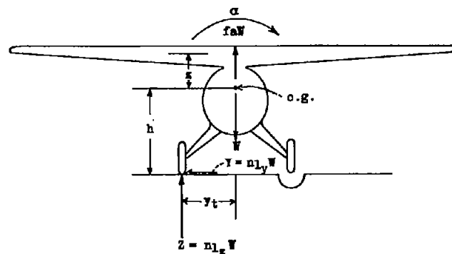
Figure 10.- Forces acting in a one-wheel landing.
