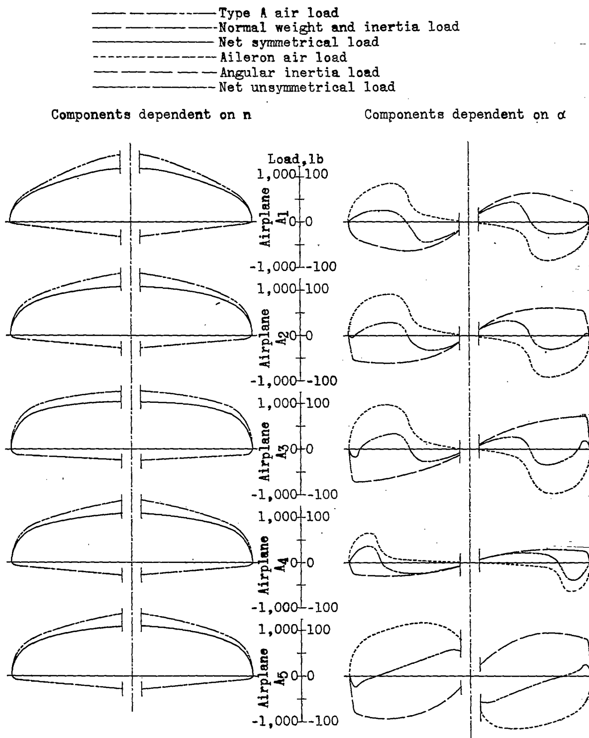
Figure 11.- Load components for airplanes A1 to A5 in flight.
