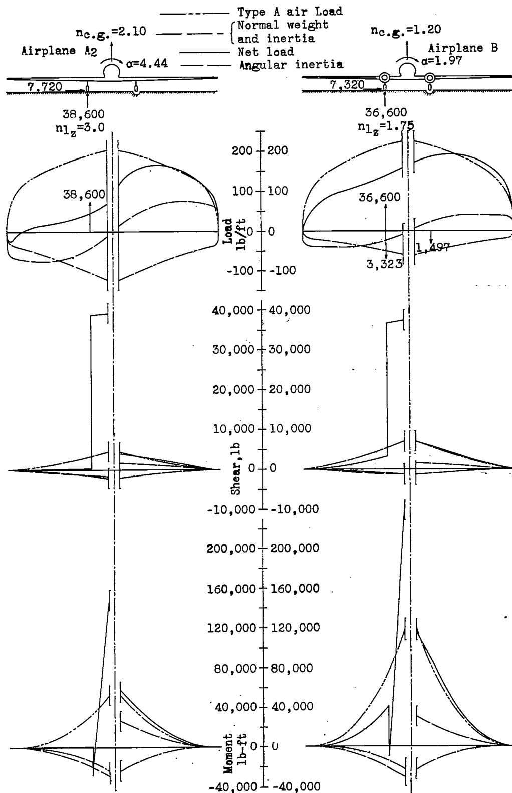
Figure 15.- Component load, shears, and moments in one-wheel landing.
