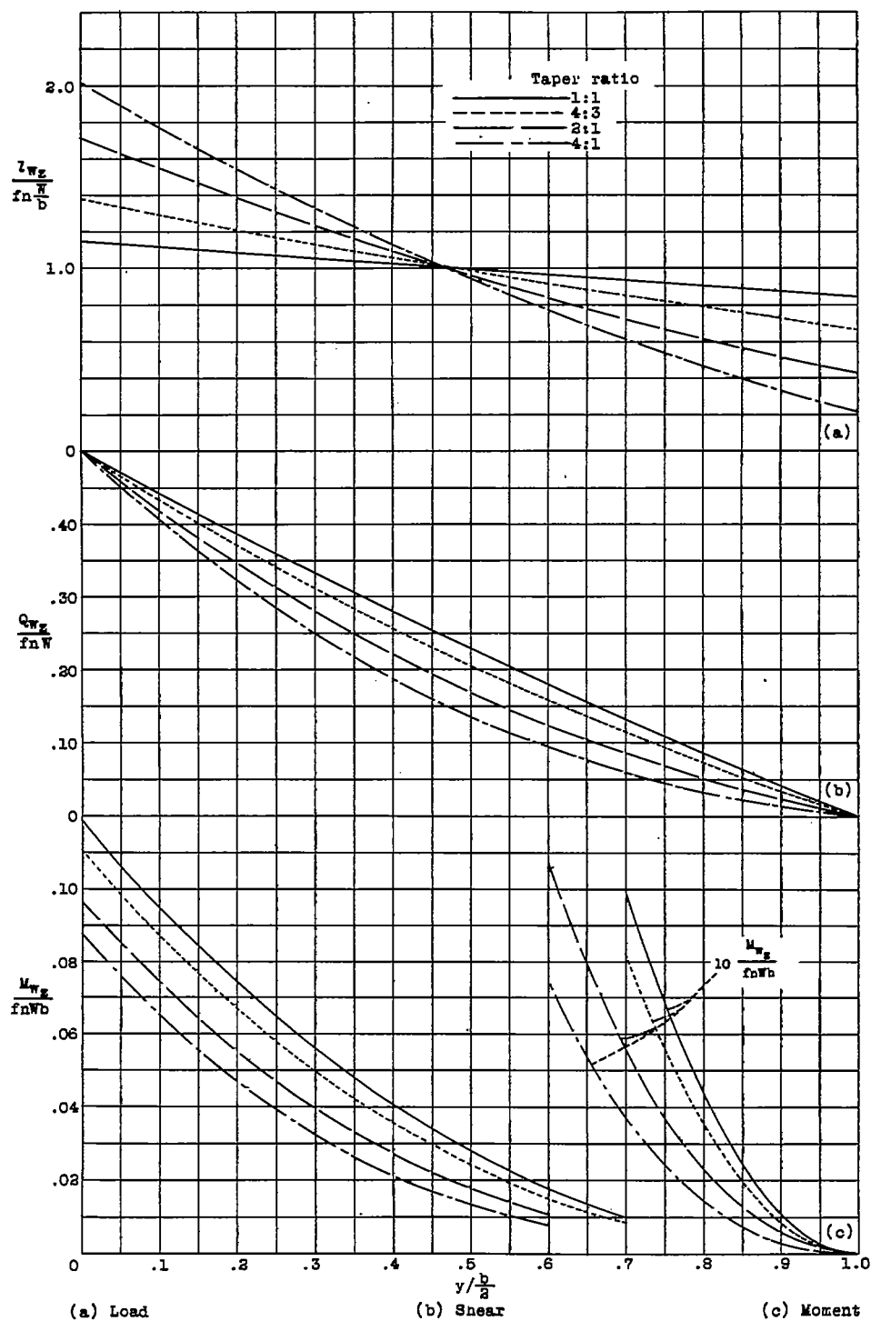
Figure 5.- Load, shear, and moment distribution due to wing weight and normal inertia load.
