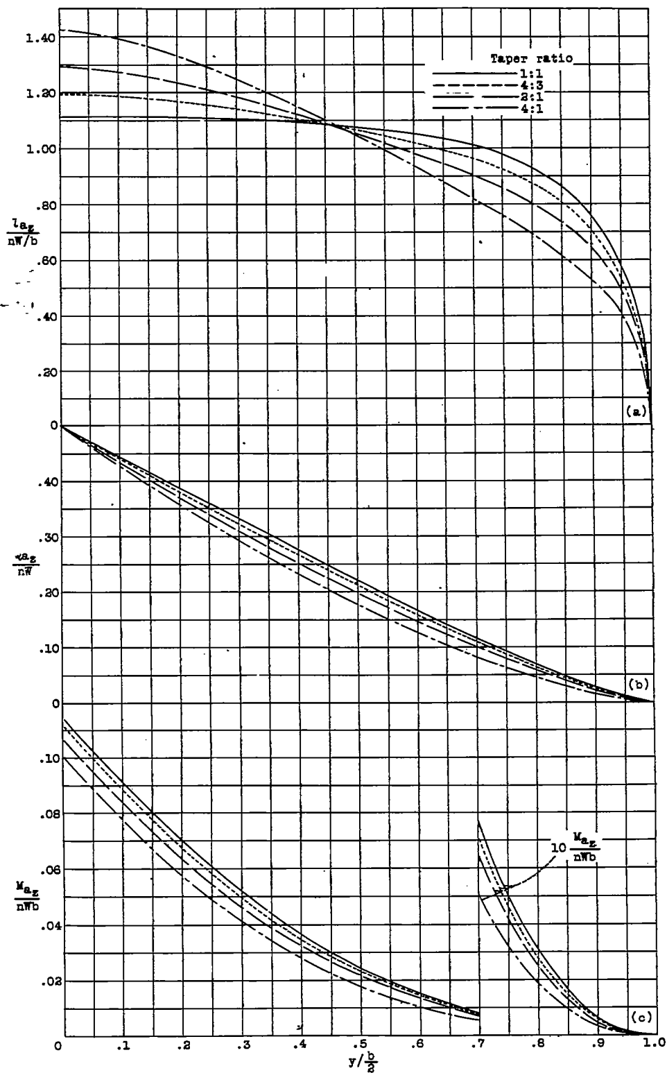
(a) Load (b) Shear (c) Moment
