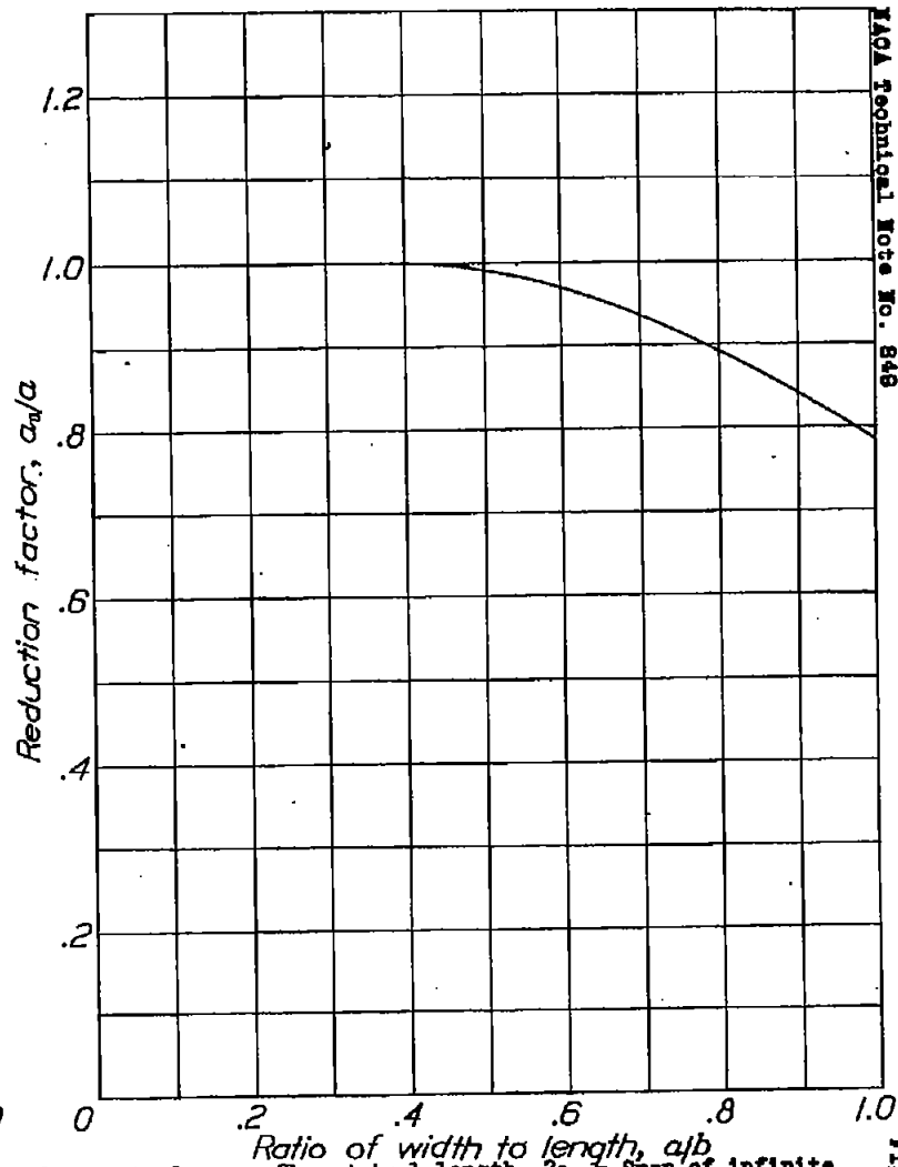
Figure 35.- Reduction factor for maximum stress at center of longest side of clamped rectangular plates.
