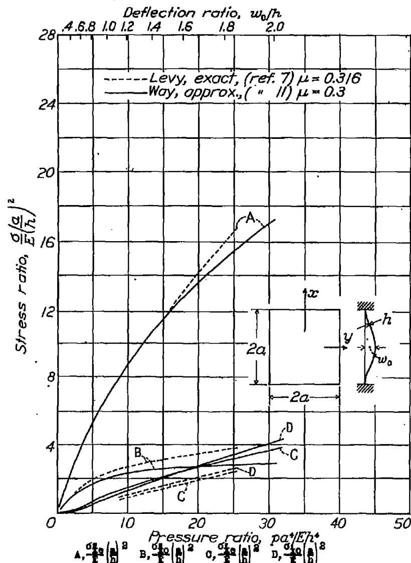
Figure 26.- Stress in a square plate with clamped edges.
