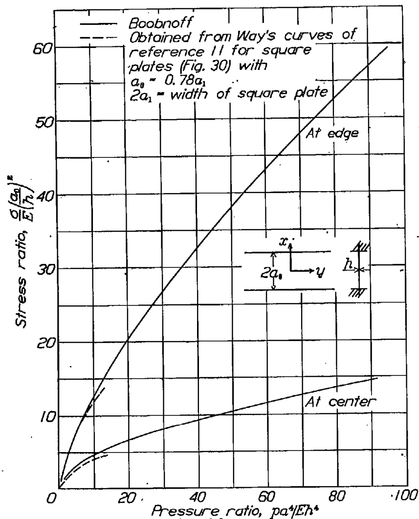
p = pressure E = Young's modulus Figure 38.— Extreme-fiber stress in infinite plate strip ( a/b = 0 ), clamped edges, according to reference 12. Poisson's ratio, 0.3.
