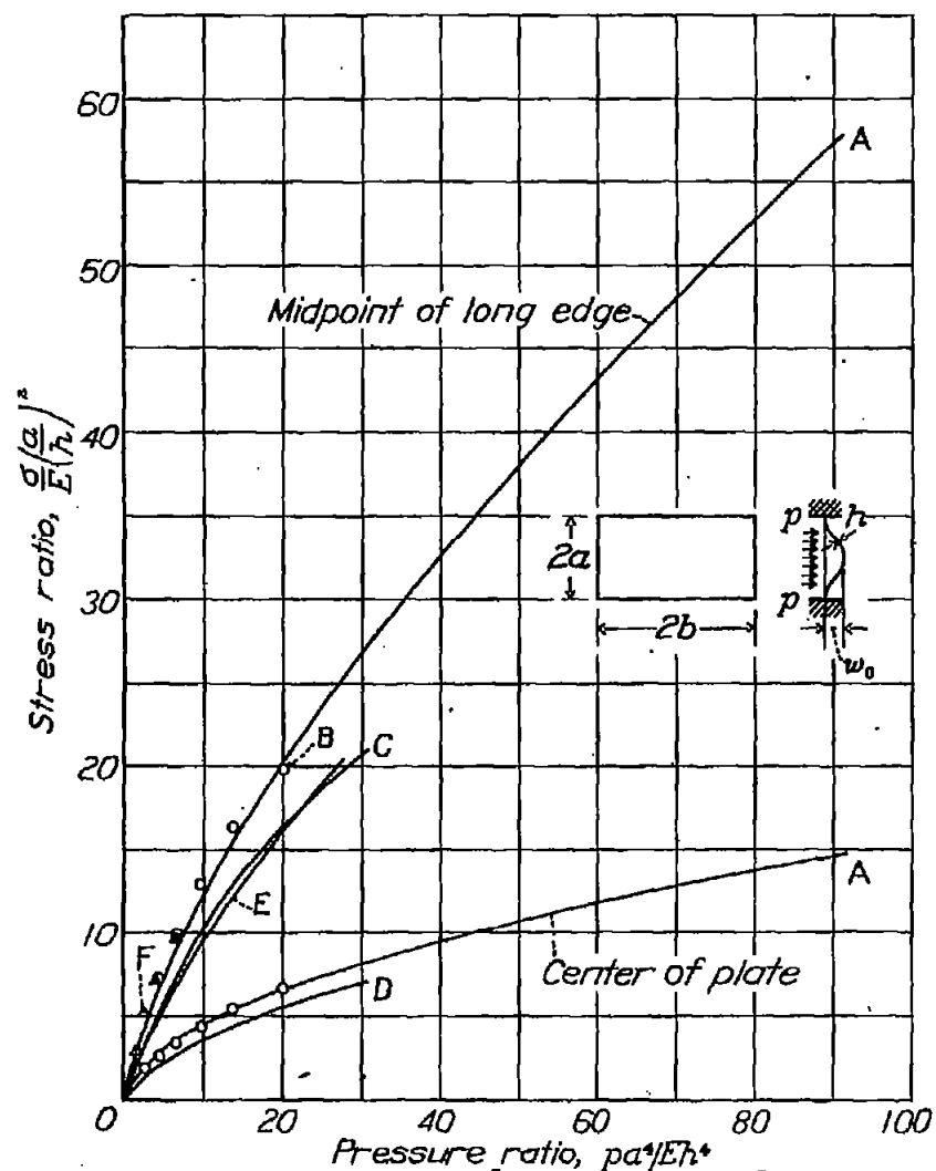
Figure 30.- Extreme-fiber stresses for rectangular plates with clamped edges. Data from references 7, 11 and 13.
