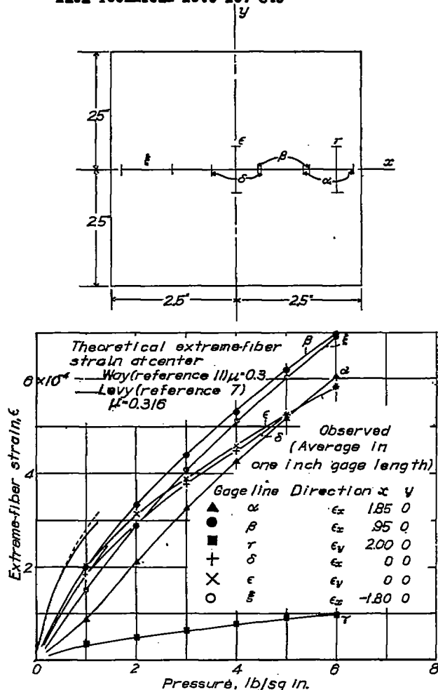
Figure 16.- Extreme-fiber strains on square 178-T aluminum-alloy plate 10a with clamped edges.
