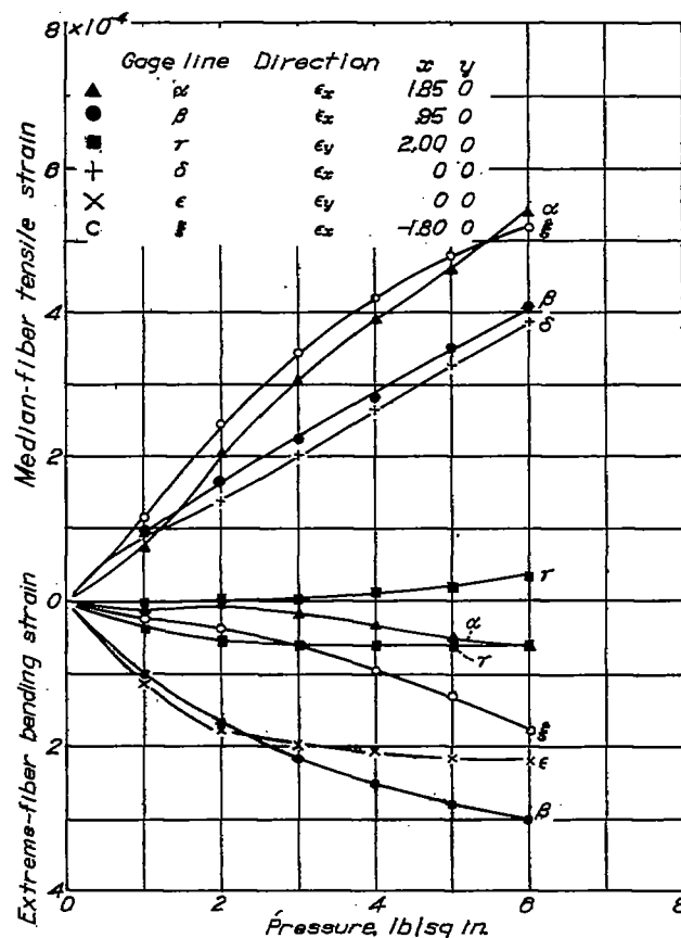
Figure 17.- Medium-fiber tensile strain and extreme-fiber bending strain (average over 1-in. gage length) for square 178-T aluminum-alloy plate 10a with clamped edges.
