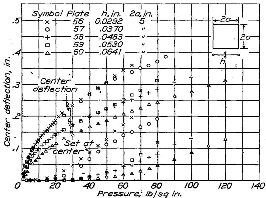
Figure 15.— Deflection and set at center of square 17S-T aluminum-alloy plates with freely supported edges.
