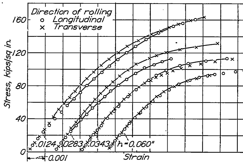
Figure 2.— Tensile stress strain curves for 18:8 stainless steel.
