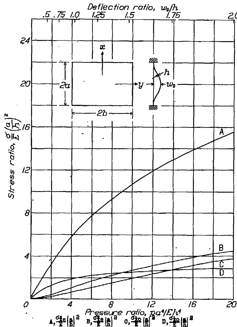
Figure 27.- Stress in a rectangular plate ( a/b = 2/3 ) with clamped edges according to reference 11. Poisson's ratio, 0.3.
