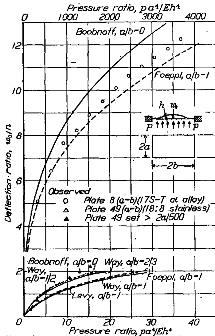
Figure 24.- Center deflection against pressure for rectangular plates with clamped edges. Poisson's ratio, 0.3.
