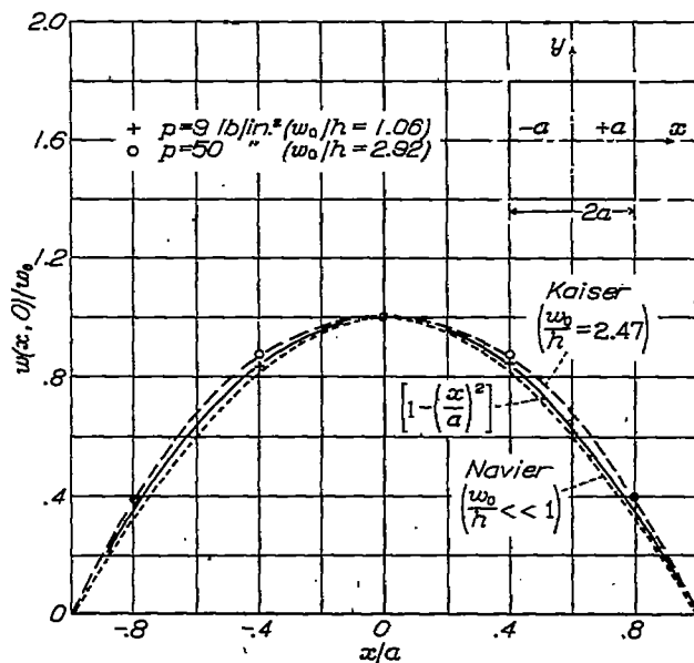
Figure 9. Change in shape of deflection curve along center line as the pressure is increased for freely supported square plate 60. h, 0.641 inch, a, 2.5 inches.
