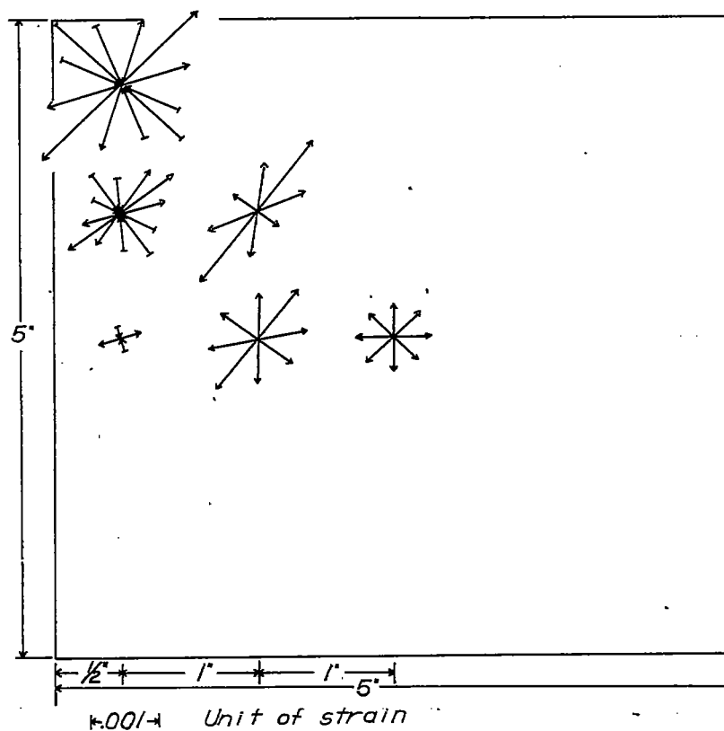
Figure 22.- Bending strains from contours on top of 5-by 5-inch 17S-T aluminum-alloy plate 54 with freely supported edges. Strains correspond to change in pressure between 1 and 15 pounds per square inch.
