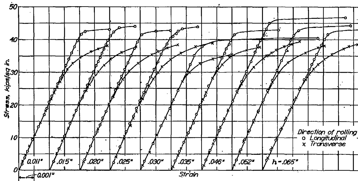
Figure 1. Tensile stress strain curves for 17S T aluminum alloy.
