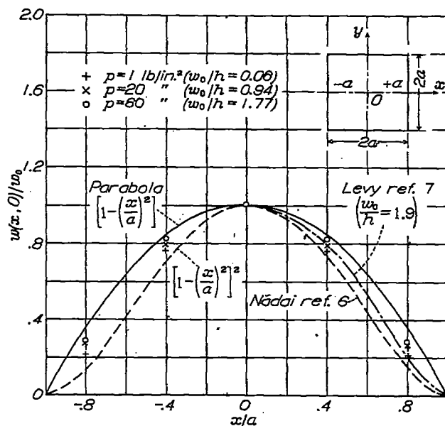
Figure 8. Change in shape of deflection curve along center line as the pressure is increased for clamped edge square plate 34. h, 0.0653 inch, a, 2.5 inches.
