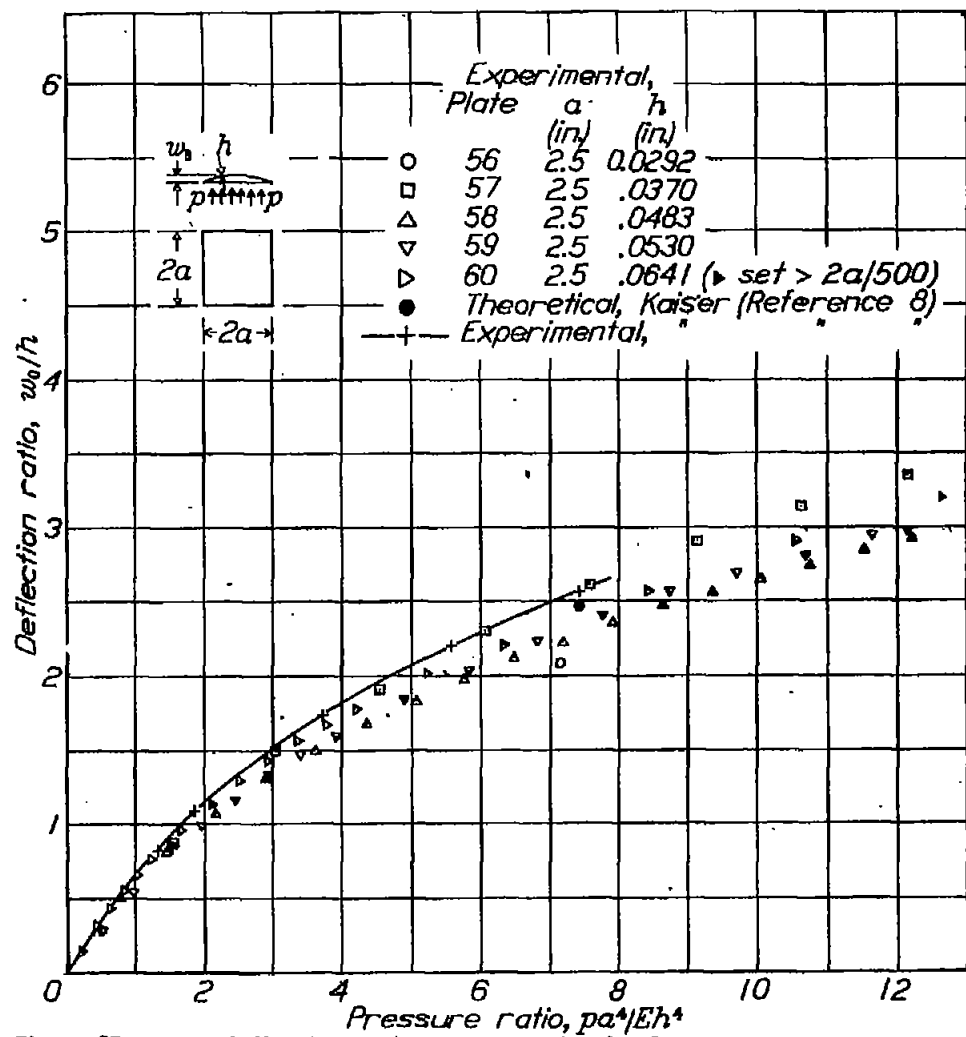
Figure 25.- Center deflection against pressure for freely supported square plates. Poisson's ratio, 0.3.
