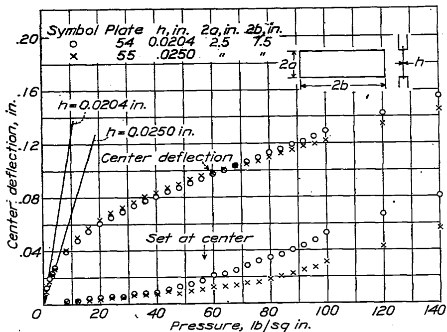
Figure 14.— Deflection and set at center of rectangular 24S-RT aluminum alloy plates with clamped edges.
