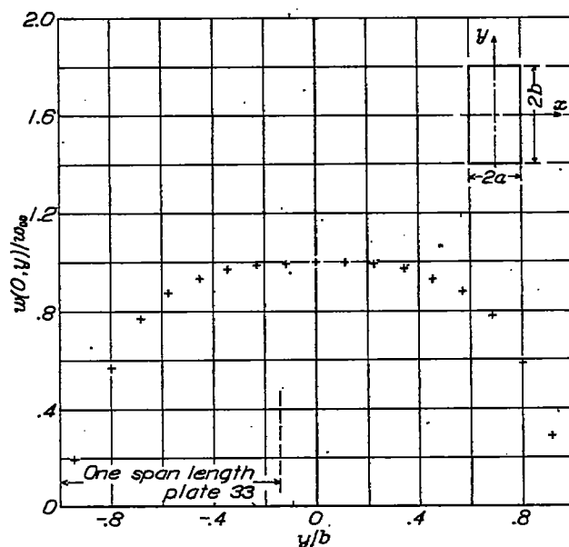
Figure 10.— Deflection curve along longitudinal center line of rectangular plates 33(17S-T) with clamped edges.
