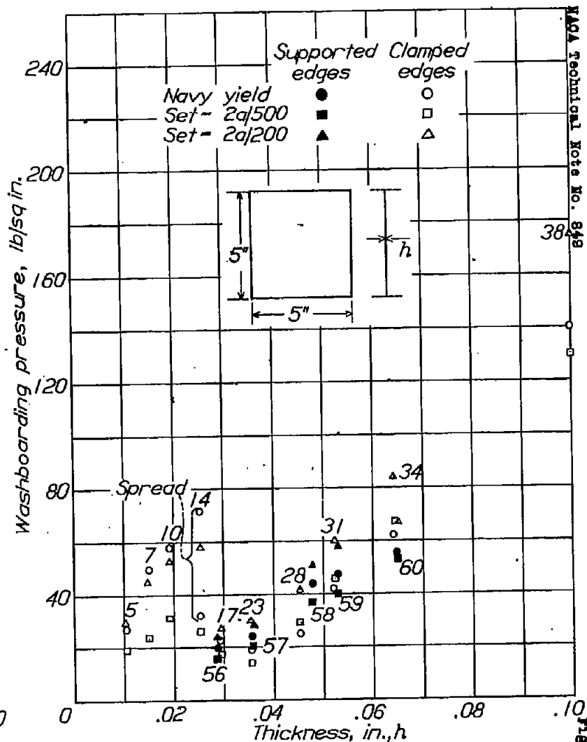
Figure 39.— Comparison of washboarding pressures for 5-by 5-inch 178-T aluminum-alloy plates.
