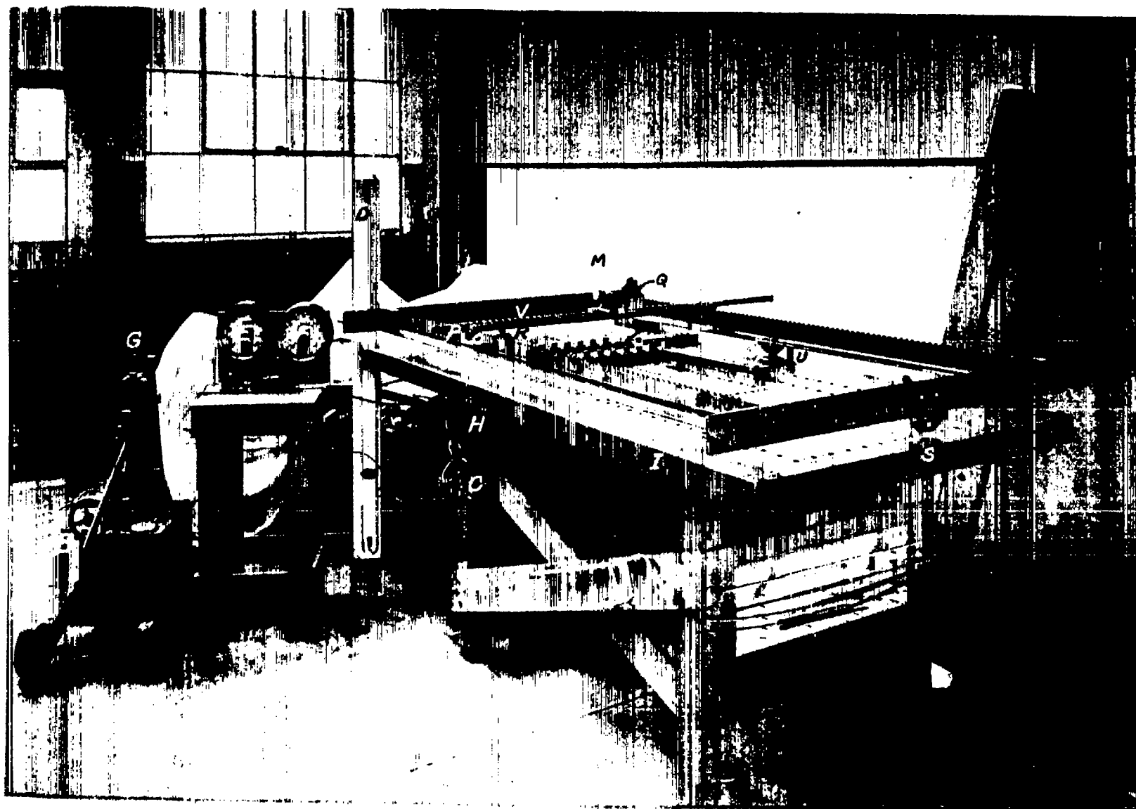
Figure 4.- Apparatus for normal-pressure tests of rectangular plates.
