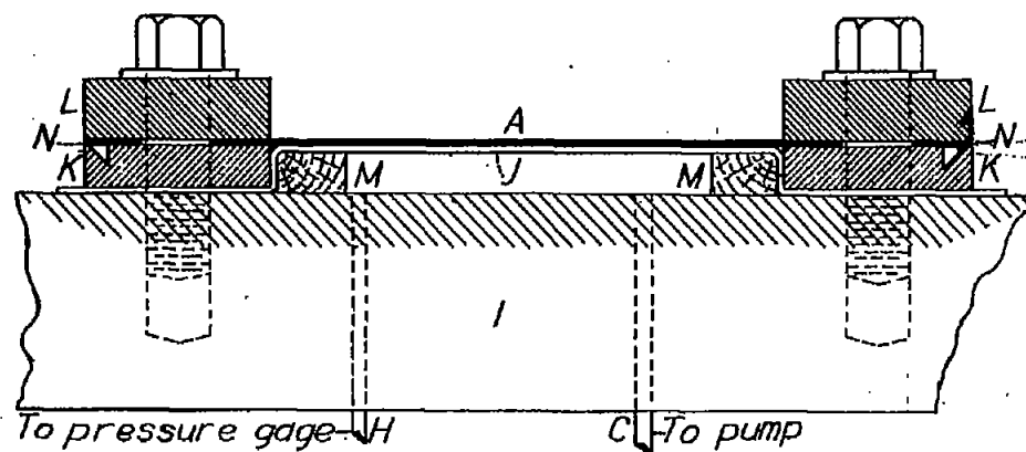
Figure 6. Section through plate mounted for normal pressure test with clamped edges.
