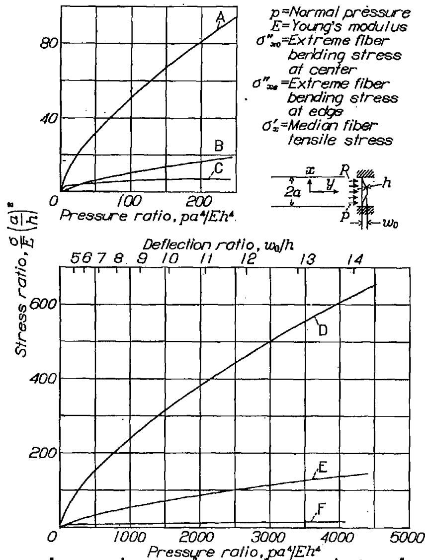
A, \frac{\sigma''_{x0}}{E} \left(\frac{a}{h}\right)^2 B, \frac{\sigma'_x}{E} \left(\frac{a}{h}\right)^2 C, \frac{\sigma''_{x\infty}}{E} \left(\frac{a}{h}\right)^2 D, \frac{\sigma''_{x0}}{E} \left(\frac{a}{h}\right)^2 E, \frac{\sigma'_x}{E} \left(\frac{a}{h}\right)^2 F, \frac{\sigma''_{x\infty}}{E} \left(\frac{a}{h}\right)^2 Figure 28.- Stress in infinite plate strip ( a/b = 0 ) with clamped edges according to reference 11. Poisson's ratio, 0.3.
