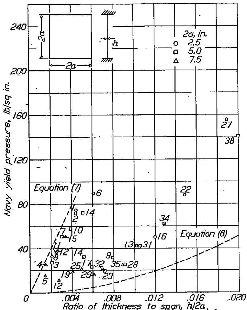
Figure 34.- Washboarding pressures (Navy yield pressure) for square 178-T aluminum-alloy plates with clamped edges. Plates 13 and 14 had two distinct yield pressures.
