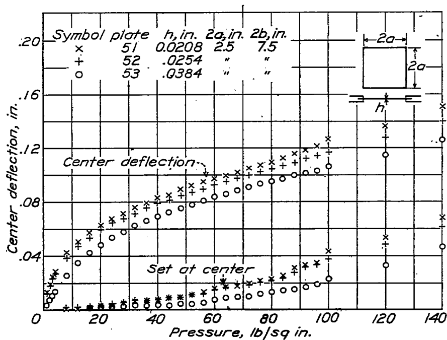
Figure 13.— Deflection and set at center of rectangular 17S-RT aluminum alloy plates with clamped edges.
