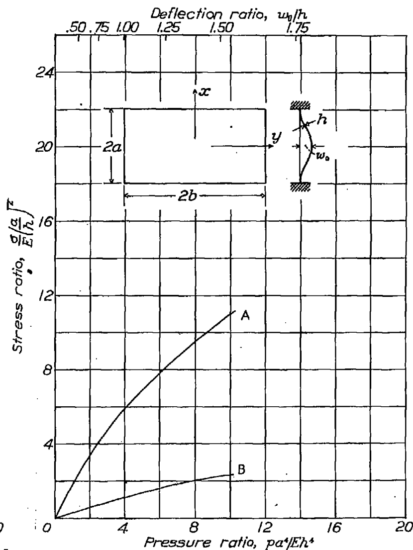
A, \frac{\sigma''_{x0}}{E} \left(\frac{a}{h}\right)^2 B, \frac{\sigma'_x}{E} \left(\frac{a}{h}\right)^2 Figure 29.- Stress in a rectangular plate ( a/b = 1/2 ) with clamped edges according to reference 11. Poisson's ratio, 0.3.
