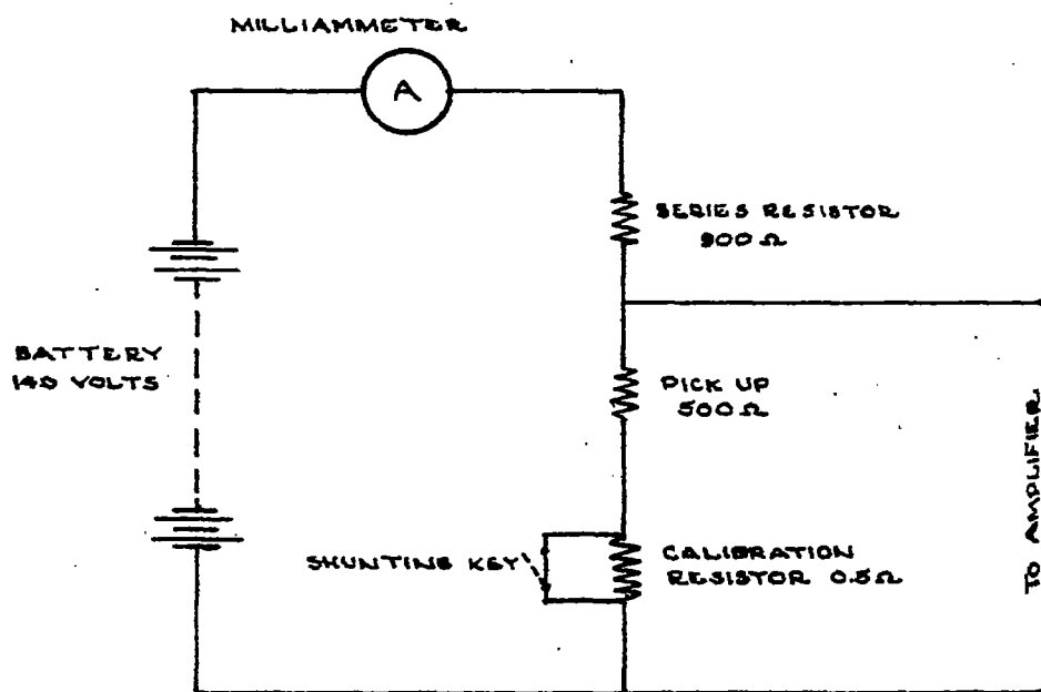
Figure 9.- Electrical circuit for dynamometer.
