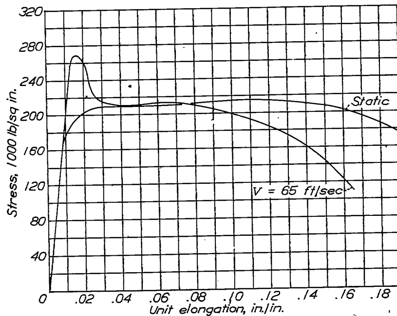
Figure 33.- Stress strain curves, 16-2 stainless steel, drawn 900°.
