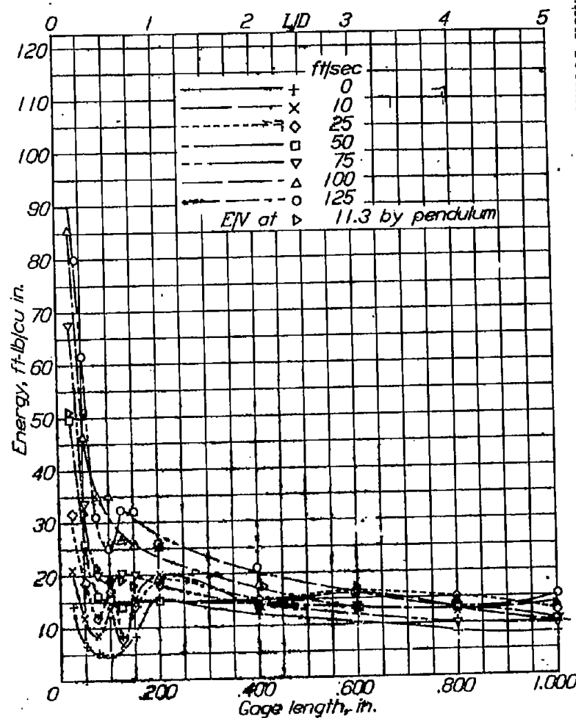
Figure 63.- Energy per unit volume against gage length.
