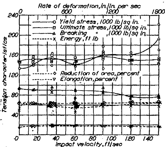
Figure 50.- Tension character- istics against impact velocity. SAE X4130 drawn 1000°F.
