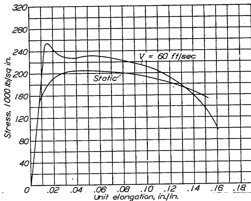
Figure 32.- Stress strain curves, 16-2 stainless steel, drawn 700°.
