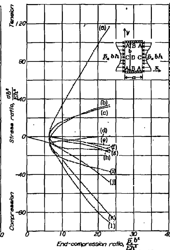
Inside of buckle (j) \sigma_x b^2/Eh^2 at A (i) \sigma_y b^2/Eh^2 at A (k) \sigma_x b^2/Eh^2 at B (l) \sigma_y b^2/Eh^2 at B (d) \sigma_x b^2/Eh^2 at C (e) \sigma_y b^2/Eh^2 at C (b) \sigma_x b^2/Eh^2 at D (c) \sigma_y b^2/Eh^2 at D Outside of buckle (j) \sigma_x b^2/Eh^2 at A (f) \sigma_y b^2/Eh^2 at A (h) \sigma_x b^2/Eh^2 at B (a) \sigma_y b^2/Eh^2 at B (d) \sigma_x b^2/Eh^2 at C (e) \sigma_y b^2/Eh^2 at C (i) \sigma_x b^2/Eh^2 at D (g) \sigma_y b^2/Eh^2 at D
