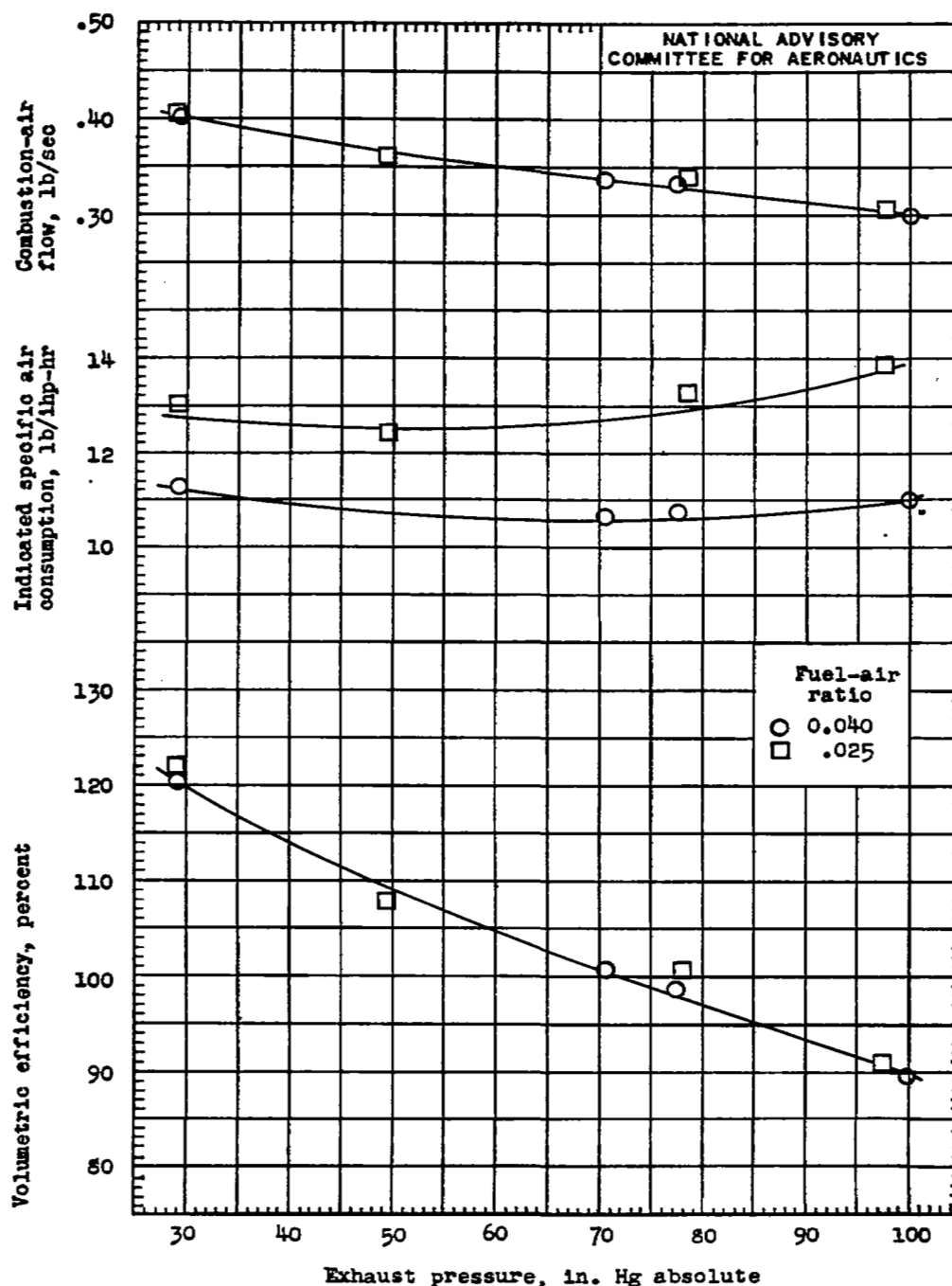
(a) Air-flow characteristics.
