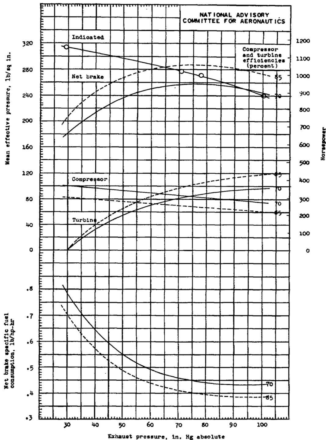
Figure 6. - Computed sea-level performance of a composite engine comprising engine converted to compression-ignition operation, compressor, and turbine at various engine exhaust pressures. Inlet-manifold pressure, 100 inches of mercury absolute; inlet-manifold air temperature, 160° F; engine speed, 1600 rps; compression ratio, 8.0; cooling-air temperature, 93° F; gear efficiency, 90 percent.
