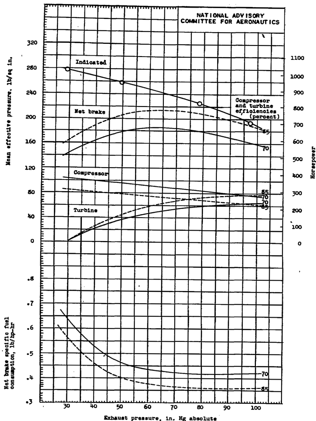
Figure 6. - Concluded. Computed sea-level performance of a composite engine comprising engine converted to compression-ignition operation, compressor, and turbine at various engine exhaust pressures. Inlet-manifold pressure, 100 inches of mercury absolute; inlet-manifold air temperature, 160° F; engine speed, 1600 rpm; compression ratio, 8.0; cooling-air temperature, 93° F; gear efficiency, 90 percent.
