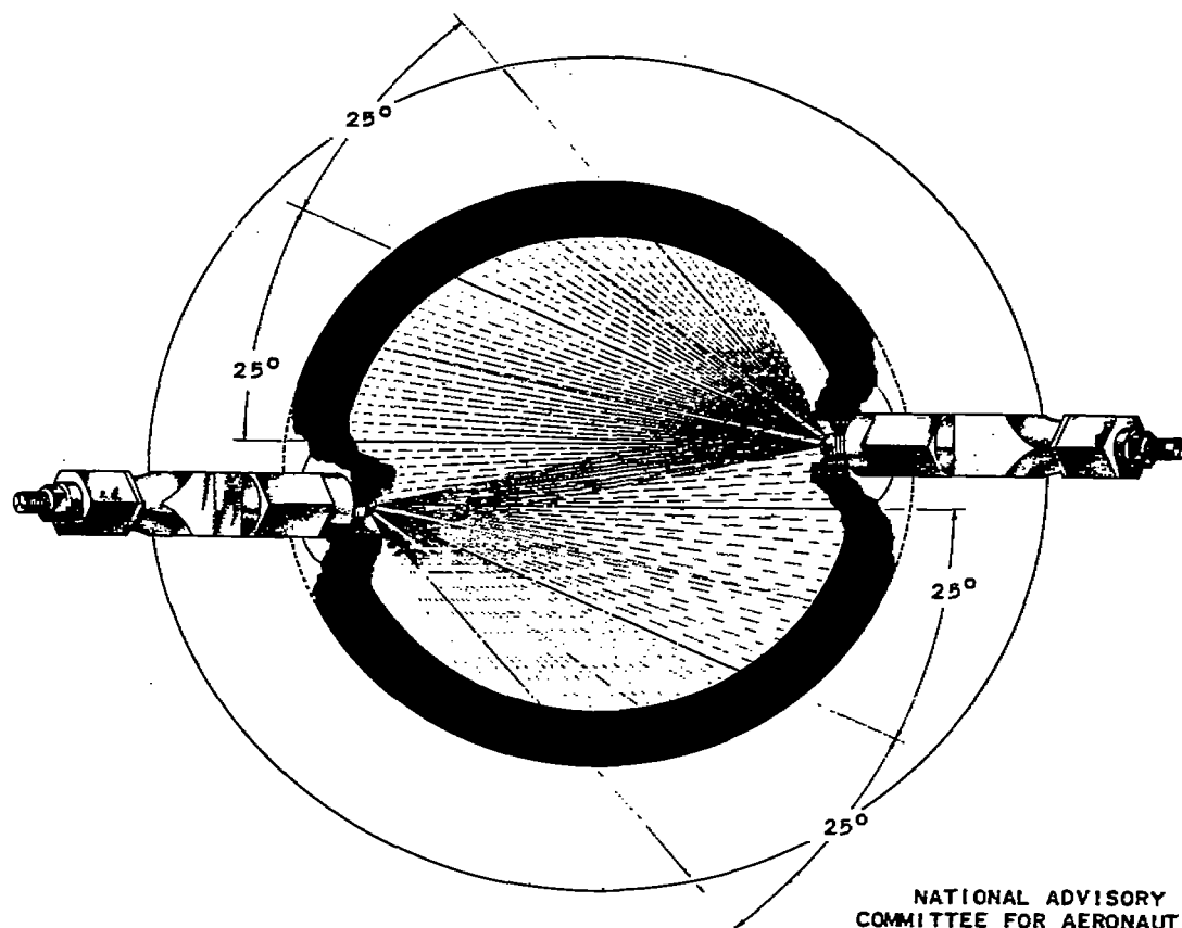
Figure 1. - Cutaway sketch of air-cooled cylinder showing location of fuel-injection nozzles in spark-plug openings and pattern of fuel-spray in cylinder.
