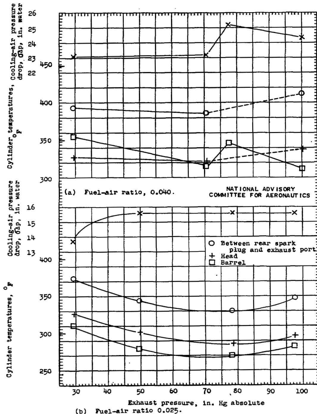
Figure 5. - Variation of cooling-air pressure drop and barrel and head temperatures of a single-cylinder engine converted to compression-ignition operation for various engine exhaust pressures. Inlet-manifold pressure, 100 inches of mercury absolute; inlet-manifold air temperature, 160° F; engine speed, 1600 rpm; cooling-air temperature, 93° F. (The broken lines indicate that temperature readings were not taken at an exhaust pressure of 77.5 in. of Hg absolute for a fuel-air ratio of 0.040.)
