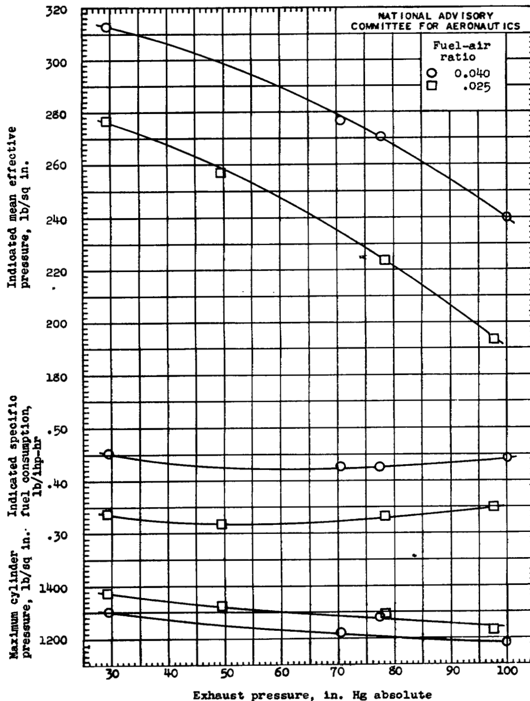
(b) Indicated mean effective pressure, indicated specific fuel consumption, and maximum cylinder pressure.
