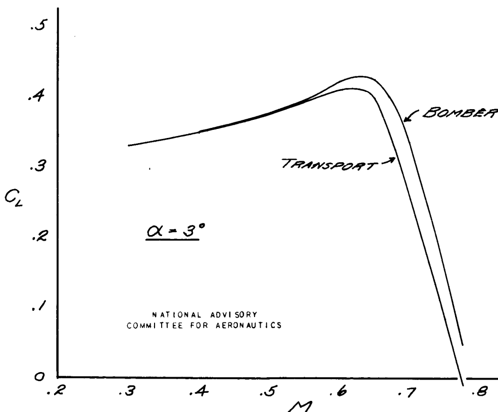
FIGURE 6(b).— VARIATION OF THE LIFT COEFFICIENT WITH MACH NUMBER FOR CONSTANT VALUES OF THE ANGLE OF ATTACK. TAIL ON.
