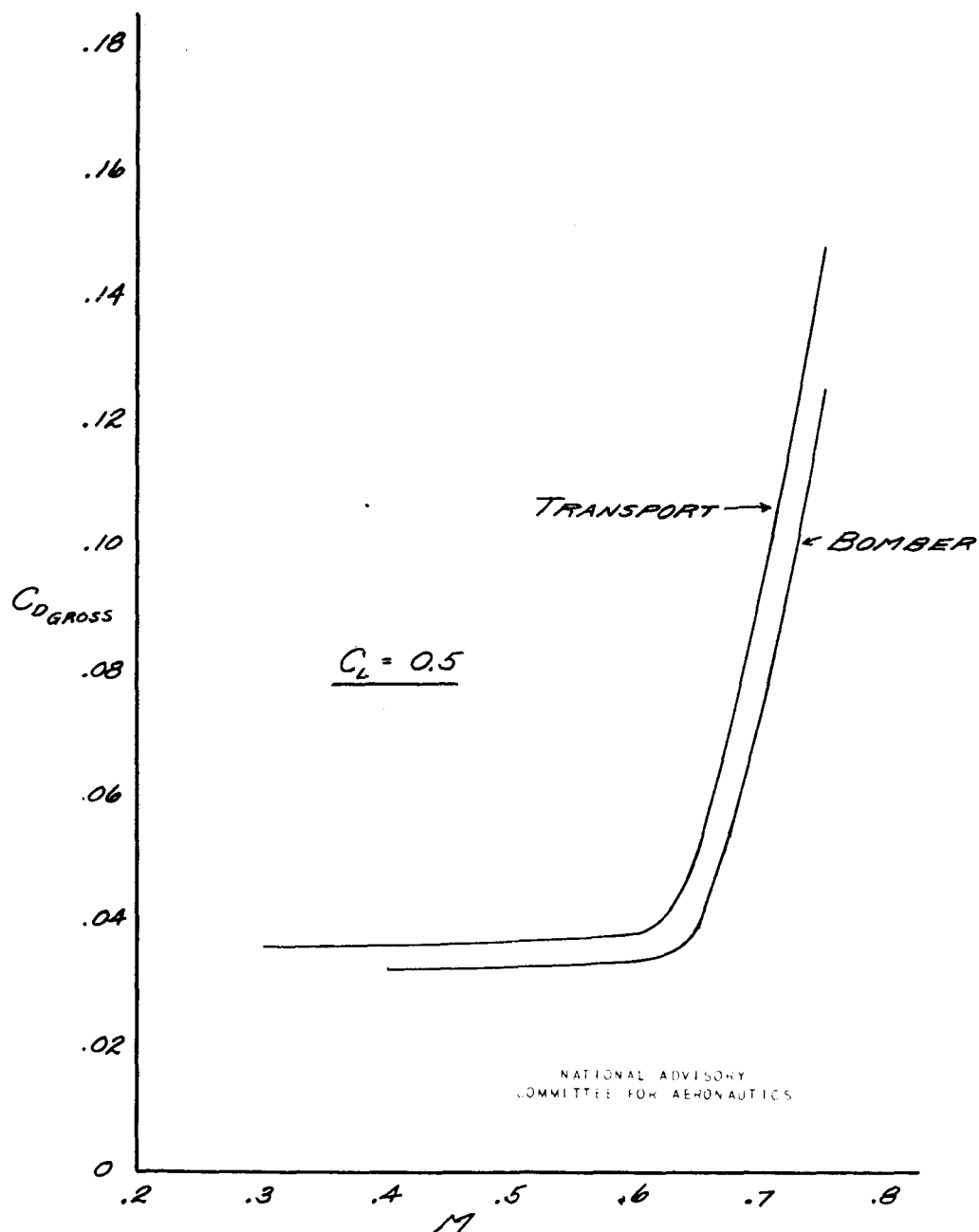
FIGURE 6(e).— VARIATION OF THE DRAG COEFFICIENT WITH MACH NUMBER FOR CONSTANT VALUES OF THE LIFT COEFFICIENT. TAIL ON.
