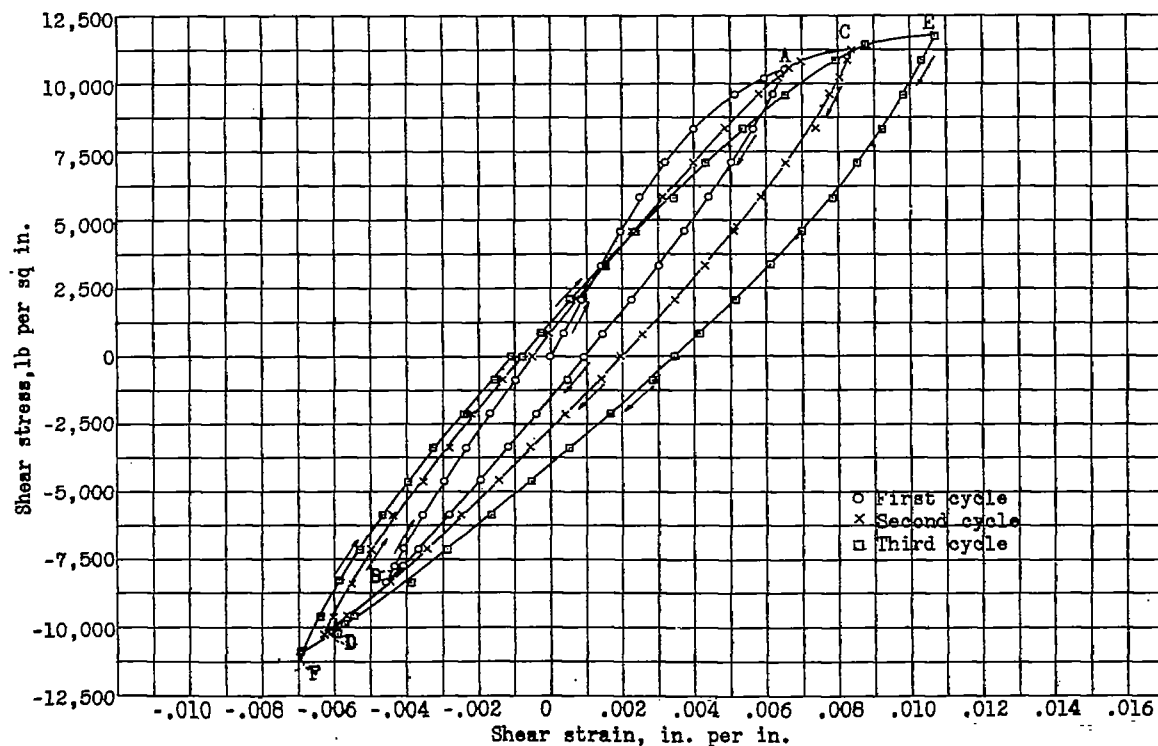
Figure 13.- Cyclic torsional stress-strain curves for magnesium alloy tubing, AM578.
