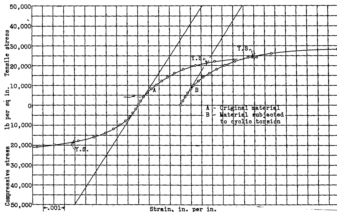
Figure 5.- Tensile and compressive stress-strain curves for copper tubing. Hard drawn copper annealed 20 minutes at 300°C.
