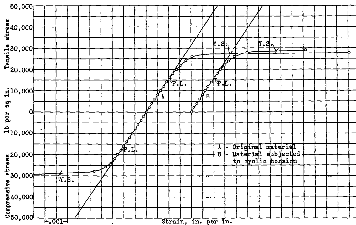
Figure 6.- Tensile and compressive stress-strain curves for brass tubing, brass (60:40).
