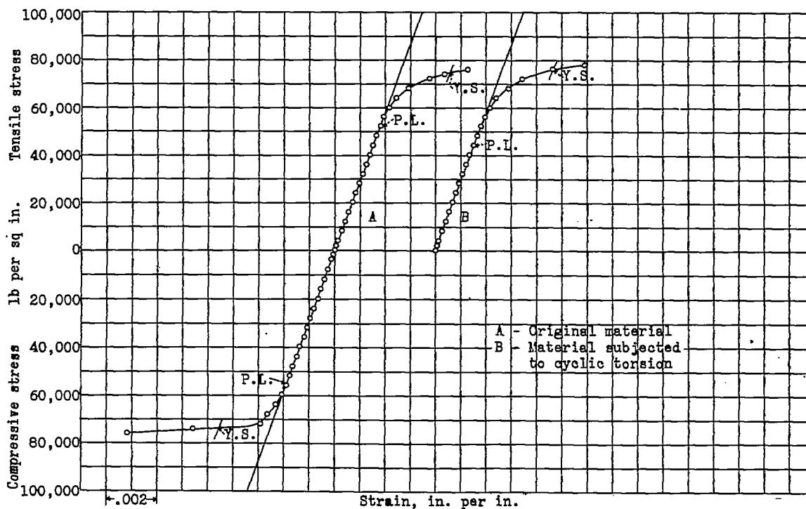
Figure 3.- Tensile and compressive stress-strain curves for seamless steel tubing, S.A.E. 1015.
