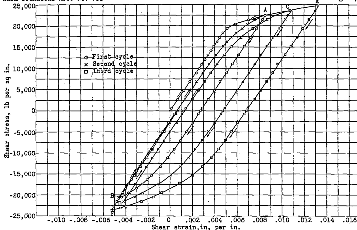
Figure 8.- Cyclic torsional stress-strain curves for aluminum alloy tubing, 17ST.
