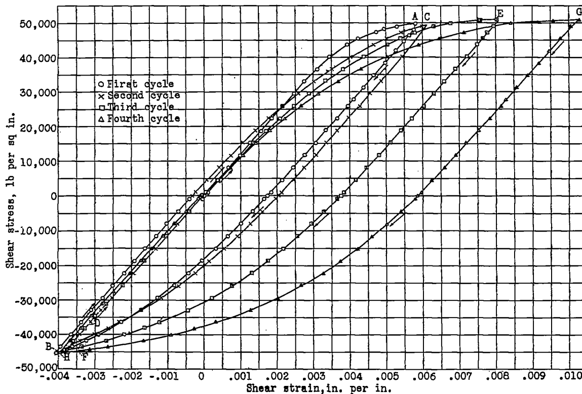
Figure 9.- Cyclic torsional stress-strain curves for seamless steel tubing, S.A.E. 1015.
