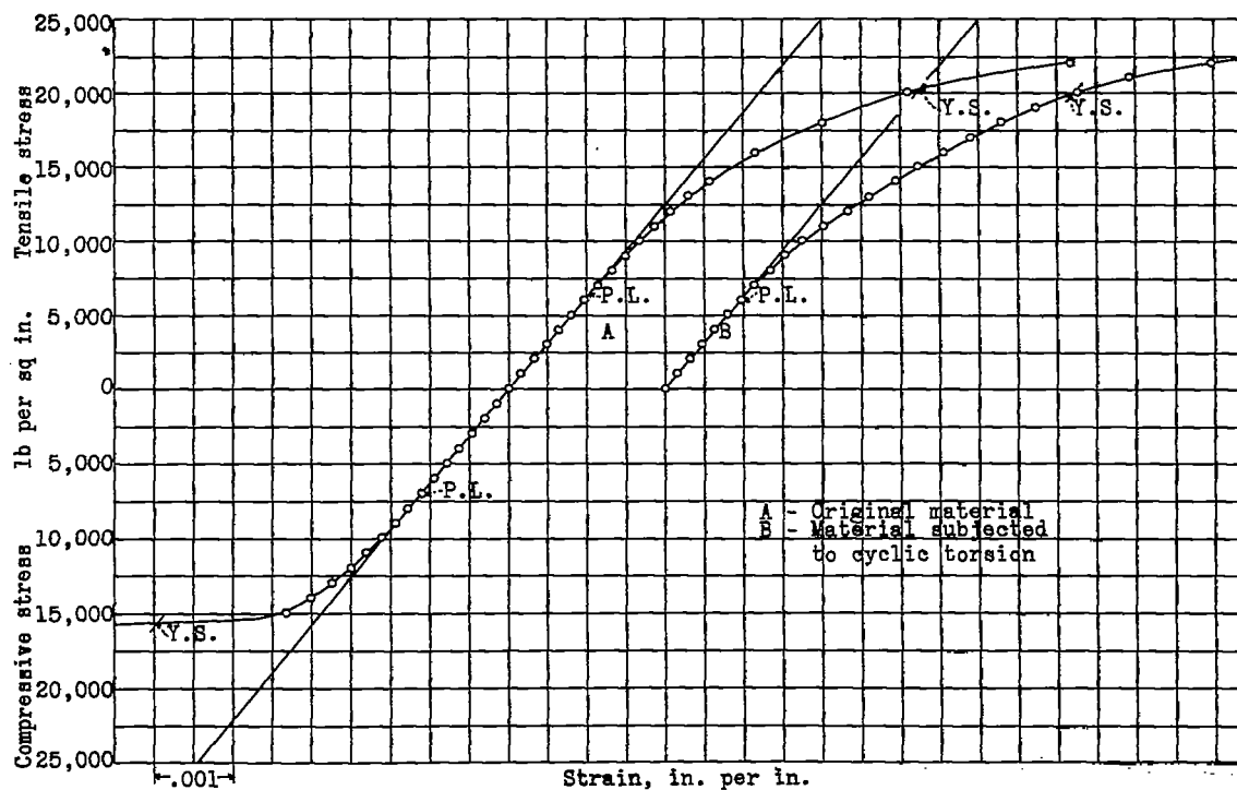
Figure 7.- Tensile and compressive stress-strain curves for magnesium alloy tubing, AM57S.
