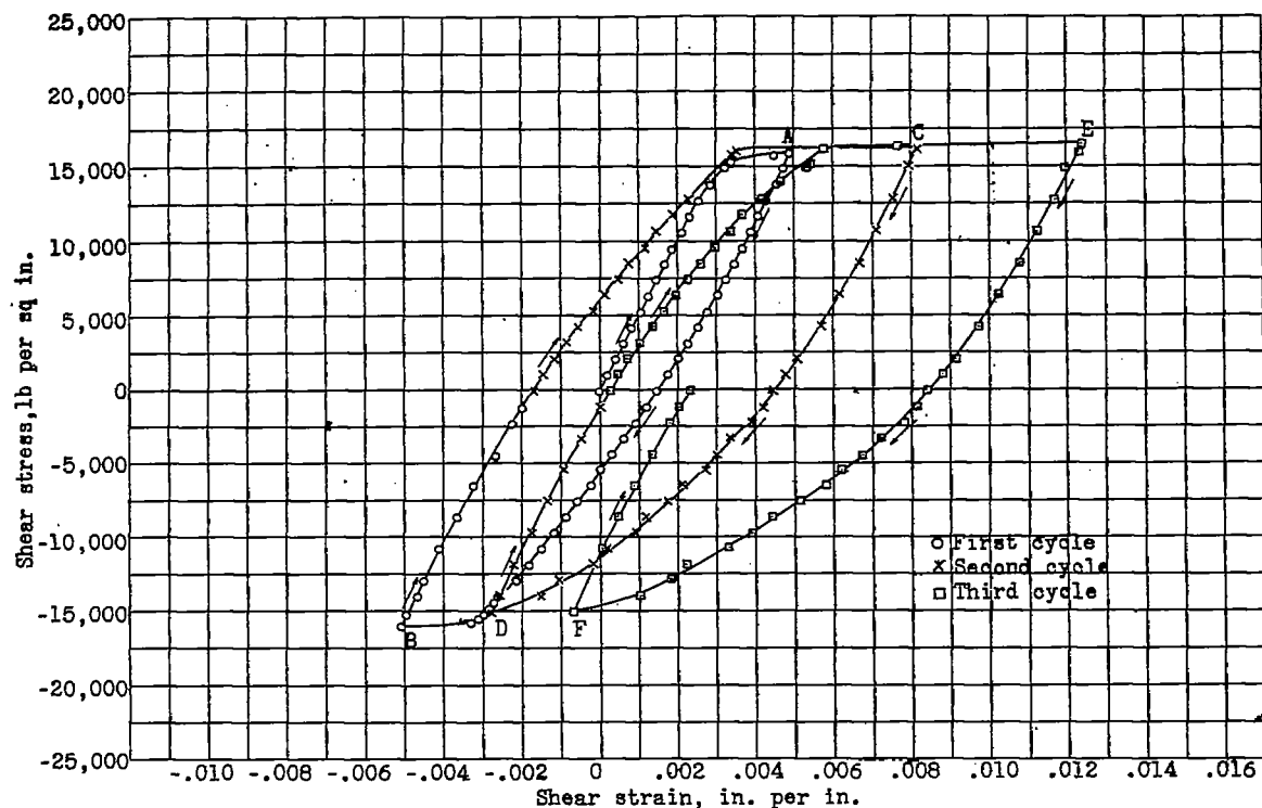
Figure 12.- Cyclic torsional stress-strain curves for brass tubing, brass (60:40).
