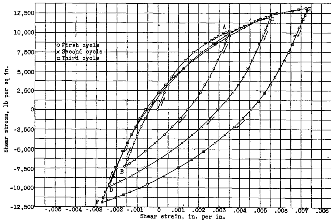
Figure 11.- Cyclic torsional stress-strain curves for copper tubing. Hard drawn copper annealed 20 minutes at 300°C.
