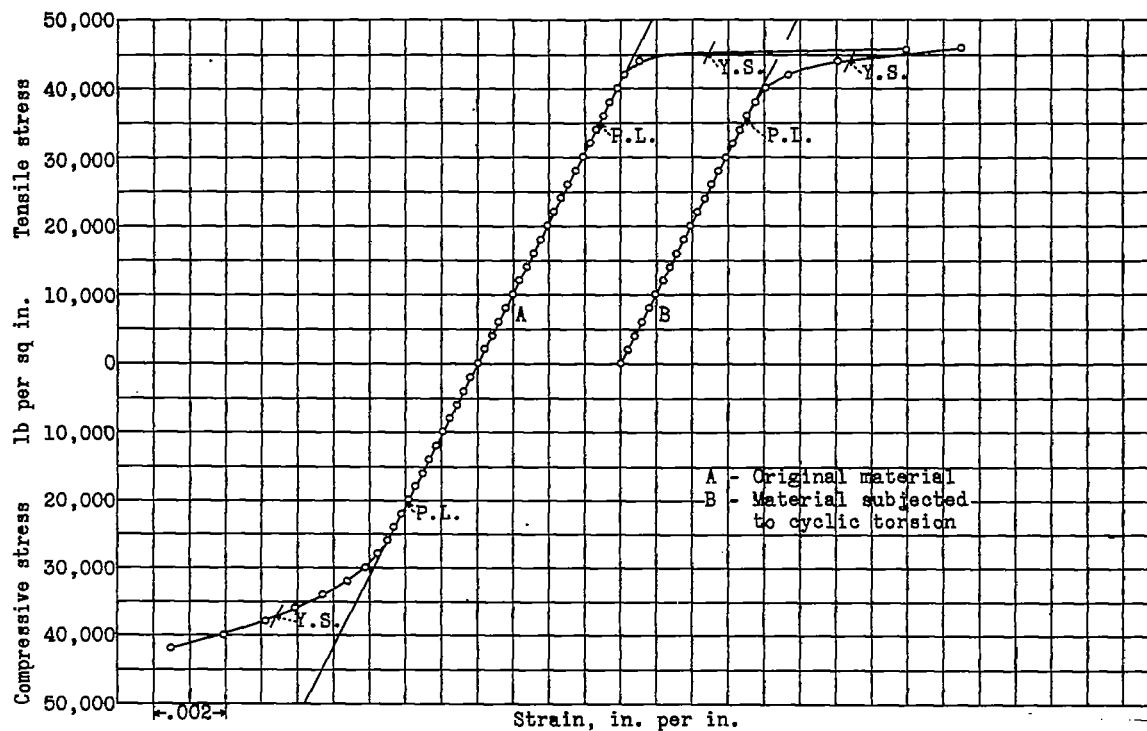
Figure 2.- Tensile and compressive stress-strain curves for aluminum alloy tubing, 17ST.
