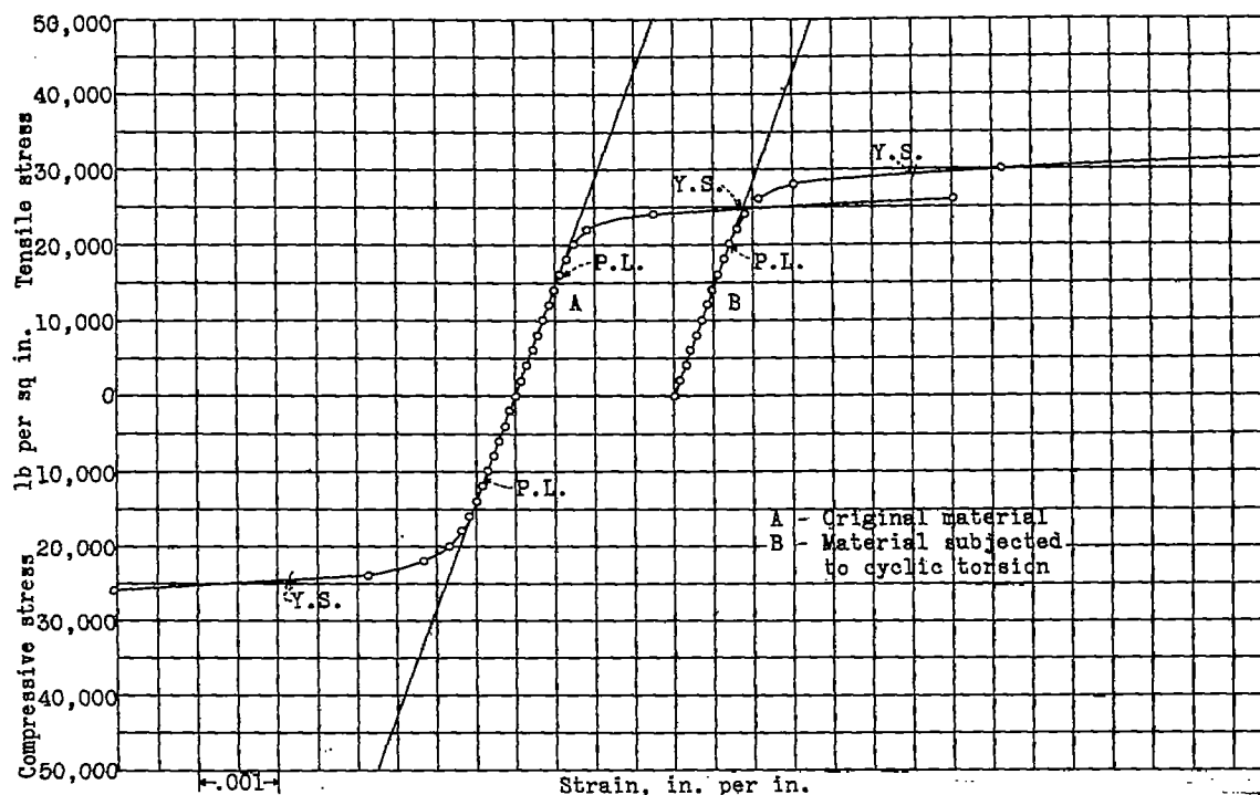
Figure 4.- Tensile and compressive stress-strain curves for wrought iron tubing.
