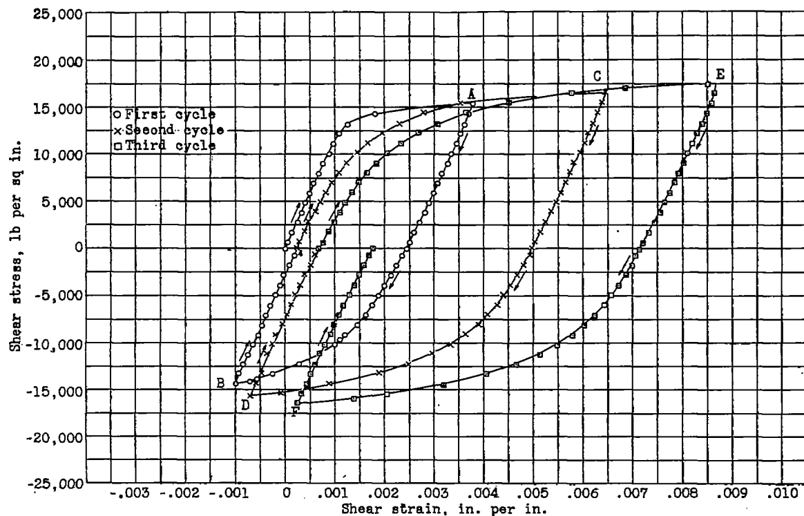
Figure 10.- Cyclic torsional stress-strain curves for wrought iron tubing.
