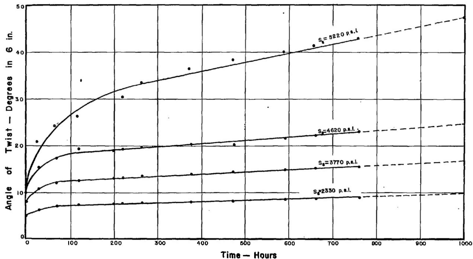
FIG. 35-STATIC TORSION CREEP TIME RELATIONS - MAT. G - SQUARE CROSS-SECTION
