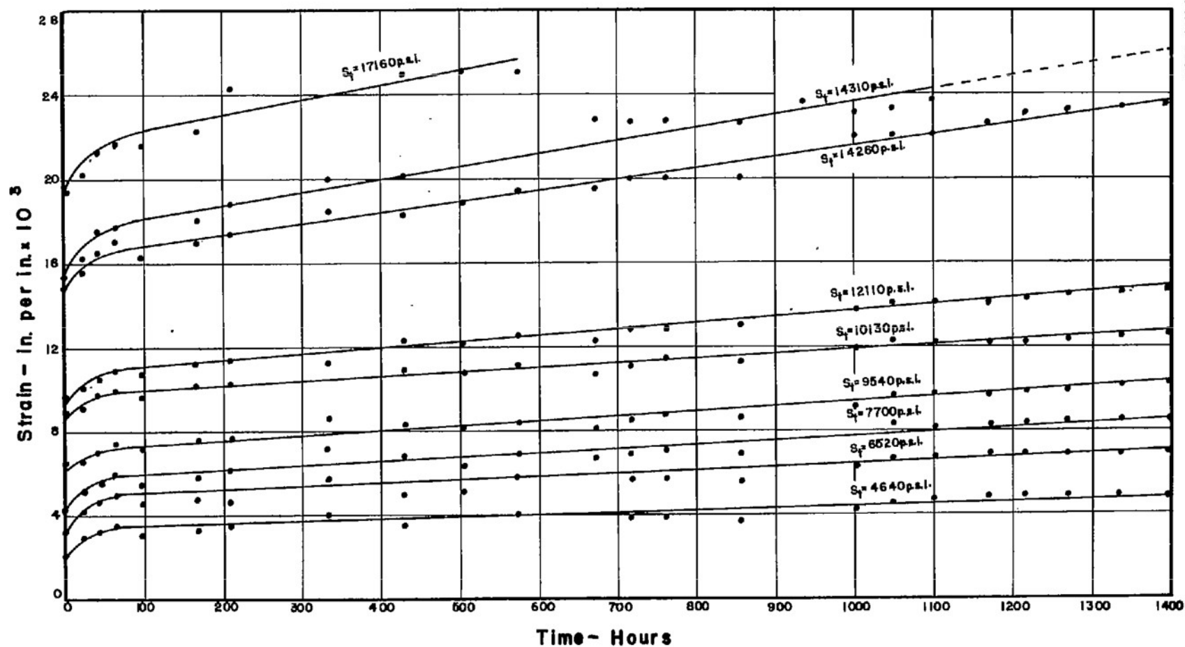
FIG.21-STATIC TENSION CREEP TIME RELATIONS - MAT.R
