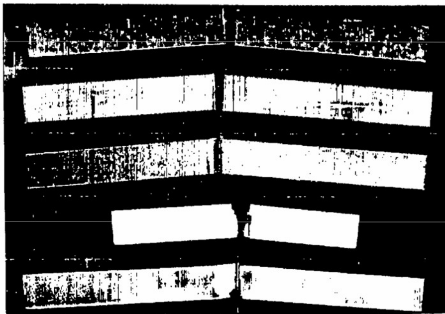
Figure 43.- Static bending specimens showing type of fracture; top to bottom, materials CL, C, R, P and G.
