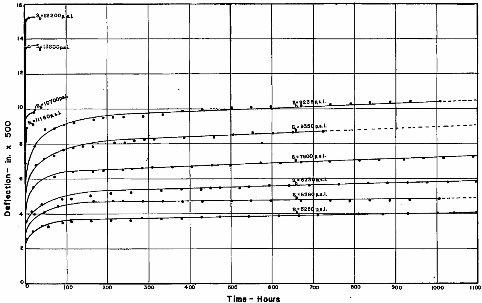
FIG.25- STATIC BENDING CREEP TIME RELATIONS-MAT. C
