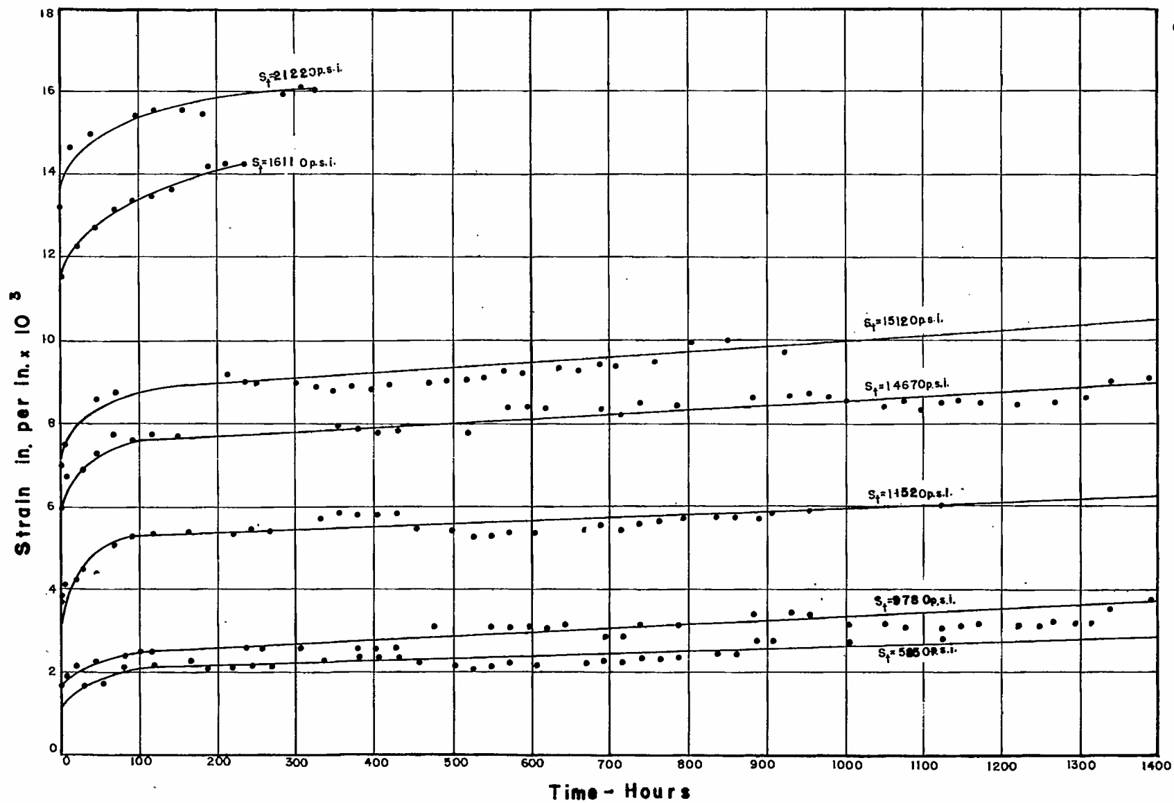
FIG. 22-STATIC TENSION CREEP TIME RELATIONS - MAT. P
