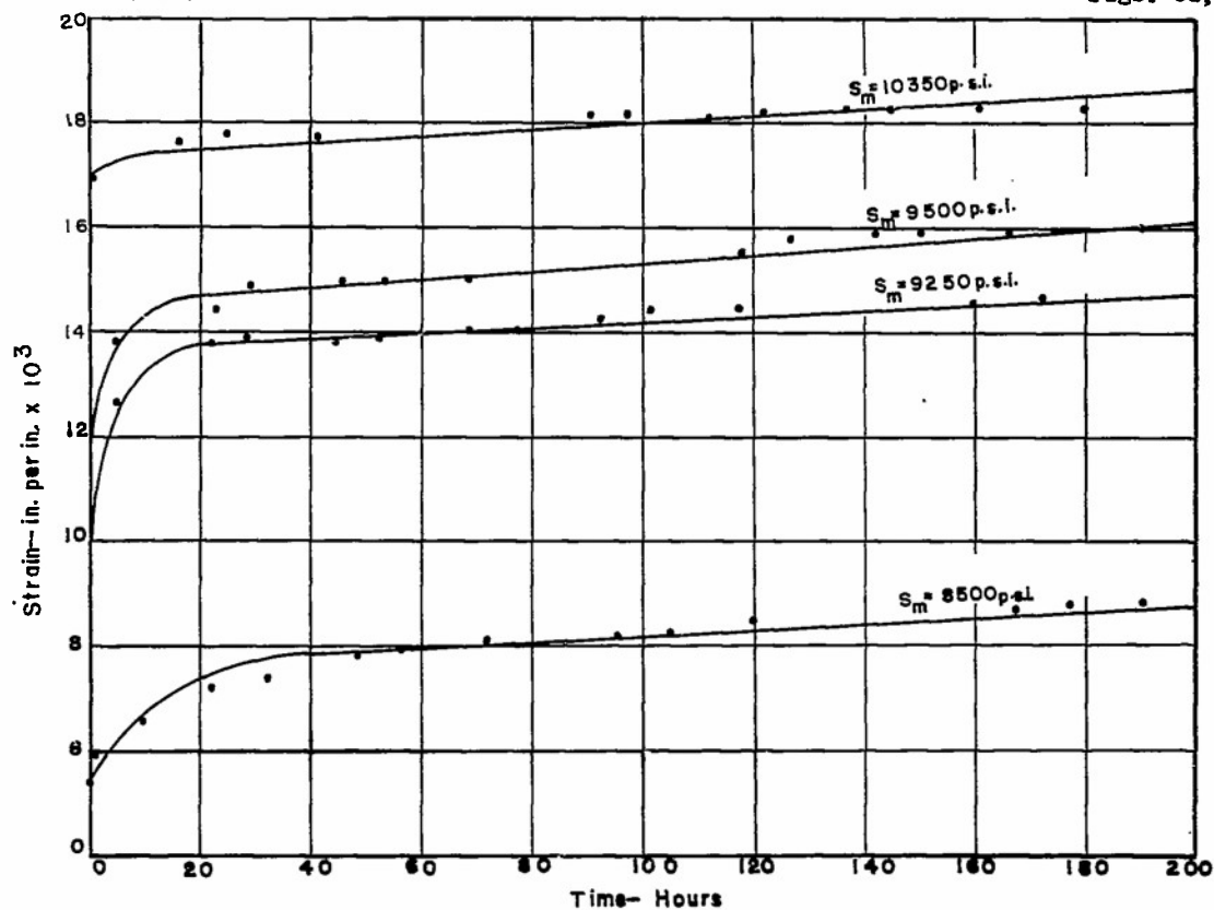
FIG.38-DYNAMIC TENSION CREEP-TIME RELATIONS - MAT. R
