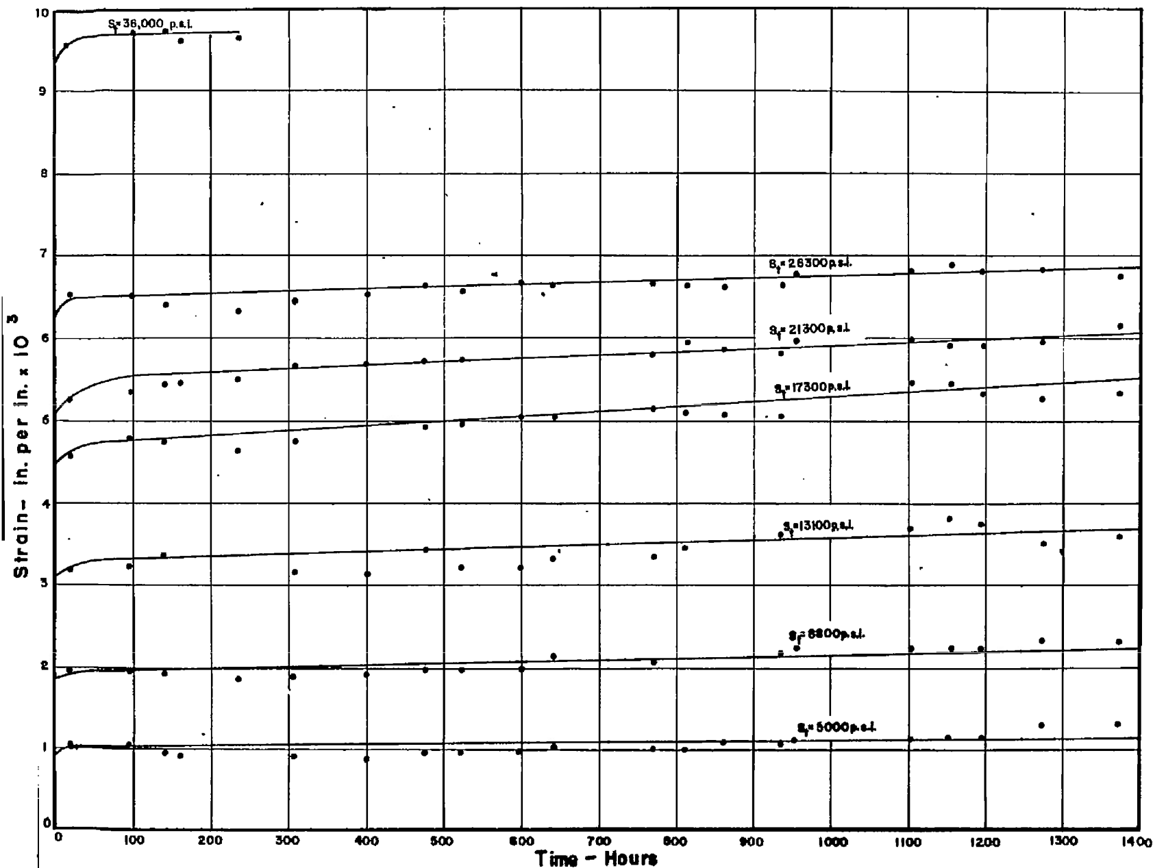
FIG.23-STATIC TENSION CREEP TIME RELATIONS- MAT. G
