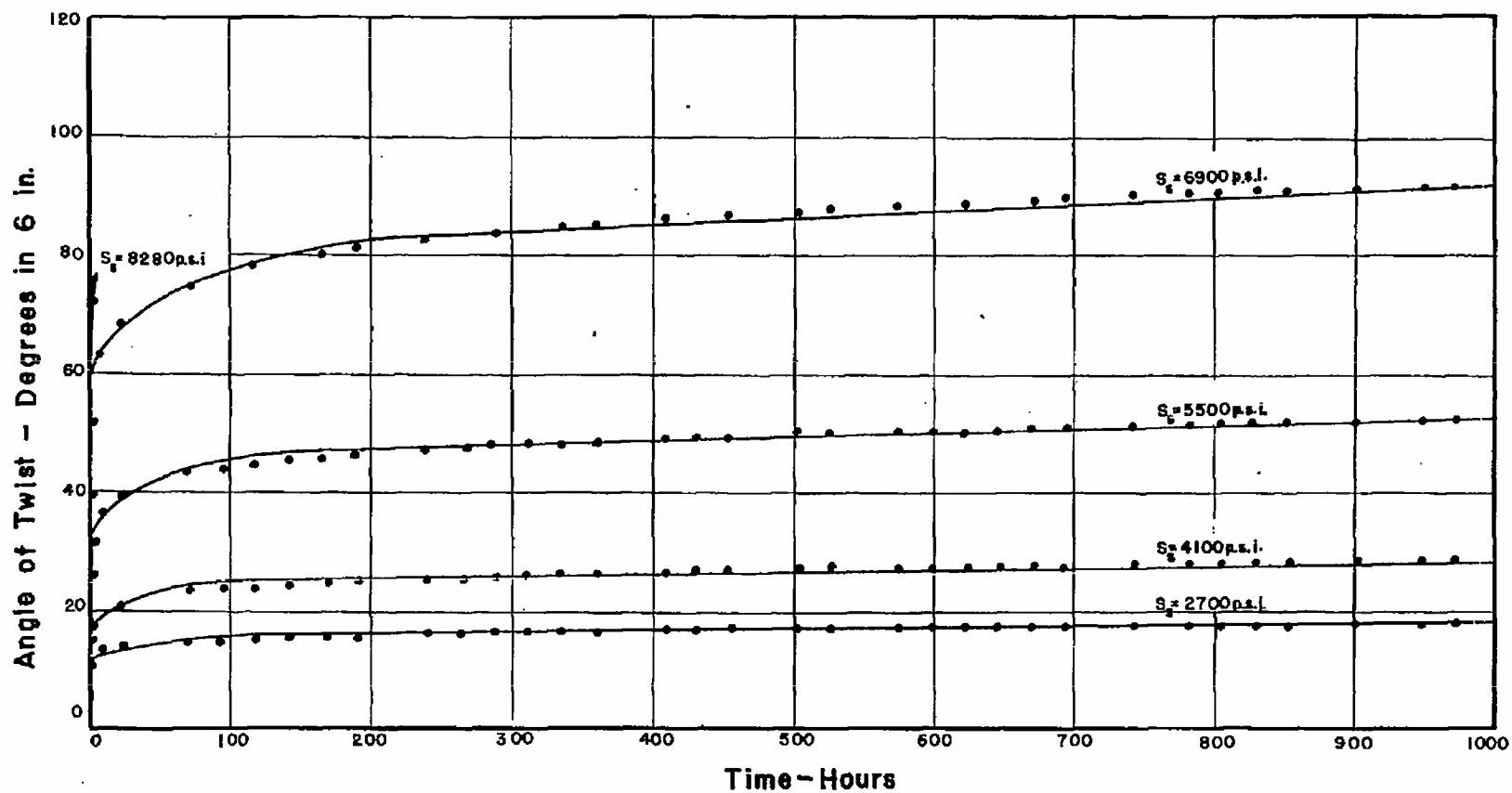
FIG.32-STATIC TORSION CREEP TIME RELATIONS-MAT. C-SQUARE CROSS-SECTION
