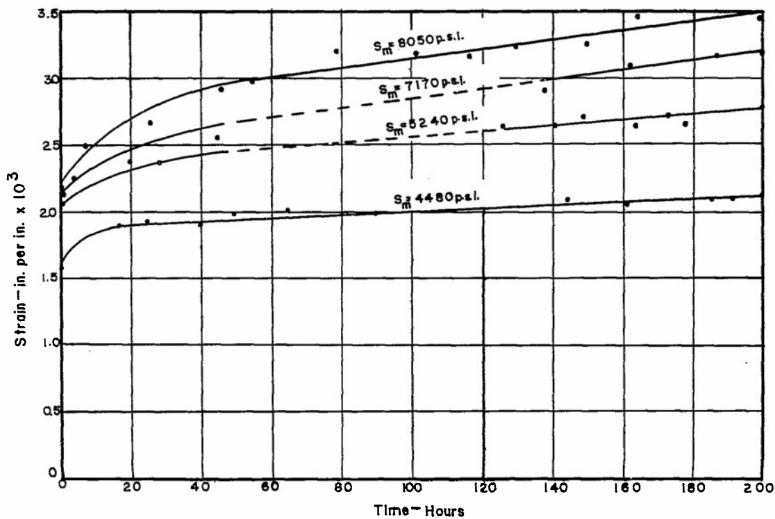
FIG.39-DYNAMIC TENSION CREEP-TIME RELATIONS - MAT. P
