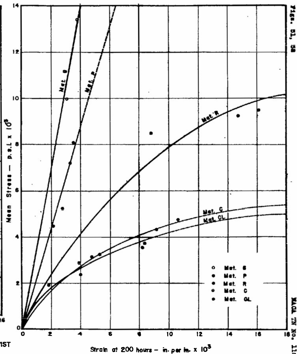
FIG. 52- COMPARISON OF DYNAMIC TENSION CREEP STRAINS
