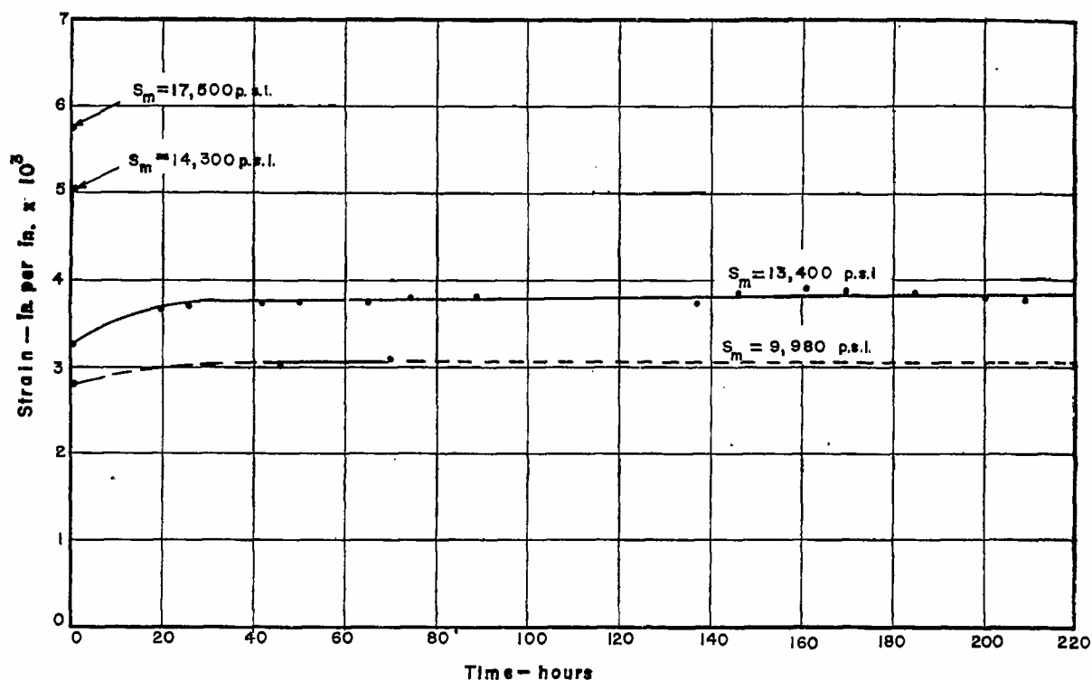
FIG. 40-DYNAMIC TENSION CREEP-TIME RELATIONS— MAT. G
