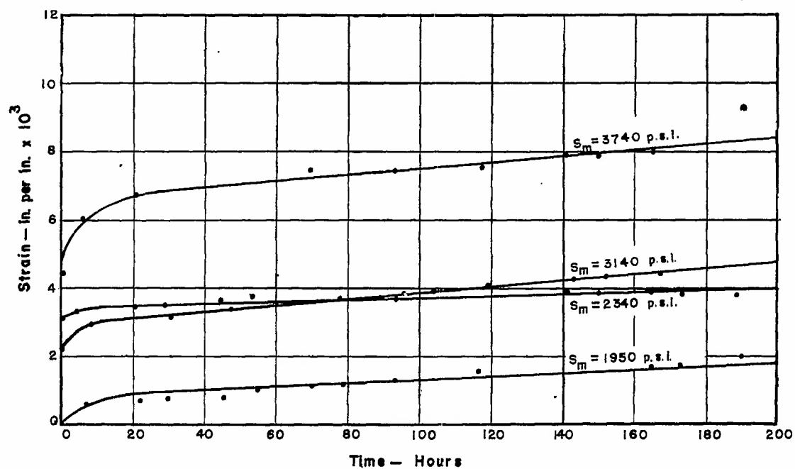
FIG.36 - DYNAMIC TENSION CREEP-TIME RELATIONS - MAT. CL
