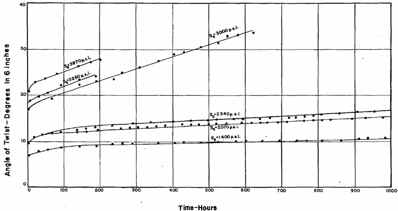
FIG. 30-STATIC TORSION CREEP TIME RELATIONS - MAT. P-ROUND CROSS-SECTION
