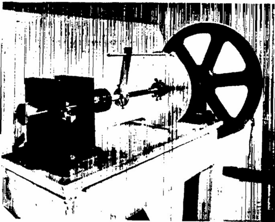
Figure 10.- Static creep torsion unit showing method of loading.
