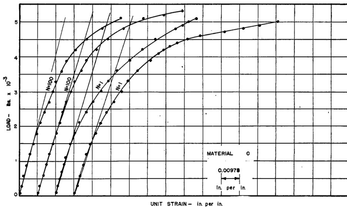
FIG. 13a - STATIC COMPRESSION LOAD-STRAIN DIAGRAMS
