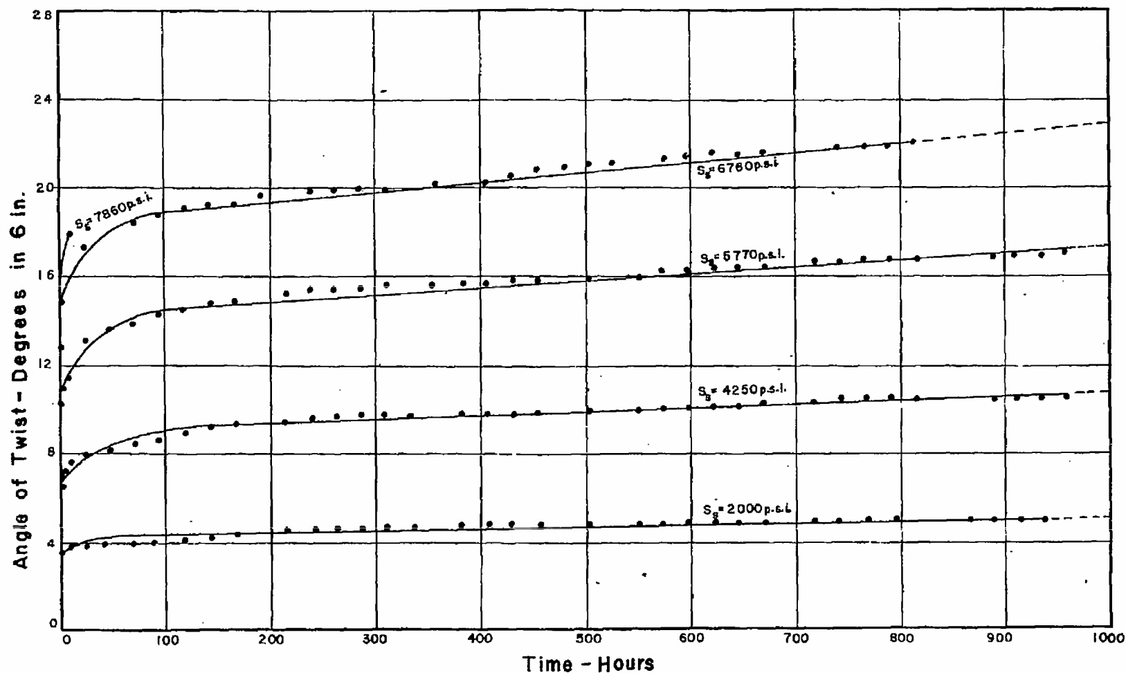
FIG. 34-STATIC TORSION CREEP TIME RELATIONS- MAT. P- SQUARE CROSS-SECTION
