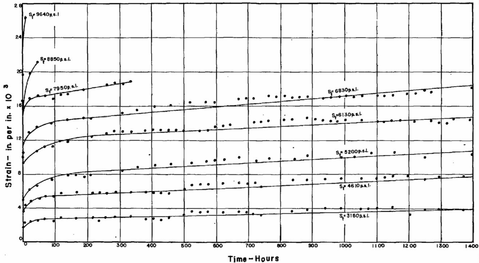
FIG.20-STATIC TENSION CREEP TIME RELATIONS - MAT. C
