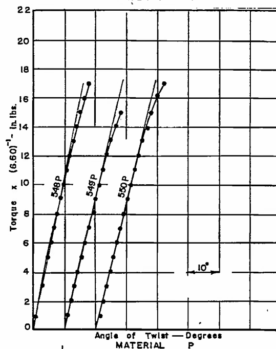
FIG. 15 - STATIC TORSION TORQUE-TWIST DIAGRAMS ROUND CROSS-SECTIONS
