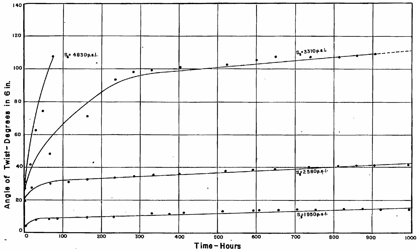
FIG.29-STATIC TORSION CREEP TIME RELATIONS MAT. R- ROUND CROSS-SECTION
