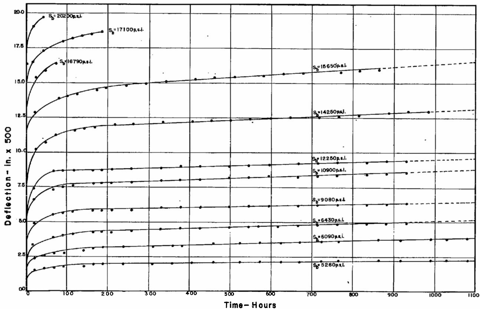
FIG.26-STATIC BENDING CREEP TIME RELATIONS - MAT. R
