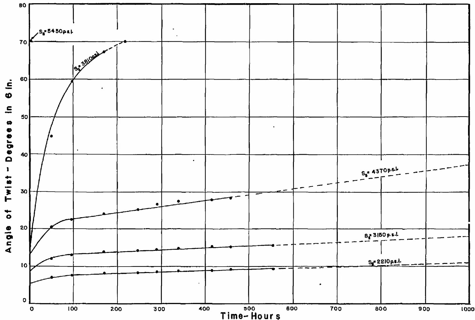
FIG.31-STATIC TORSION CREEP TIME RELATIONS - MAT. G - ROUND CROSS-SECTION
