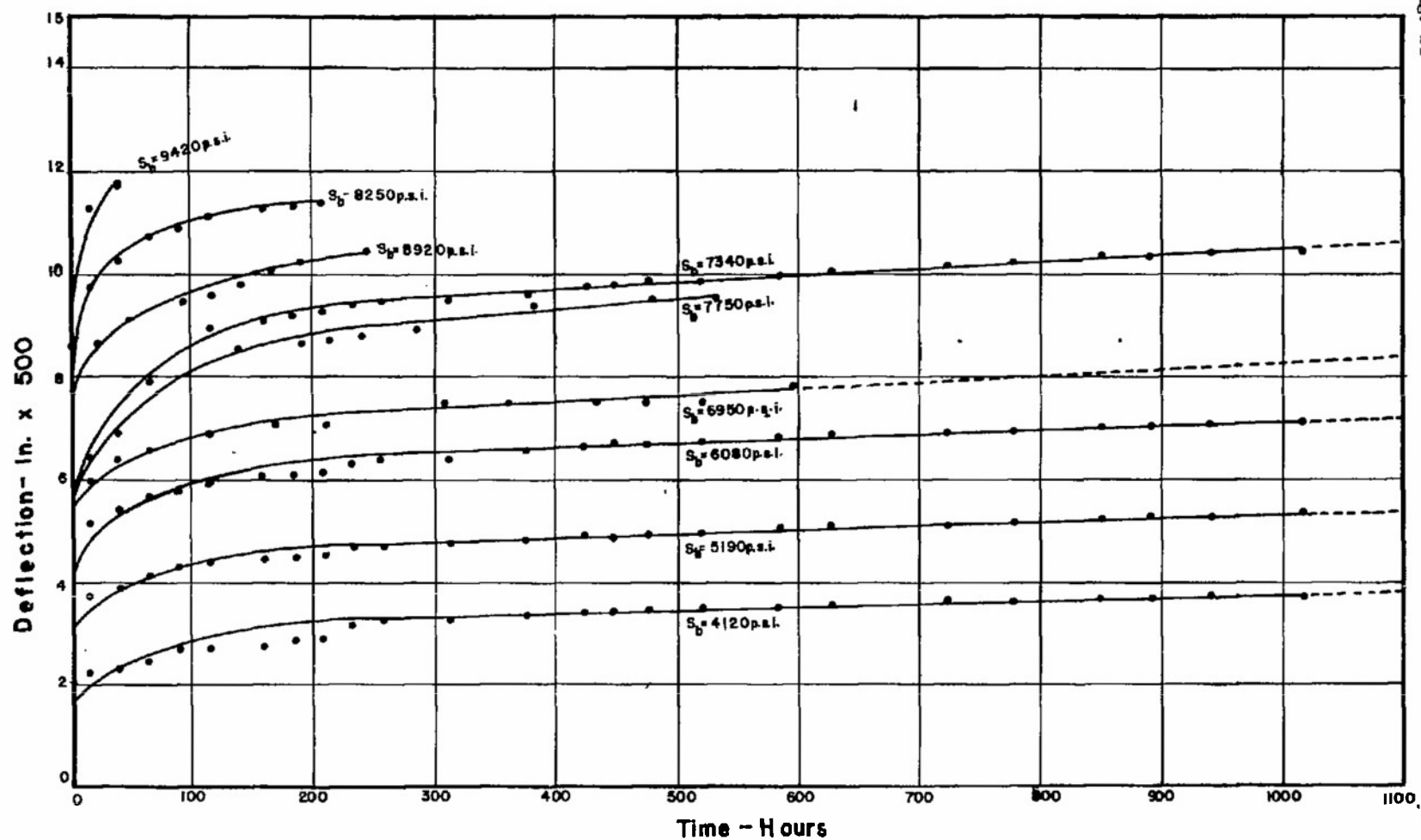
FIG.24-STATIC BENDING CREEP TIME RELATIONS - MAT.CL
