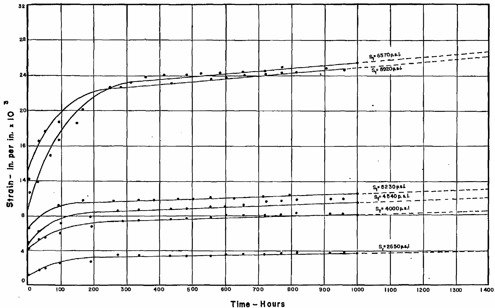
FIG. 19-STATIC TENSION CREEP TIME RELATIONS- MAT. CL.
