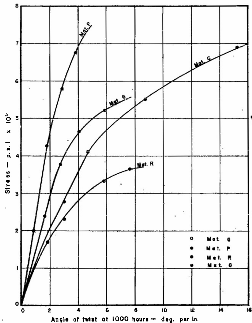
FIG. 51- COMPARISON OF STATIC TORSION CREEP ANGLES OF TWIST SQUARE CROSS-SECTION
