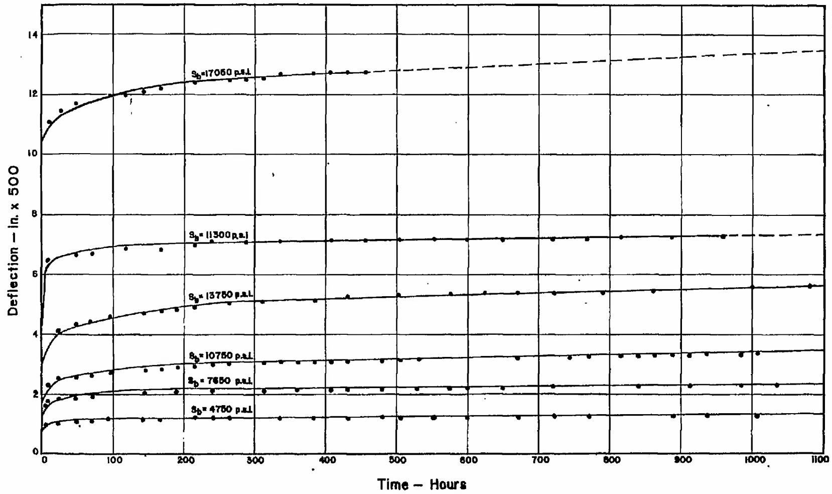
FIG.27.-STATIC BENDING CREEP TIME RELATIONS - MAT. P
