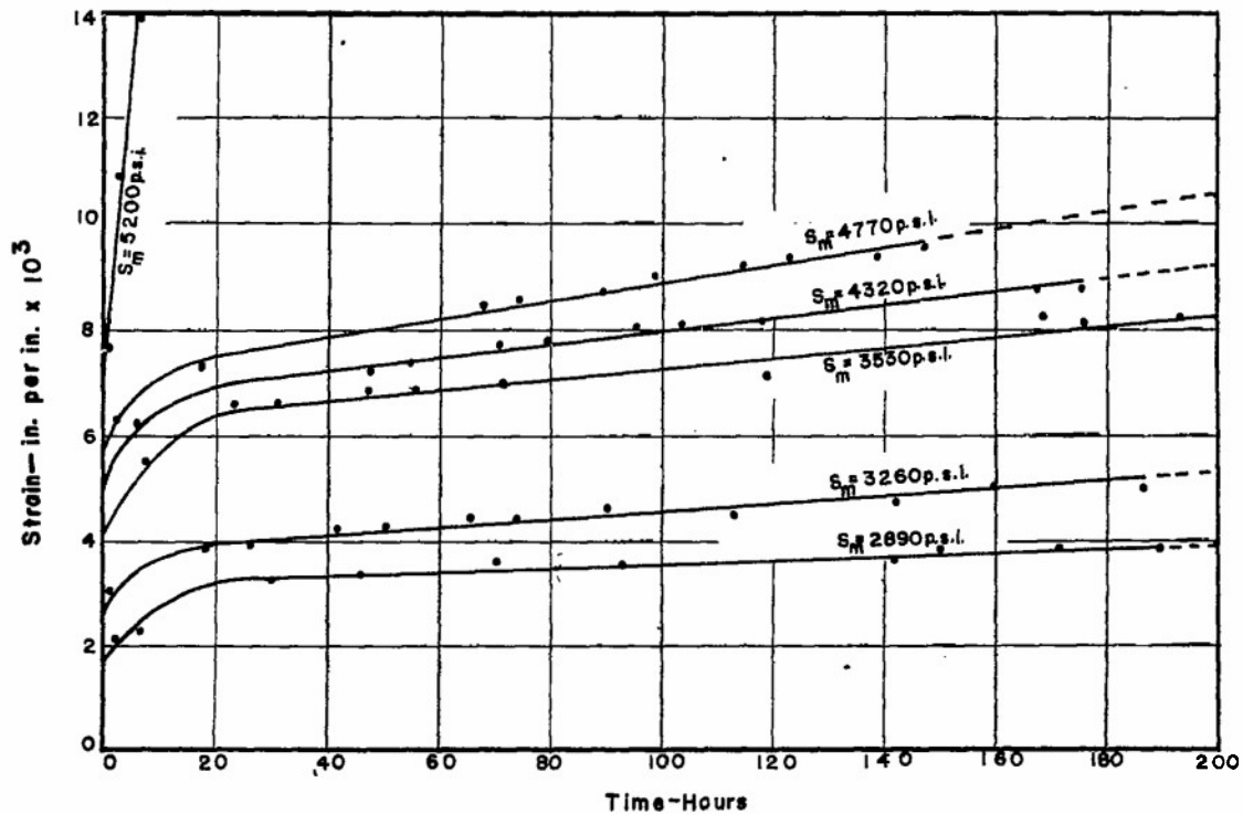
FIG.37-DYNAMIC TENSION CREEP-TIME RELATIONS-MAT. C
