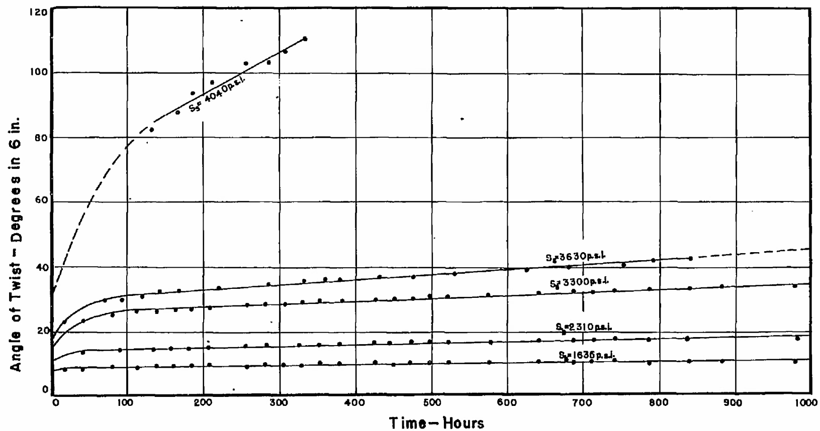
FIG.33-STATIC TORSION CREEP TIME RELATIONS - MAT. R - SQUARE CROSS-SECTION
