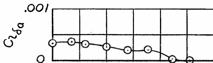
(a) Aileron effectiveness.
