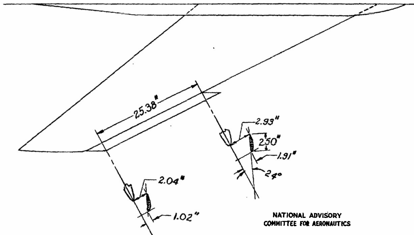
Figure 7.- Partial-span slat 1.
