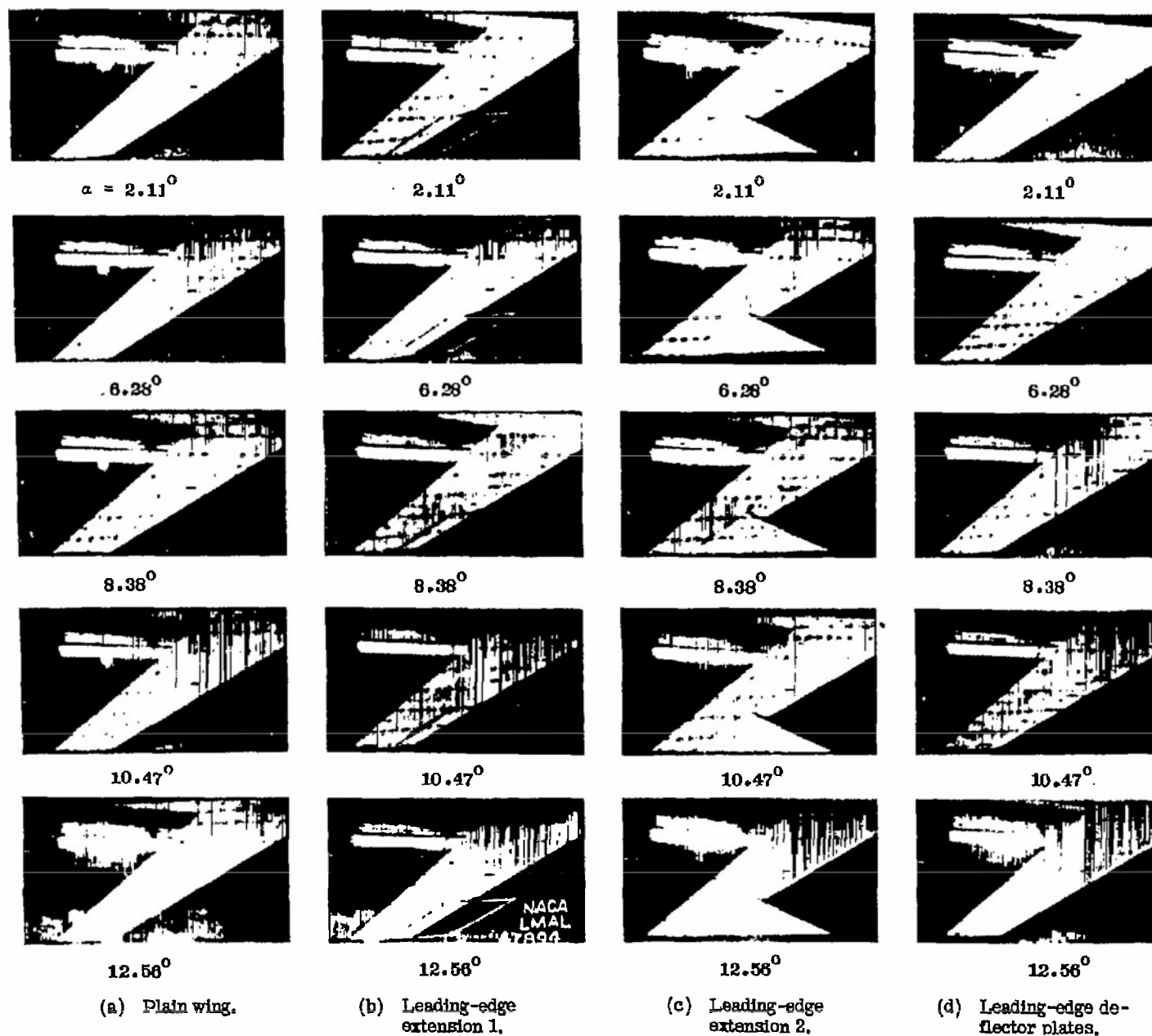
Figure 28.- Tuft studies over upper surface of 60° swept-back wing with leading-edge extensions and six deflector plates.
