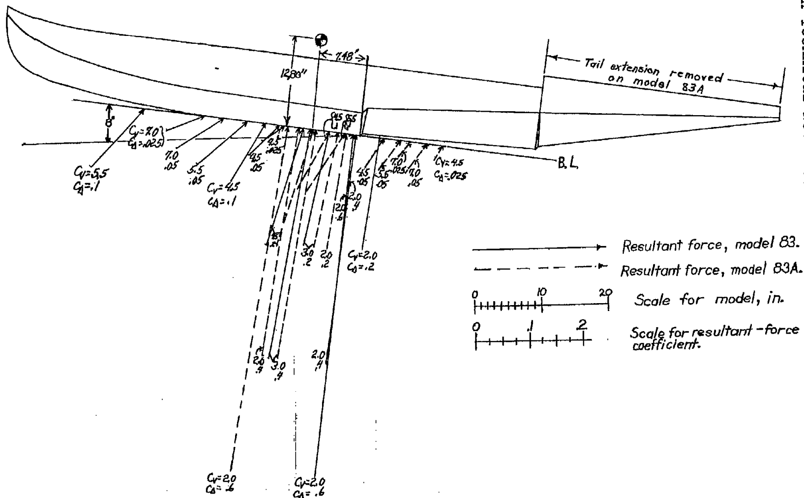
Figure 10.- Models 83 and 83A. Vector diagram of resultant forces, \gamma=8^\circ . Resultant-force coefficient = \sqrt{C_A^2 + C_R^2} ; direction of resultant force, \theta = \tan^{-1} A/R ; beam of model, b = 17.72 inches.
