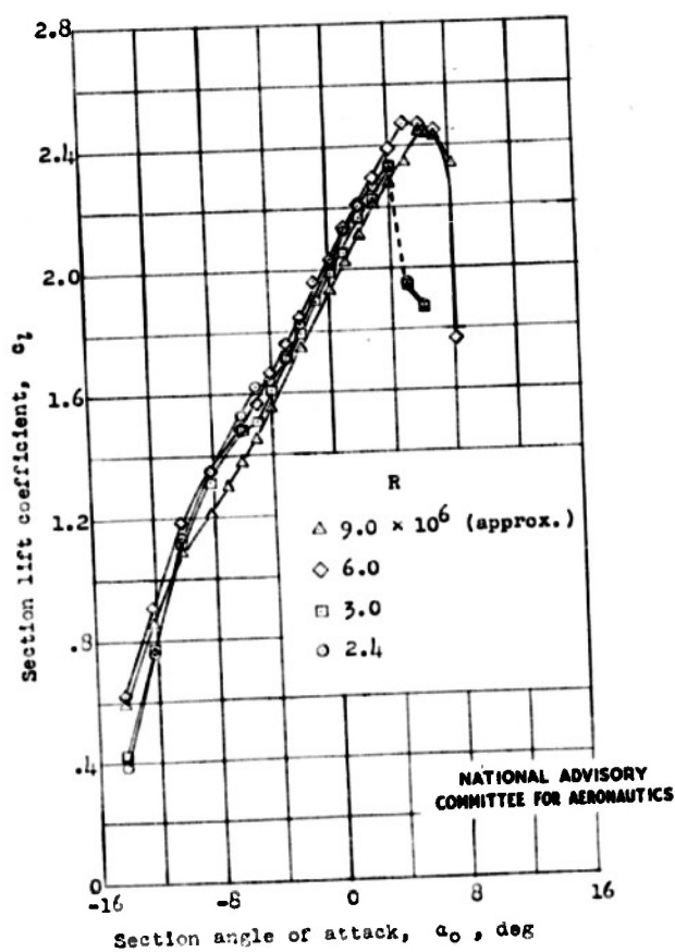
Figure 12.- Section lift characteristics of the NACA 65-210 airfoil with slotted flap 1 at various Reynolds numbers. \delta_f = 4.5^\circ ; x = 0.92 ; y = 0.95 .
