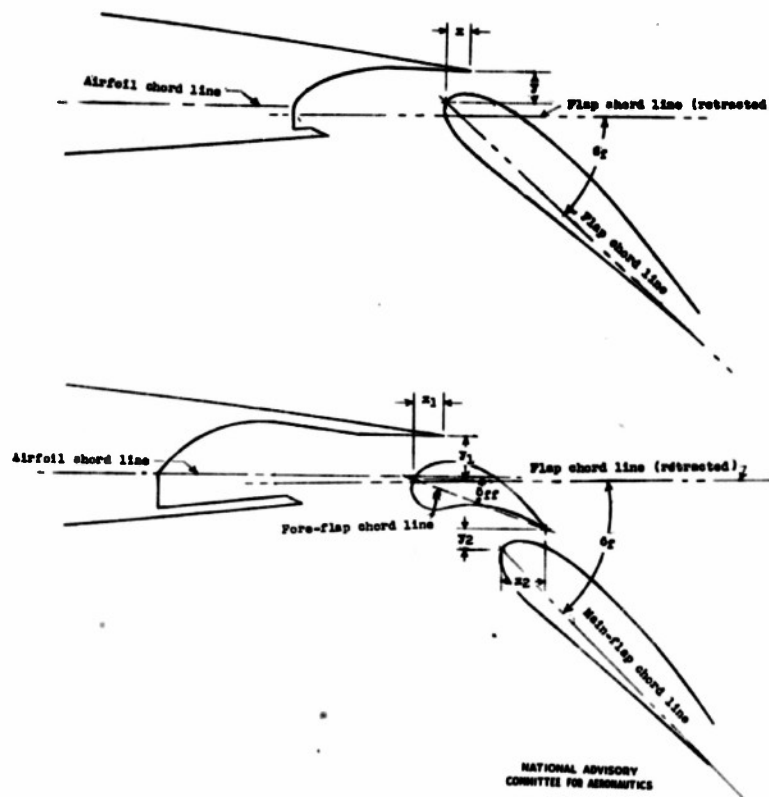
(b) Variables used to define flap configurations.
