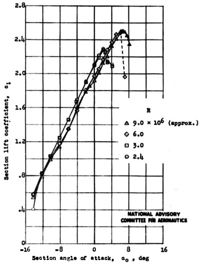
Figure 15.- Section lift characteristics of the NACA 65-210 airfoil with slotted flap 2 at various Reynolds numbers. \delta_f = 41.5^\circ ; x = 1.42 ; y = 0.92 .
