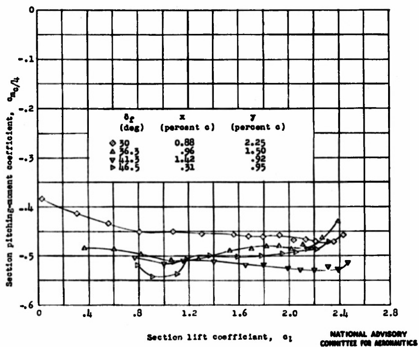
Figure 16.- Section pitching-moment characteristics of the NACA 65-210 airfoil with slotted flap 2. R = 6.0 \times 10^6 (approx.).
