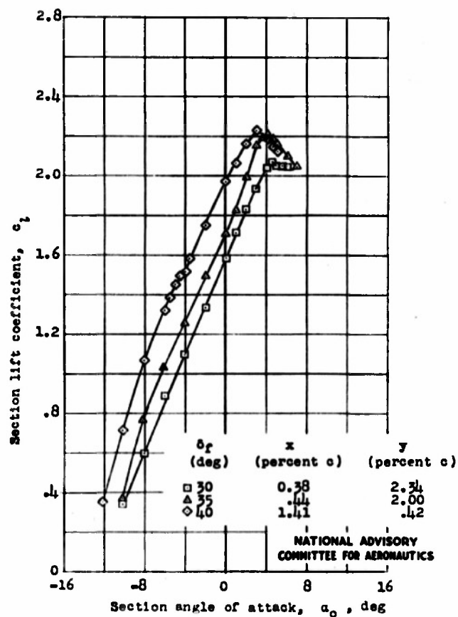
Figure 17.- Section lift characteristics of the NACA 65-210 airfoil with slotted flap 3. R = 2.4 \times 10^6 (approx.); smooth.
