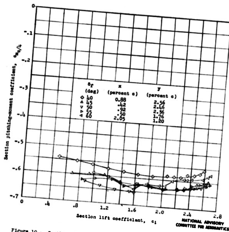
Figure 10.- Section pitching-moment characteristics of the NACA 65-210 airfoil with a 0.312c double slotted flap. R = 6.0 \times 10^6 (approx.).
