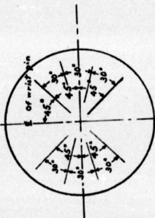
Chart showing location of oil-drain holes
