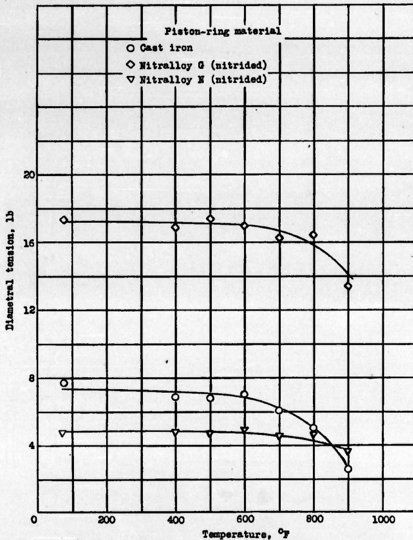
Figure 7.- Effect of piston-ring temperature on diametral tension. (Rings held 1 hr at each temperature.)
