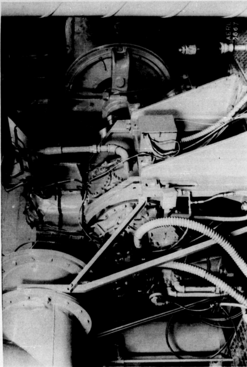
Figure 2.- Single-cylinder-engine assembly.
