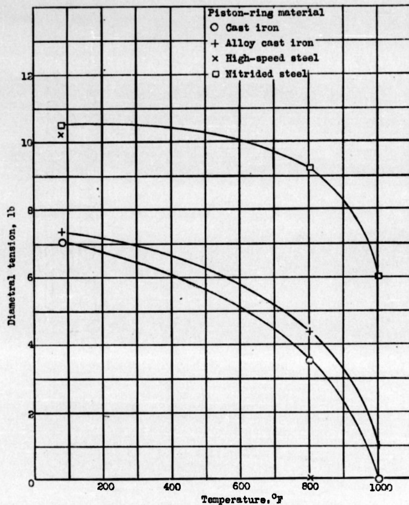
Figure 6.-- Effect of piston-ring temperature on diametral tension. (Rings hold 6 to 8 hr at each temperature.)
