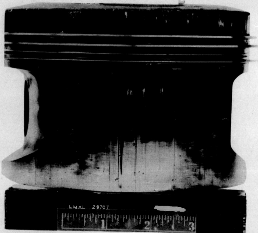
Figure 20.- Piston assembly after high-output tests. High-tension oil rings.
