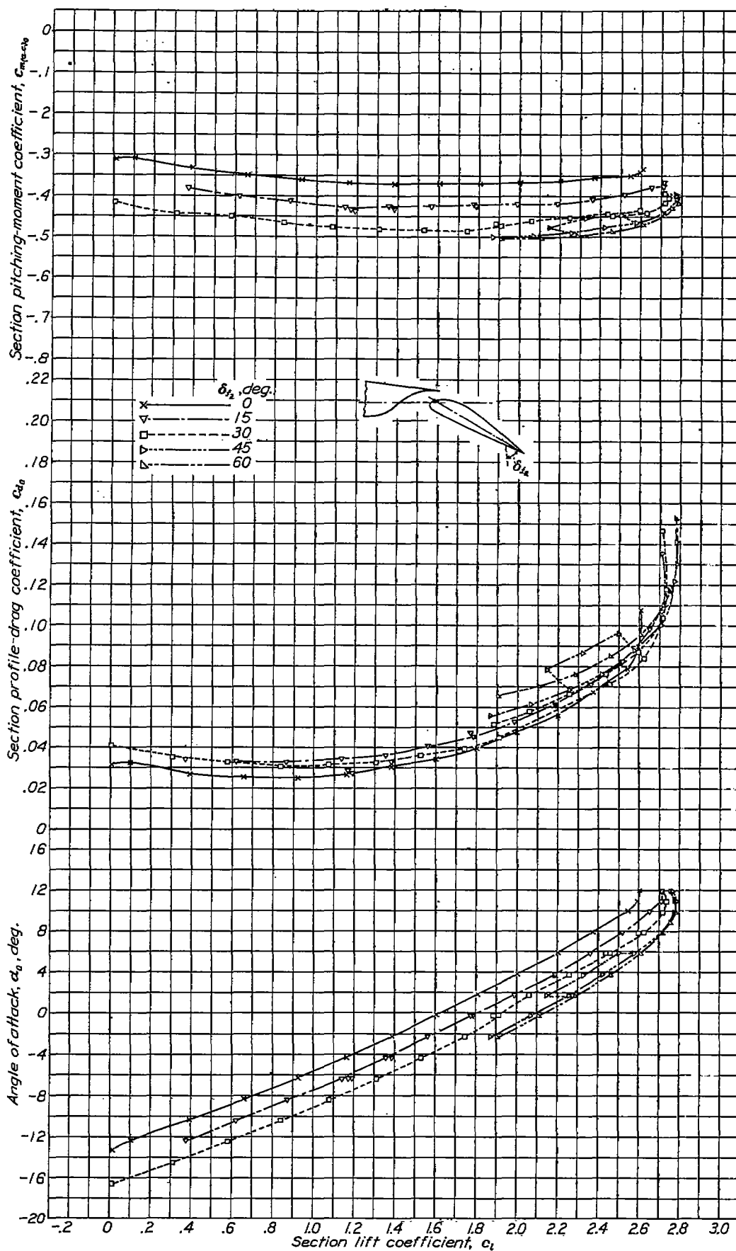
FIGURE 7.—Section characteristics of the N. A. C. A. 23012 airfoil with the main slotted flap deflected 30° and the auxiliary 0.05c s split flap deflected various amounts.
