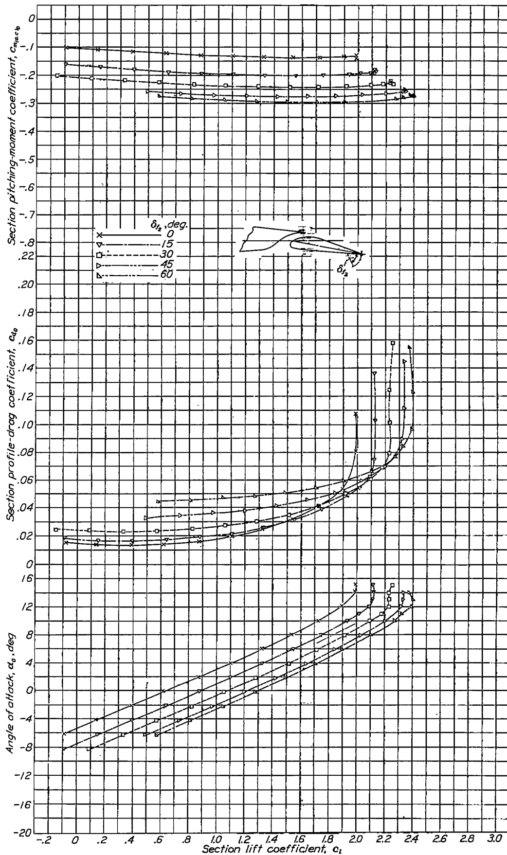
FIGURE 5.—Section characteristics of the N. A. C. A. 23012 airfoil with the main slotted flap deflected 10^\circ and the auxiliary 0.06% split flap deflected various amounts.
