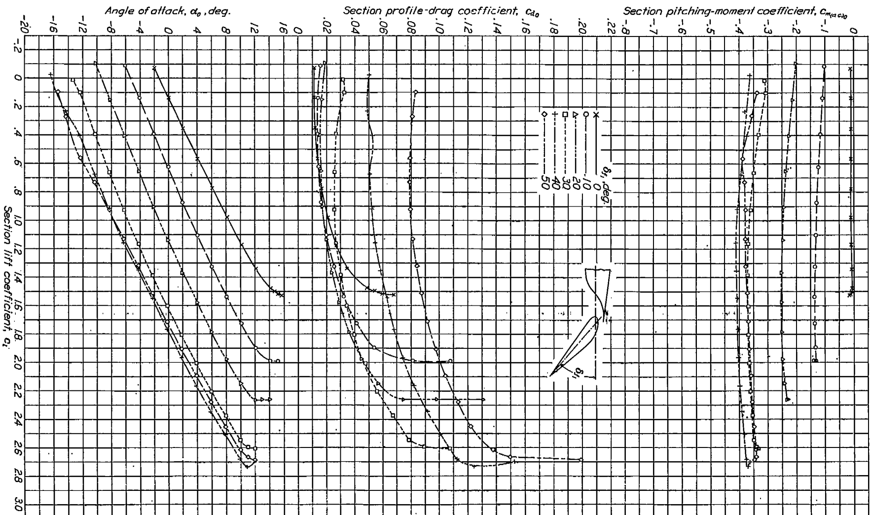
FIGURE 3.—Section characteristics of the N. A. C. A. 23012 airfoil with the main slotted flap deflected various amounts.
