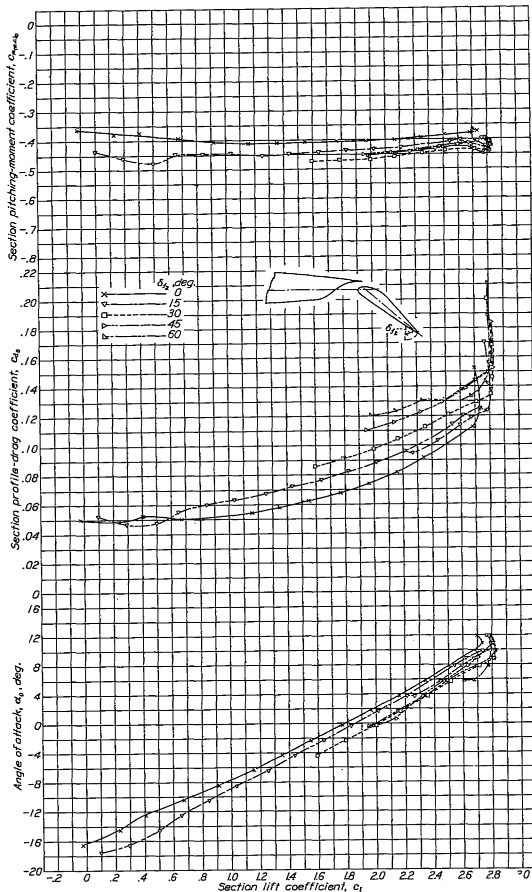
FIGURE 8.—Section characteristics of the N. A. C. A. 23012 airfoil with the main slotted flap deflected 40° and the auxiliary 0.05 c_u split flap deflected various amounts.
