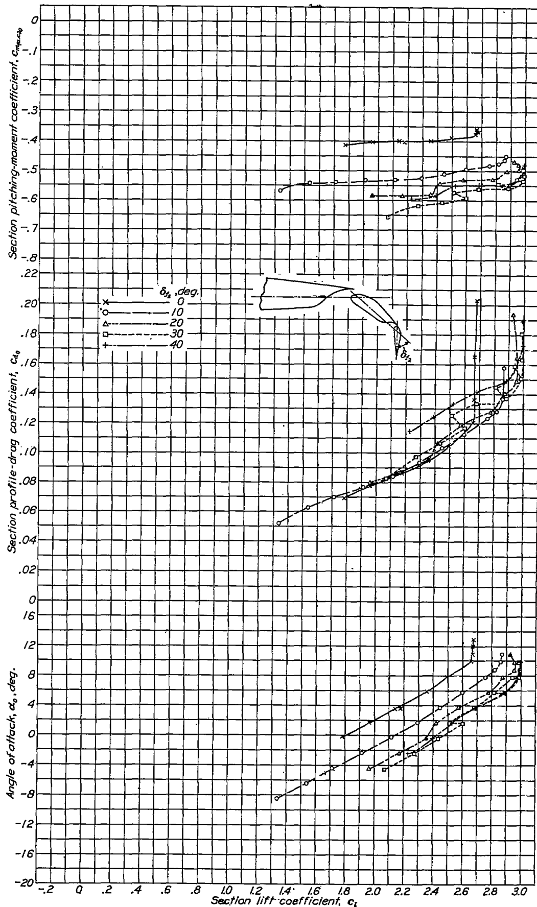
FIGURE 24—Section characteristics of the N. A. O. A. 23012 airfoil with the main slotted flap deflected 40^\circ and the auxiliary 0.10c slotted flap deflected various amounts.
