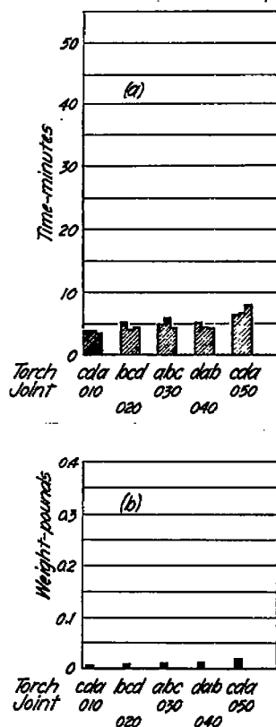
(a) Time required to weld butt joints. (b) Weights of weld metal in butt joints.
