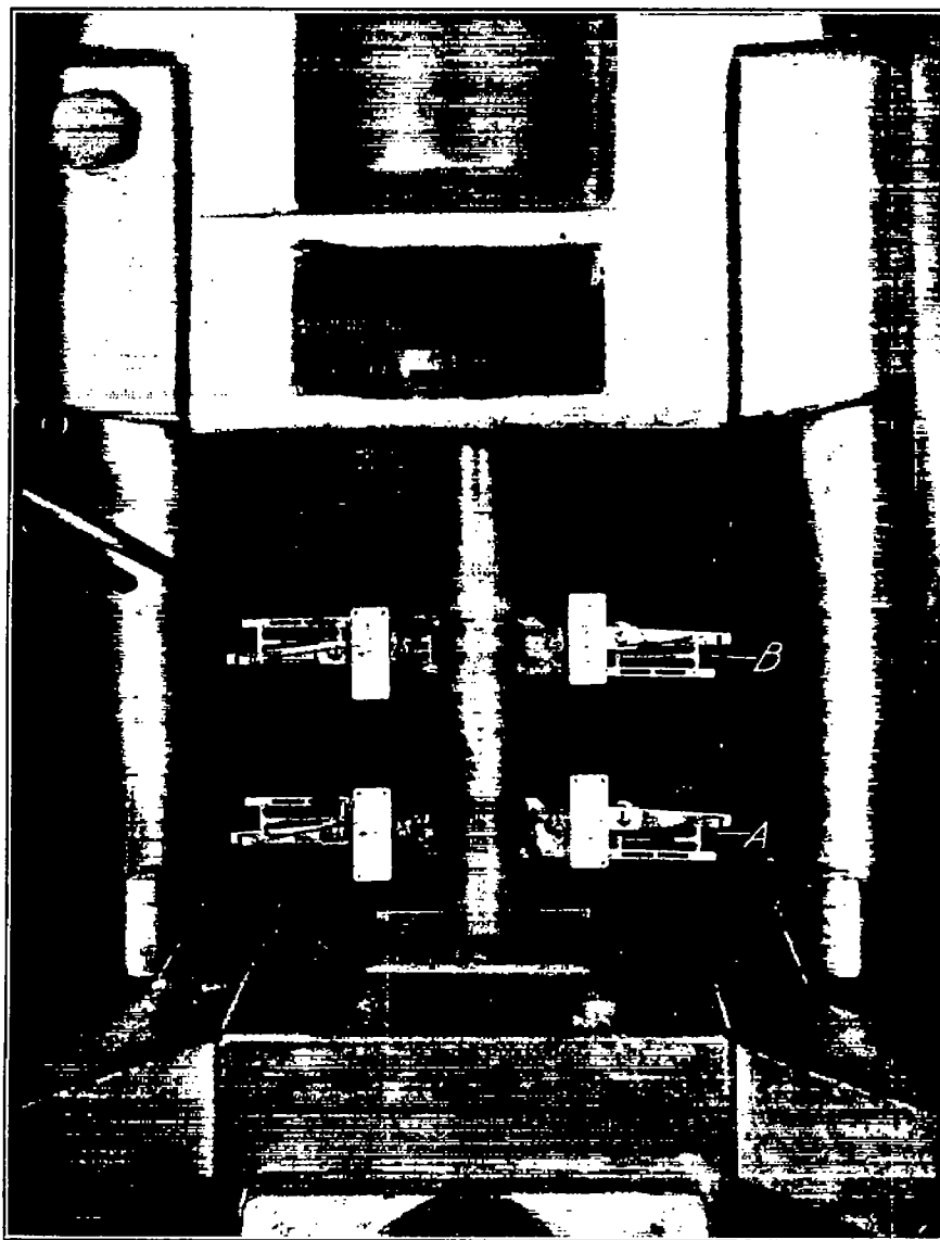
FIGURE 18.—Huggenberger extensometers on butt-joint to measure the strain near the weld and at a distance from the weld
