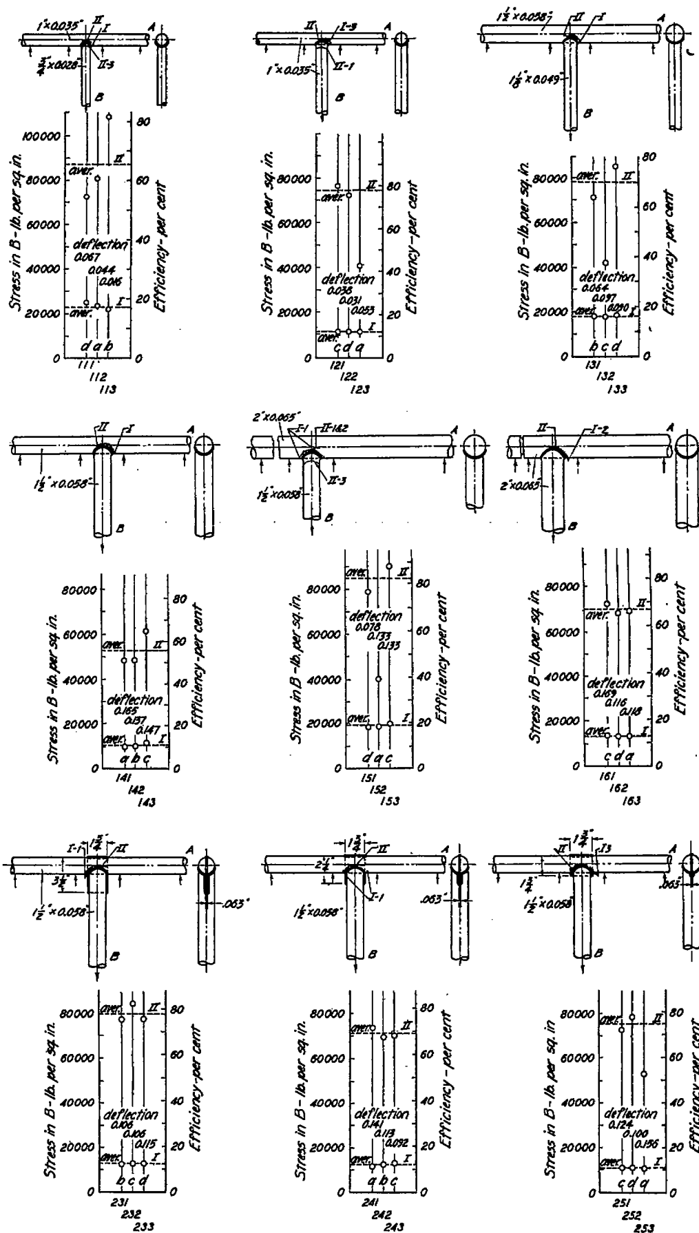
FIGURE 20.—Test results for T joints 110 to 280. Maximum stresses and efficiencies have been plotted on the same graph. For example, in joint 111, the maximum stress in loading I was 25,000 lb./in. 2 tension in tube B from the stress scale on the left side of the graph. The plotted points also indicate efficiency and on the right side, joint 111 is seen to have an efficiency of 18 per cent in loading I. The permanent deflection at midspan was 0.067 inch. In loading II the joint failed at a stress of 73,000 lb./in. 2 Its efficiency in loading II was 54 per cent
