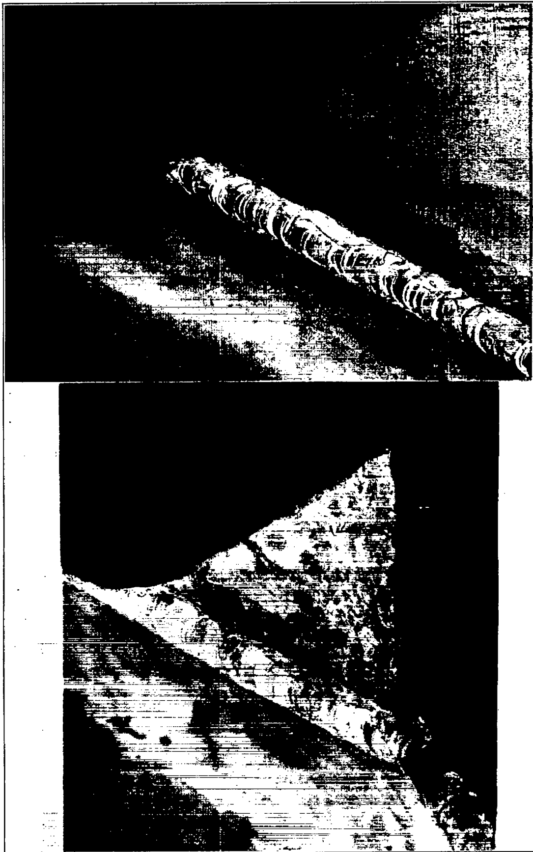
FIGURE 15.—Cracks produced by residual stresses in joints after cooling. Upper, in specimen 753; lower, in specimen 351.
