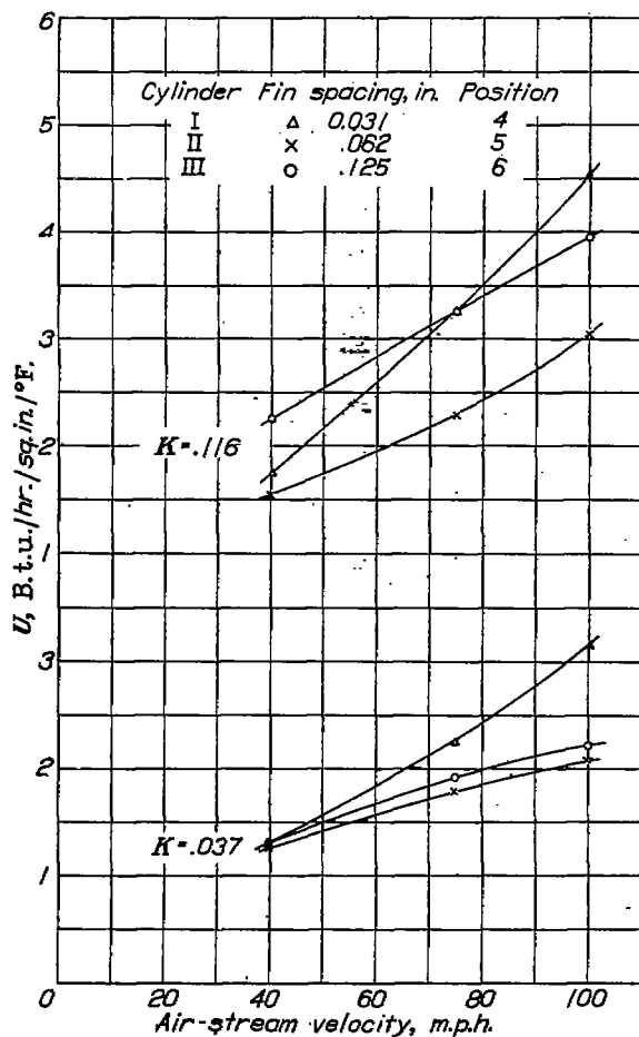
FIGURE 17.—Variation of average heat-transfer coefficient with air-stream velocity for three cylinders having \frac{1}{4} -inch fin width in positions 4, 5, and 6, with two engine conductivities. Cruising condition.
