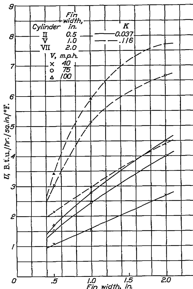
FIGURE 11.—Variation of average heat-transfer coefficient with fin width for three cylinders having \frac{1}{8} -inch fin spacing, for two engine conductivities and three air-stream velocities. All tests in position 2 with wooden cylinders in place. Cruising condition.
