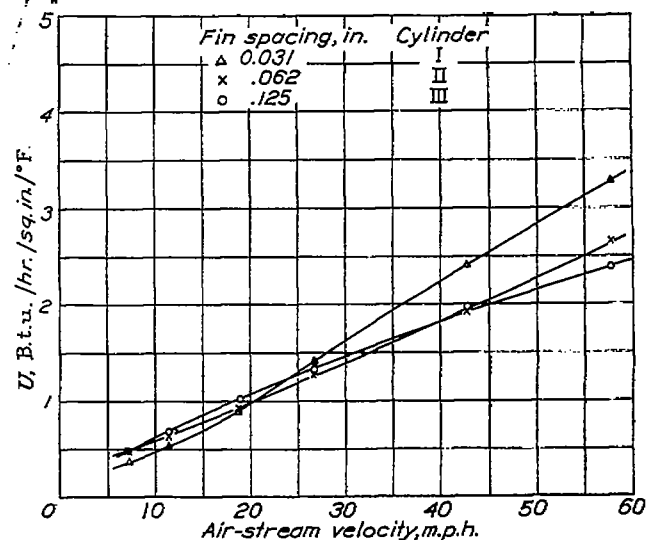
FIGURE 18.—Variation of average heat-transfer coefficient with air-stream velocity for three cylinders having \frac{1}{4} -inch fin width. Duct tests.
