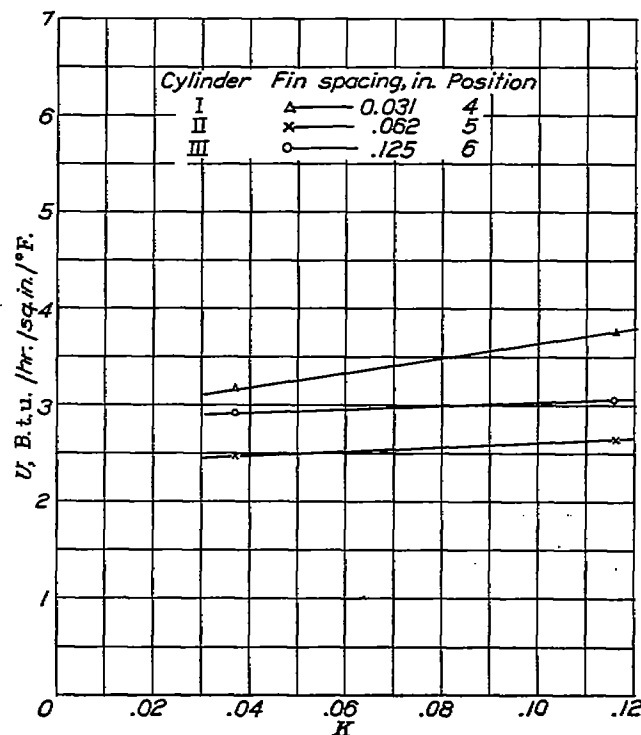
FIGURE 7.—Variation of average heat-transfer coefficient with engine conductivity for three cylinders having \frac{1}{4} -inch fin width tested in positions 4, 5, and 6. Ground run.
