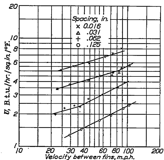
FIGURE 15.—Variation of average heat-transfer coefficient with velocity between the fins on the baffled part of the cylinder.
