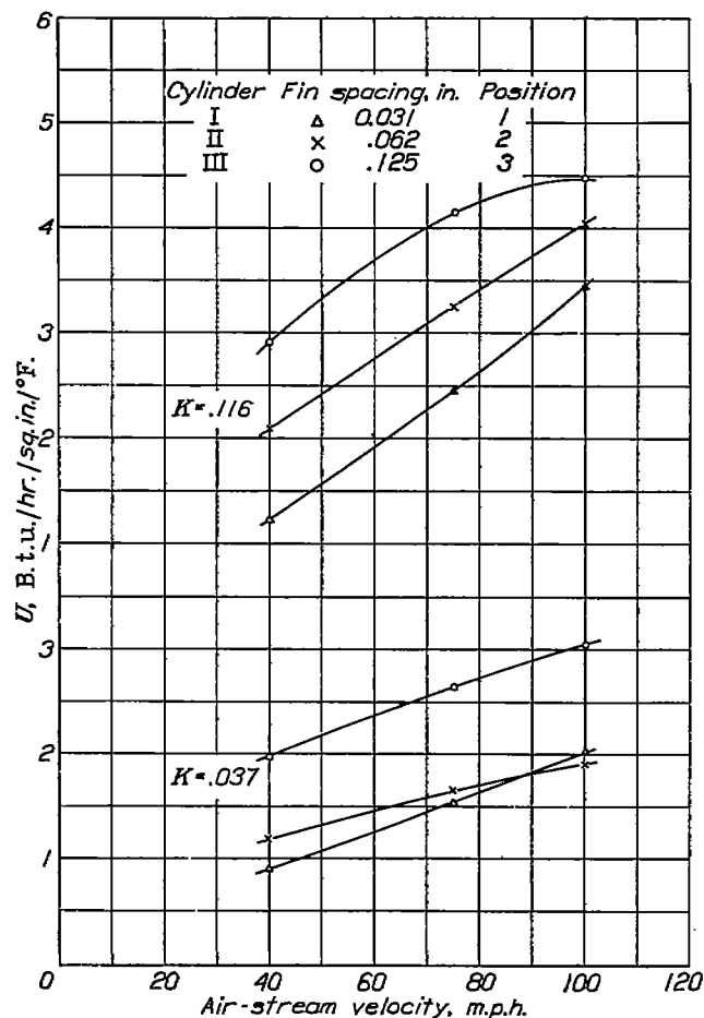
FIGURE 13.—Variation of average heat-transfer coefficient with air-stream velocity for three cylinders having 1/4-inch fin width in positions 1, 2, and 3 for two engine conductivities. Wooden cylinders in place. Cruising condition.
