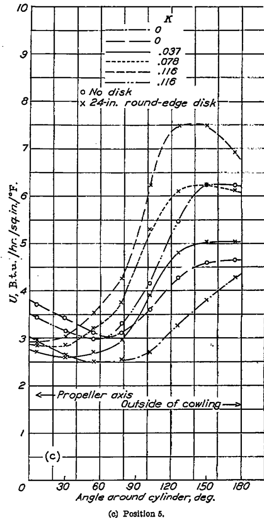
FIGURE 20.—Variation of local heat-transfer coefficient with angle around cylinder for cylinder V with \frac{1}{16} -inch fin spacing and 1-inch fin width for several engine conductivities, with and without disk in nose. Wooden cylinders. Ground condition.
