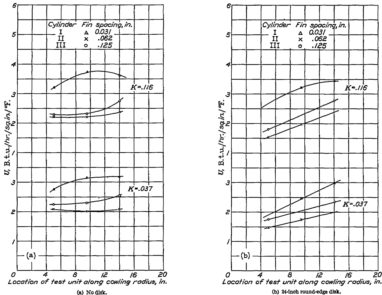
FIGURE 6.—Variation of average heat-transfer coefficient with location along the cowling radius for three cylinders having \frac{1}{4} -inch fin width tested in positions 1, 2, and 3. Ground run.
