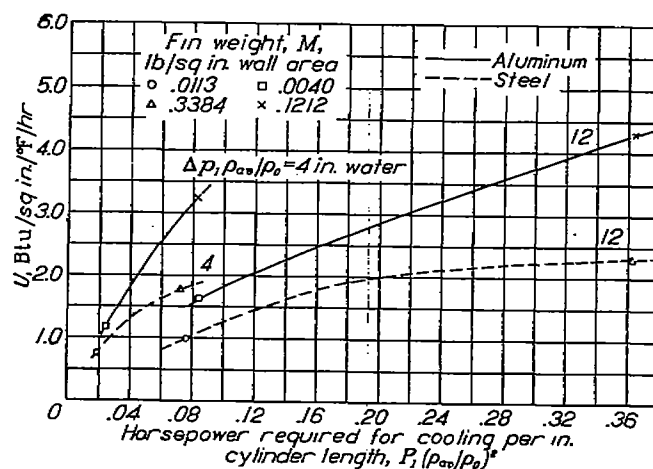
FIGURE 28.—Variation of maximum heat transfer with power required for cooling. Criterion, fin weight.
