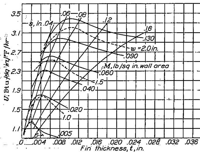
FIGURE 12.—Optimum dimensions for copper fins with specified fin space. Criterion, fin weight; \Delta p, \rho_{av}/\rho_o , 4 inches of water.
