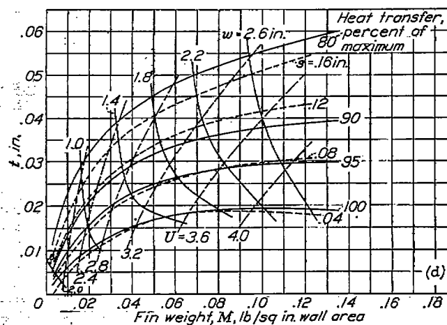
(d) Pressure difference \Delta p_{12} = p_1 - p_2 , 12 inches of water.
