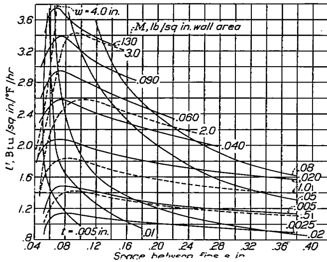
FIGURE 13.—Optimum dimensions for magnesium fins with specified fin thickness. Criterion, fin weight; \Delta p_{\text{max}}/\rho_{\text{air}} 4 inches of water.
