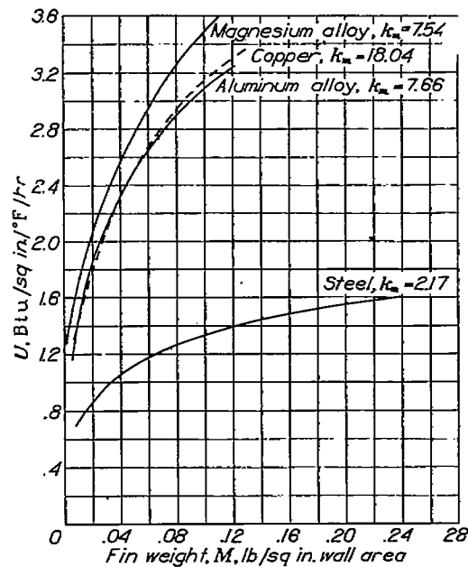
FIGURE 15.—Variation of maximum over-all heat-transfer coefficient with weight of fins for several fin materials. Criterion, fin weight; \Delta p_{\text{max}}/\rho_{\text{air}} 4 inches of water.
