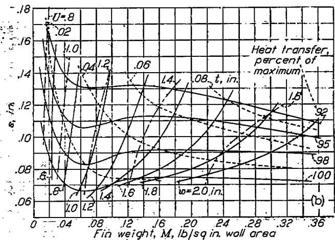
(b) Pressure difference \Delta p_{10} = \rho_0 , 4 inches of water.
