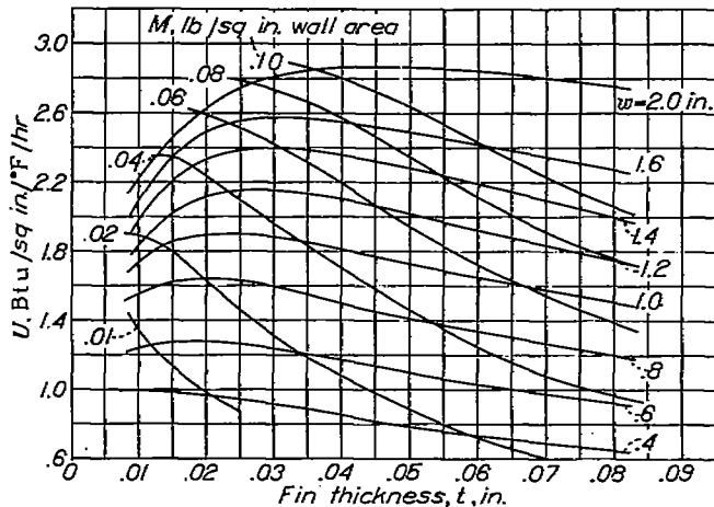
FIGURE 20.—Optimum dimensions for aluminum fins with specified fin width. Criterion, fin weight; \Delta p_{1p+1/p_0} 4 inches of water; optimum fin space constant at 0.072 inch.
