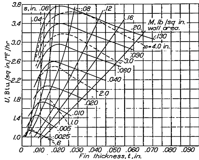
FIGURE 14.—Optimum dimensions for magnesium fins with specified fin space Criterion, fin weight; \Delta p_{\text{max}}/\rho_{\text{air}} 4 inches of water.
