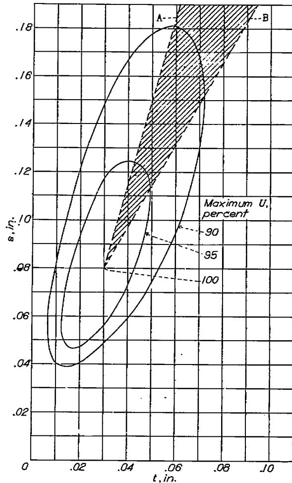
FIGURE 5.—Variation of s and t for several percentages of maximum heat-transfer coefficient. Constant M and \Delta p_{total} / \rho_a / \rho_o .
