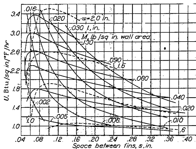
FIGURE 11.—Optimum dimensions for copper fins with specified fin thickness. Criterion, fin weight; \Delta p, \rho_{av}/\rho_o , 4 inches of water.
