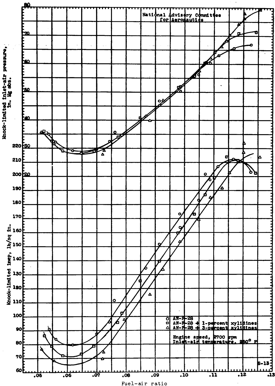
Figure 2. - Effect of addition of xylydines on knock-limited performance of AN-F-28 fuel in a 17.6 engine. Compression ratio, 7.0; engine speed, 2700 rpm; inlet-air temperature, 250° F; spark advance, 40° B.T.C.; inlet-coolant temperature, 250° F.
