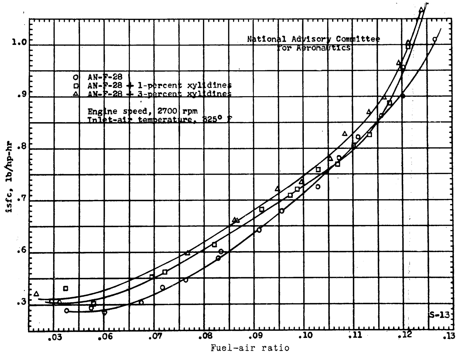
Figure 3. - Concluded. Effect of addition of xylidines on knock-limited performance of AN-F-28 fuel in a 17.6 engine. Compression ratio, 7.0; engine speed, 2700 rpm; inlet-air temperature, 325° F; spark advance, 40° B.T.C.; inlet-coolant temperature, 250° F.
