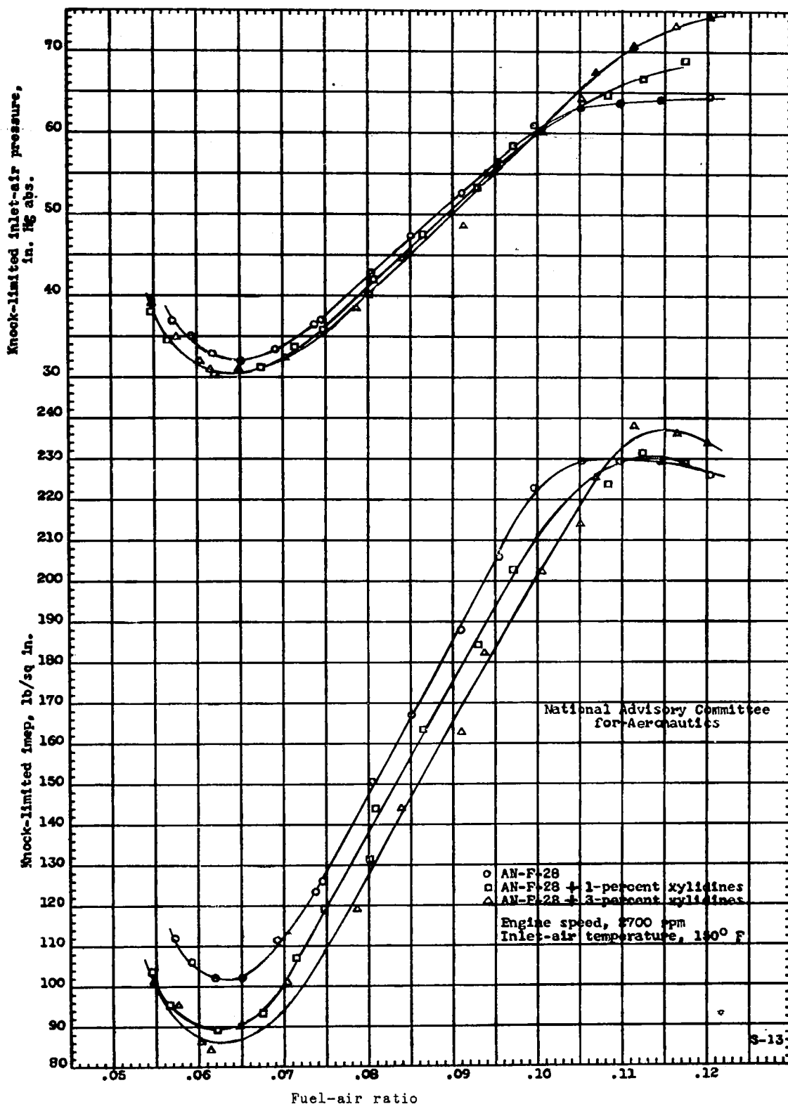
Figure 1. - Effect of addition of xyliidines on knock-limited performance of AN-F-28 fuel in a 17.6 engine. Compression ratio, 7.0; engine speed, 2700 rpm; inlet-air temperature, 150° F; spark advance, 40° B.T.C.; inlet-coolant temperature, 250° F.
