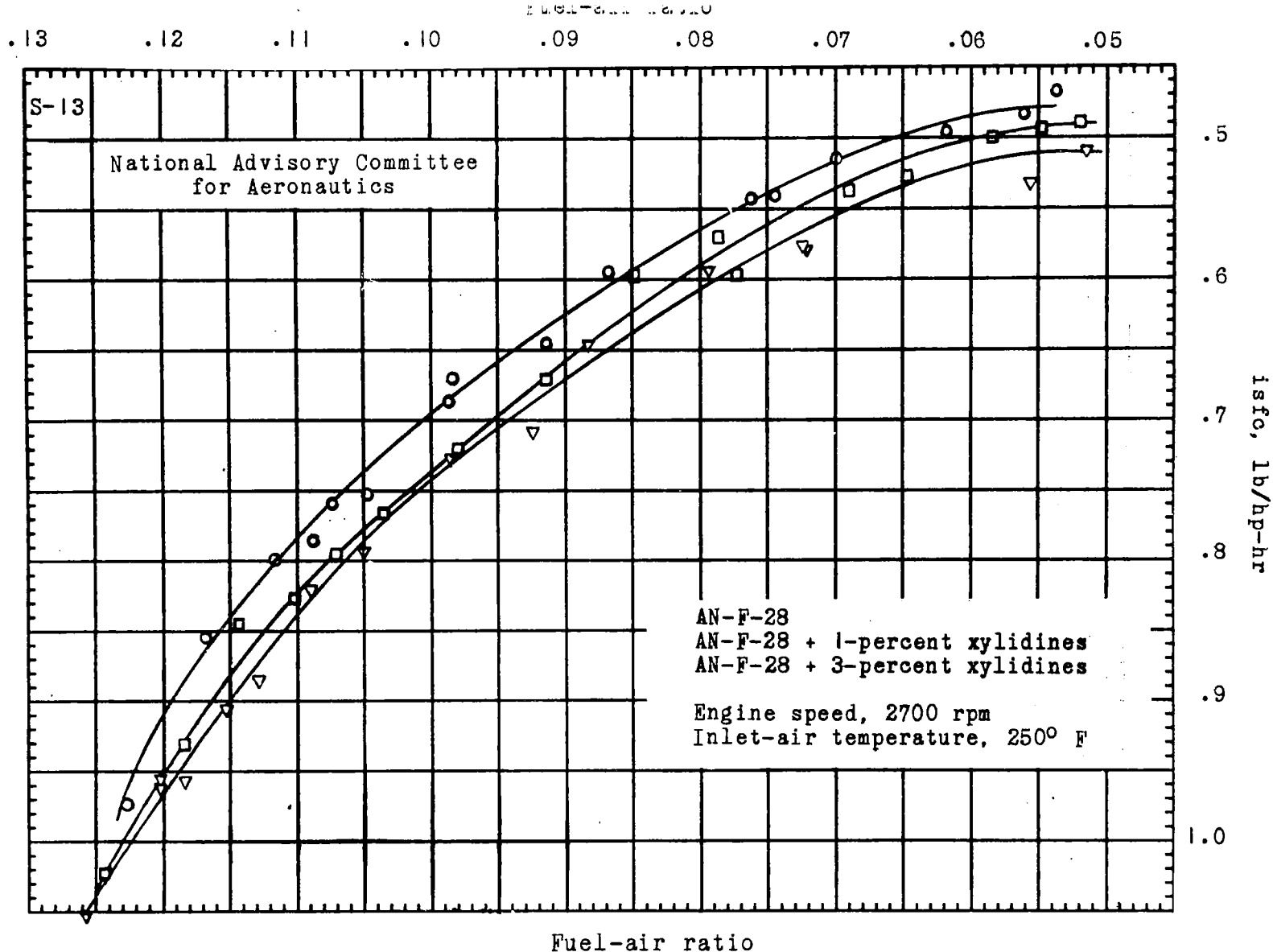
Figure 2. - Concluded. Effect of addition of xylidines on knock-limited performance of AN-F-28 fuel in a 17.6 engine. Compression ratio, 7.0; engine speed, 2700 rpm; inlet-air temperature, 250° F; spark advance, 40° B.T.C.; inlet-coolant temperature, 250° F.
