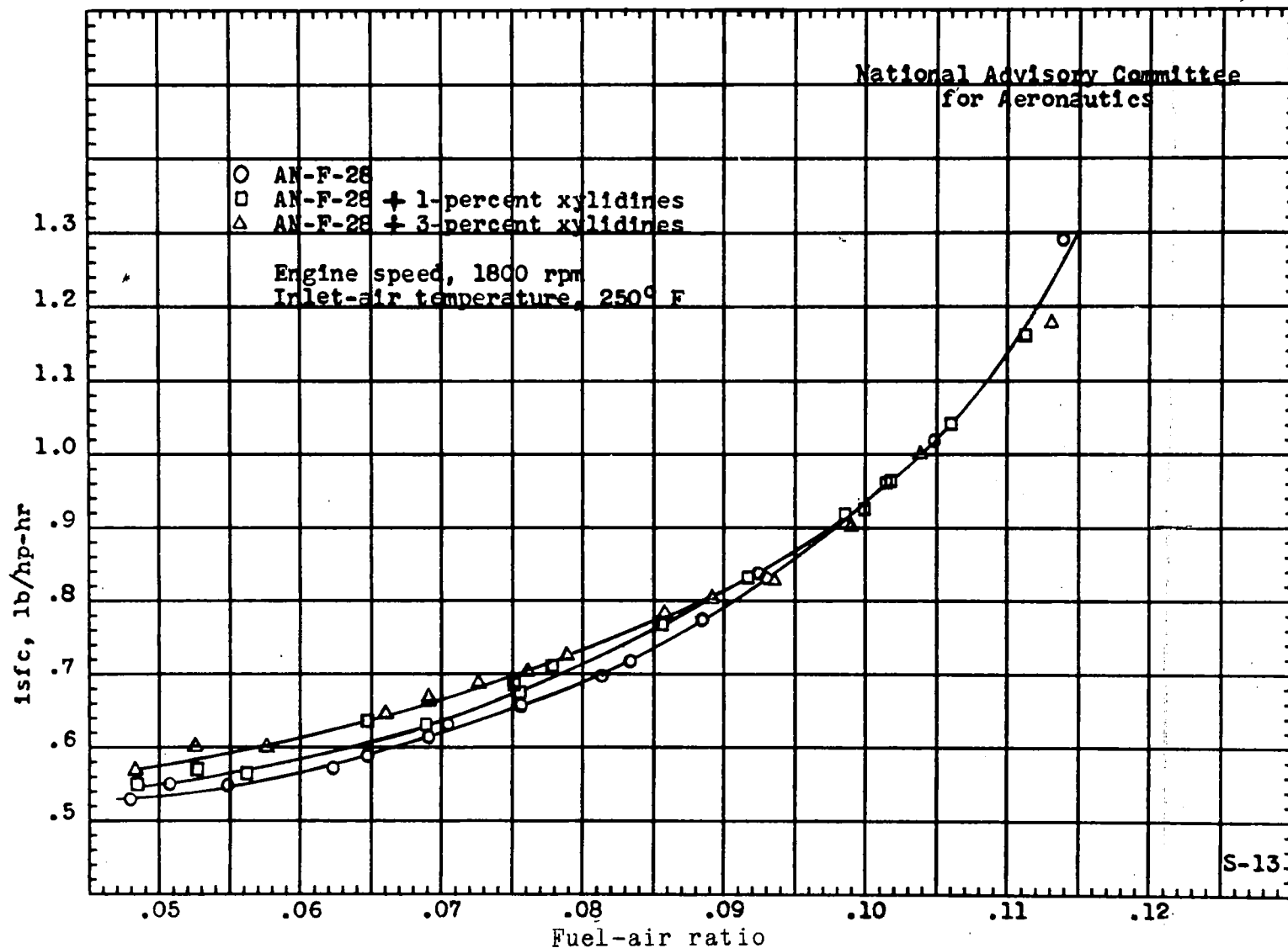
Figure 4. - Concluded. Effect of addition of xylidines on knock-limited performance of AN-F-28 fuel in a 17.6 engine. Compression ratio, 7.0; engine speed, 1800 rpm; inlet-air temperature, 250° F; spark advance, 40° B.T.C.; inlet-coolant temperature, 250° F.
