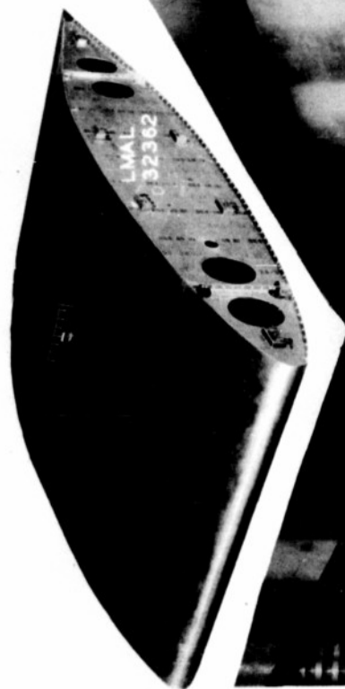
Figure 11.- Test of low-drag wing specimen with load applied through spars.
