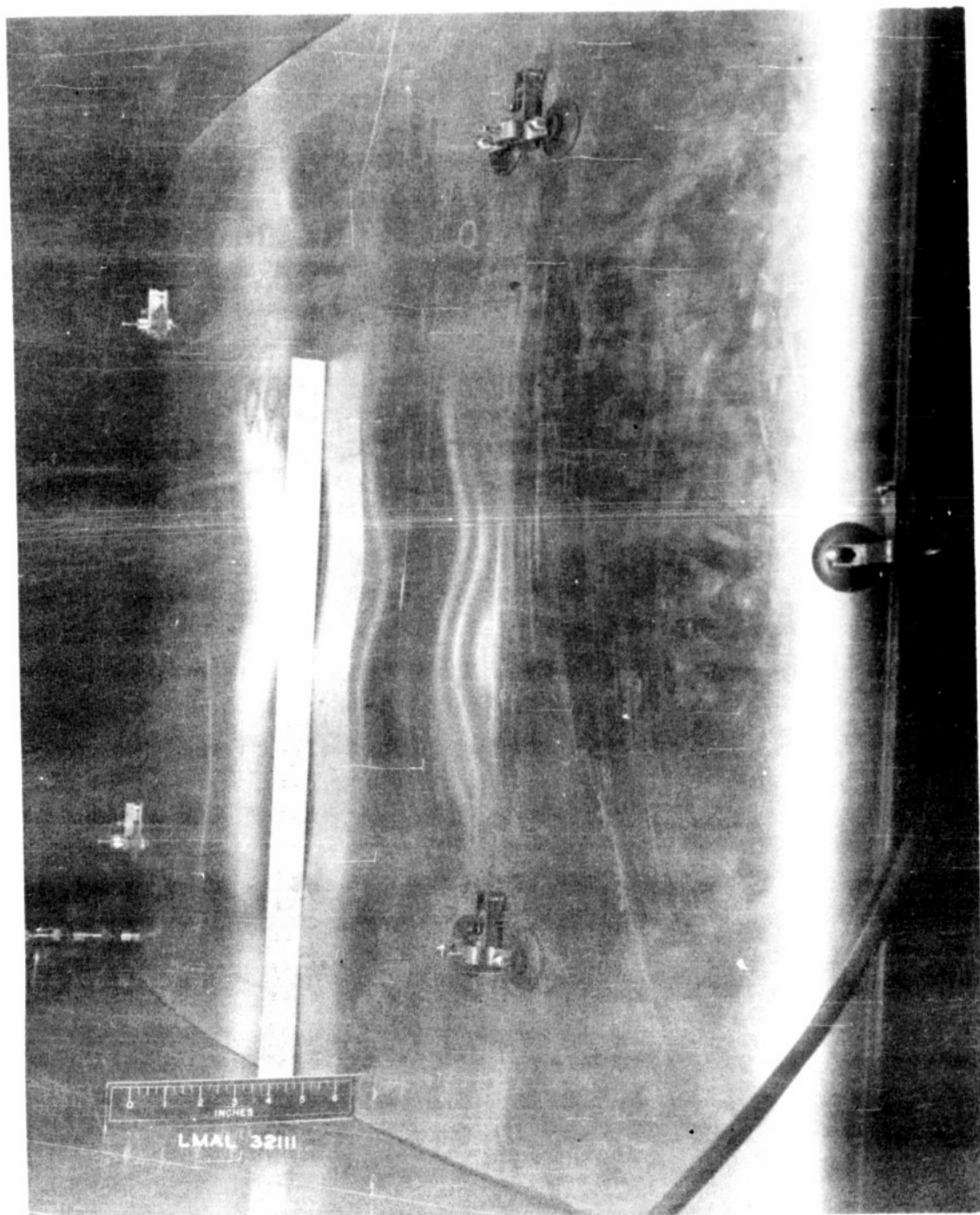
Figure 7.- Buckles in low-drag wing specimen at load of 85,000 pounds.
