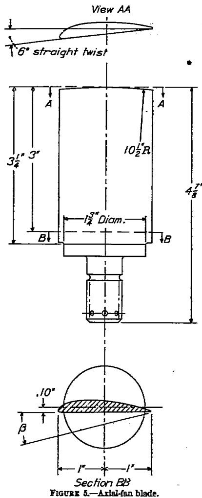
FIGURE 6.—Axial-fan blade.
