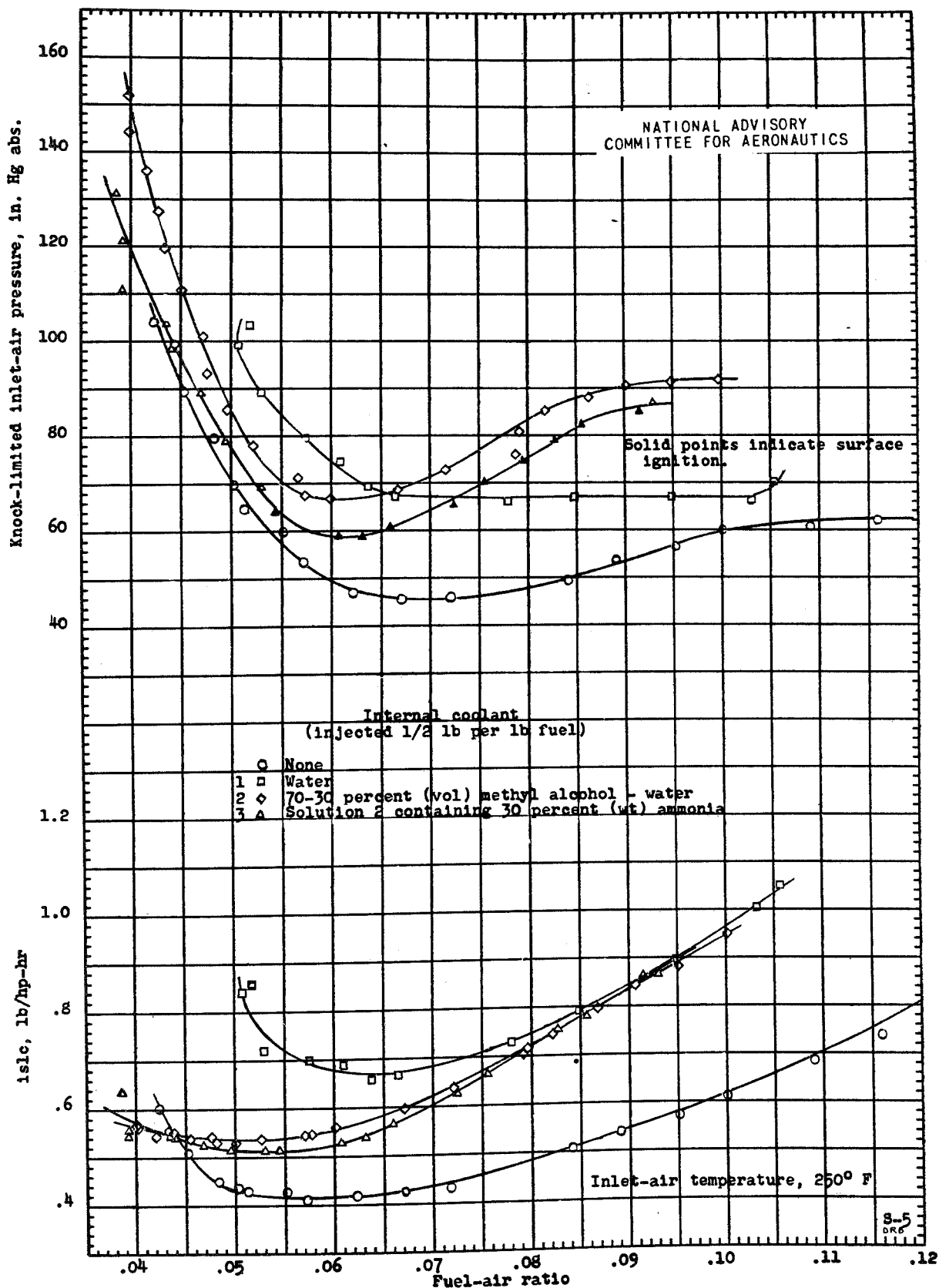
(b) Variation of indicated specific liquid consumption and knock-limited inlet-air pressure with fuel-air ratio at 250° F inlet-air temperature. Figure 5. - Continued. Effect of internal coolants 1, 2, and 3 on knock-limited engine performance. CFR engine; fuel, AN-F-28 fuel; compression ratio, 7.0; inlet-coolant temperature, 250° F; spark advance, 30° B.T.C.; engine speed, 2500 rpm.
