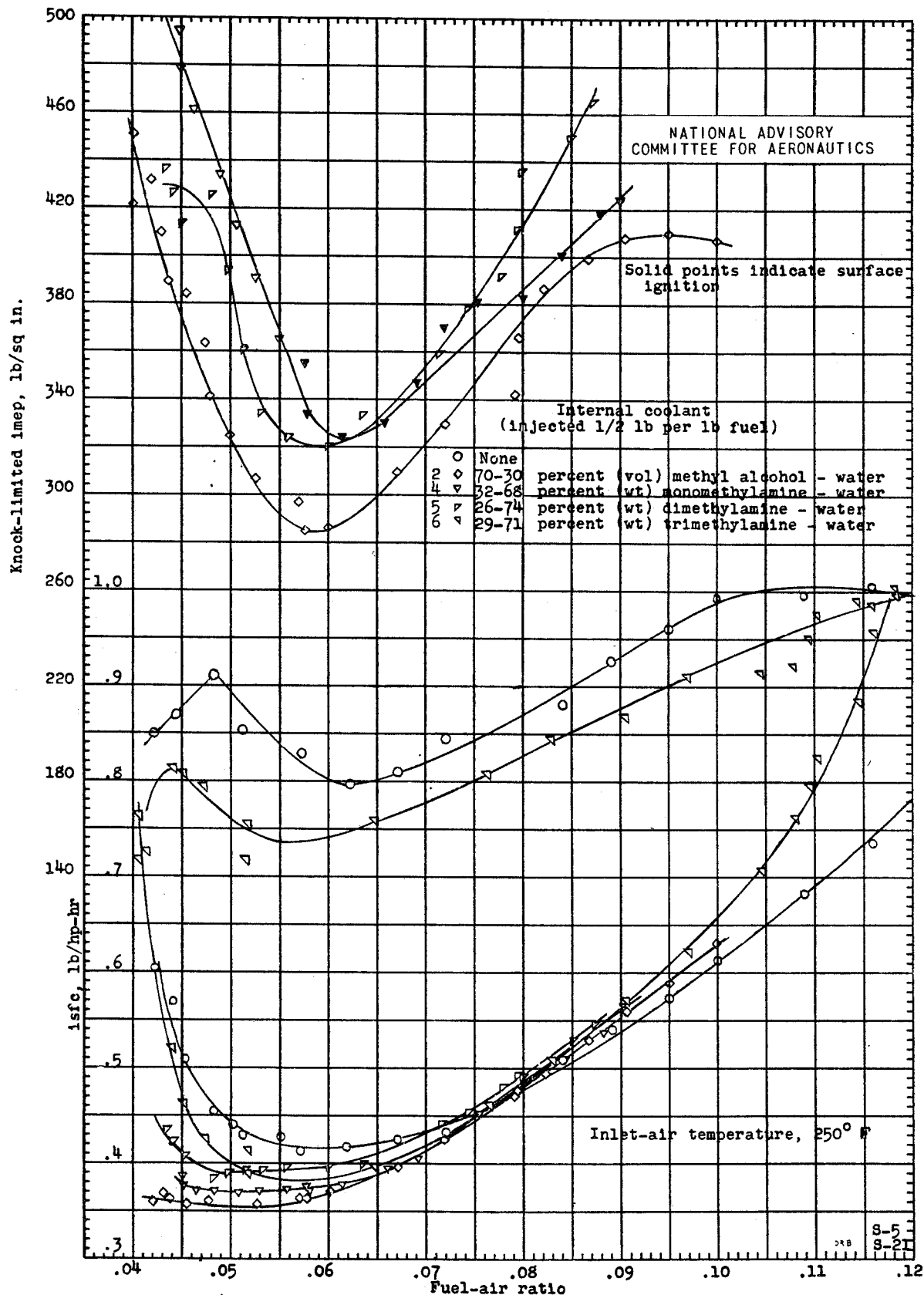
(a) Variation of indicated specific fuel consumption and knock-limited indicated mean effective pressure with fuel-air ratio at 250° F inlet-air temperature.
