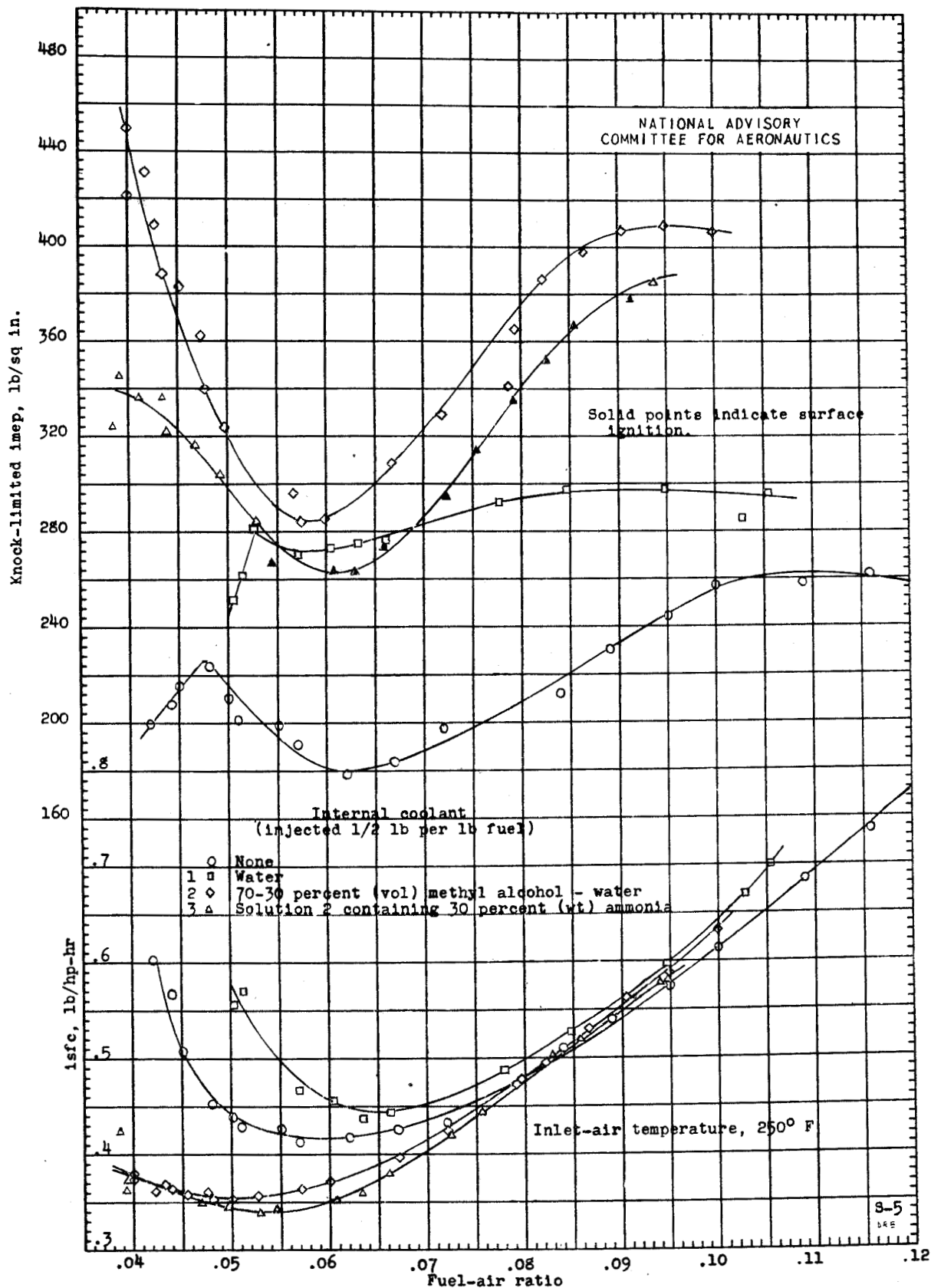
(a) Variation of indicated specific fuel consumption and knock-limited indicated mean effective pressure with fuel-air ratio at 250° F inlet-air temperature.
