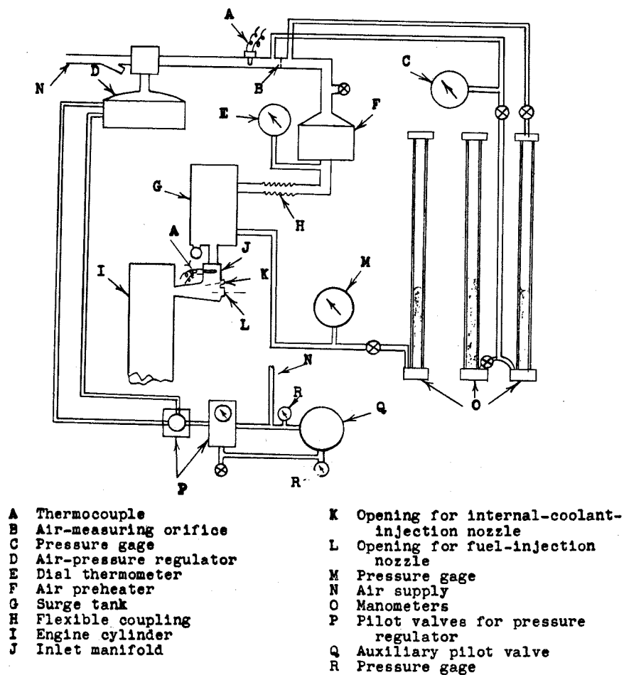
Figure 2. - Diagram of inlet-air system.
