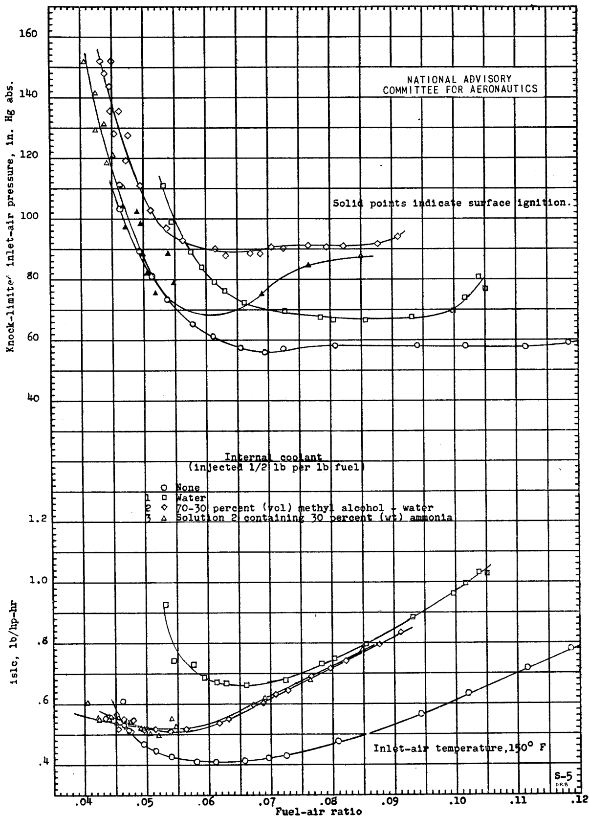
(d) Variation of indicated specific liquid consumption and knock-limited inlet-air pressure with fuel-air ratio at 150° F inlet-air temperature. Figure 5. - Concluded. Effect of internal coolants 1, 2, and 3 on knock-limited engine performance. CFR engine; fuel, AN-F-28 fuel; compression ratio, 7.0; inlet-coolant temperature, 250° F; spark advance, 30° B.T.C.; engine speed, 2500 rpm.
