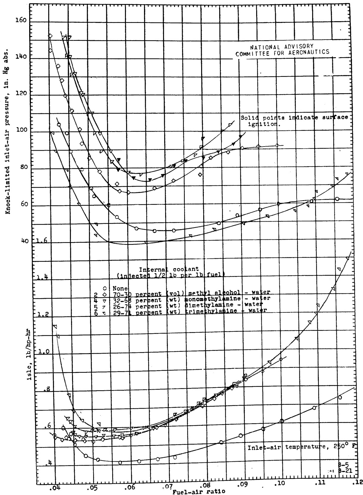
(b) Variation of indicated specific liquid consumption and knock-limited inlet-air pressure with fuel-air ratio at 250° F inlet-air temperature. Figure 6. - Continued. Effect of internal coolants 2, 4, 5, and 6 on knock-limited engine performance. CFR engine; fuel, AN-F-28 fuel; compression ratio, 7.0; inlet-coolant temperature, 250° F; spark advance, 30° B.T.C.; engine speed, 2500 rpm.
