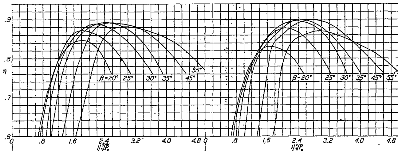
FIGURE 28.—Curves of propulsive efficiency against 1/\sqrt{P_c} for propeller C on nose 4. FIGURE 29.—Curves of propulsive efficiency against 1/\sqrt{P_c} for propeller C1 on nose 4.
