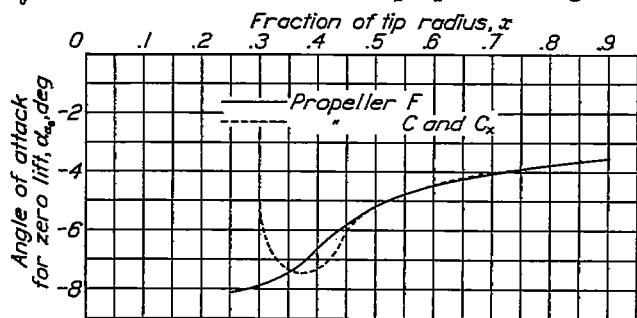
FIGURE 44.—Angle of zero lift.
