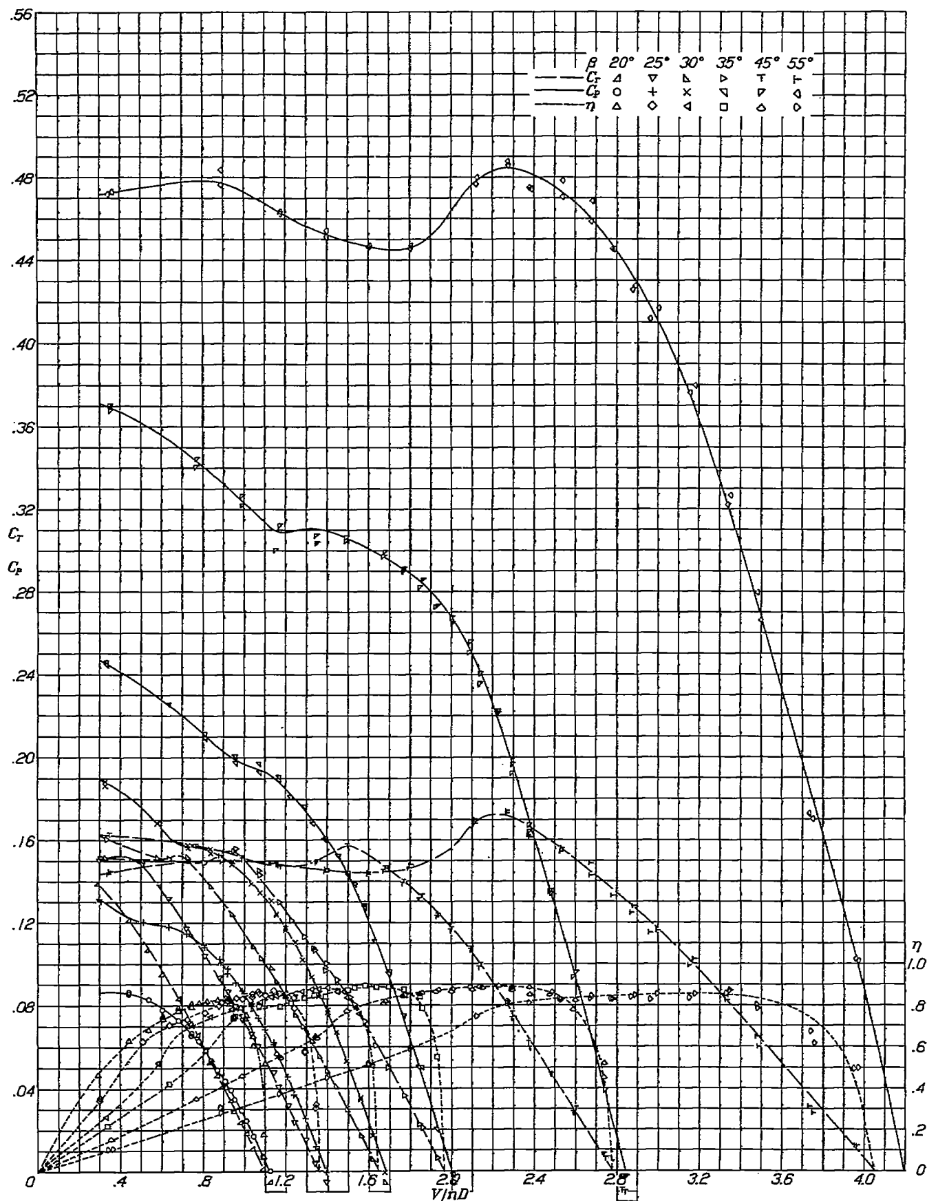
FIGURE 18.—Curves of C_T , C_P , and \eta against V/\pi D for propeller C_2 on nose 5 with splaner 1.
