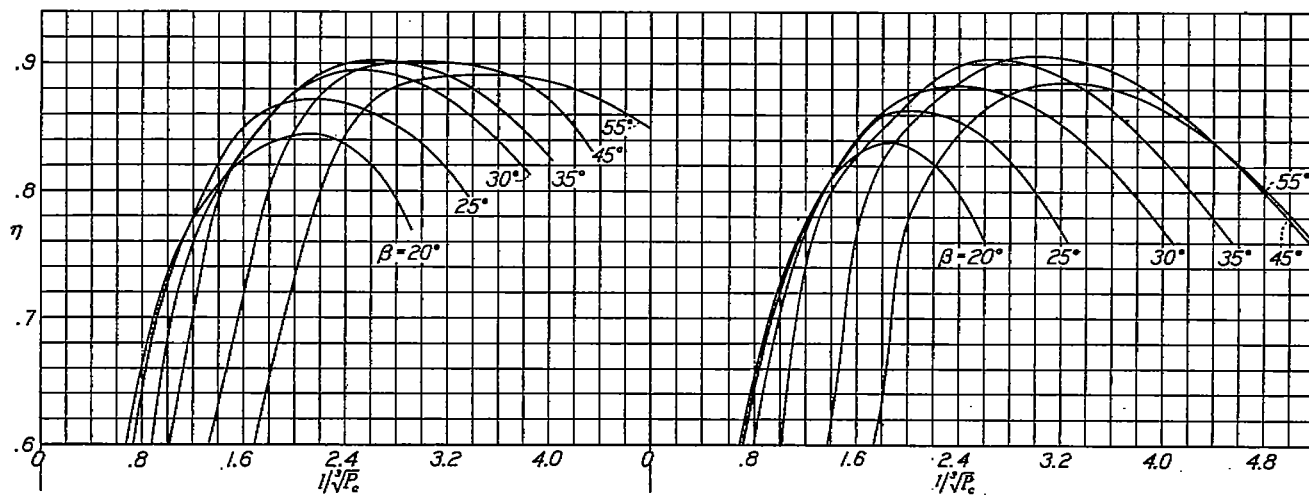
FIGURE 26.—Curves of propulsive efficiency against 1/\sqrt{P_e} for propeller O on nose 3 with spinner 1.
