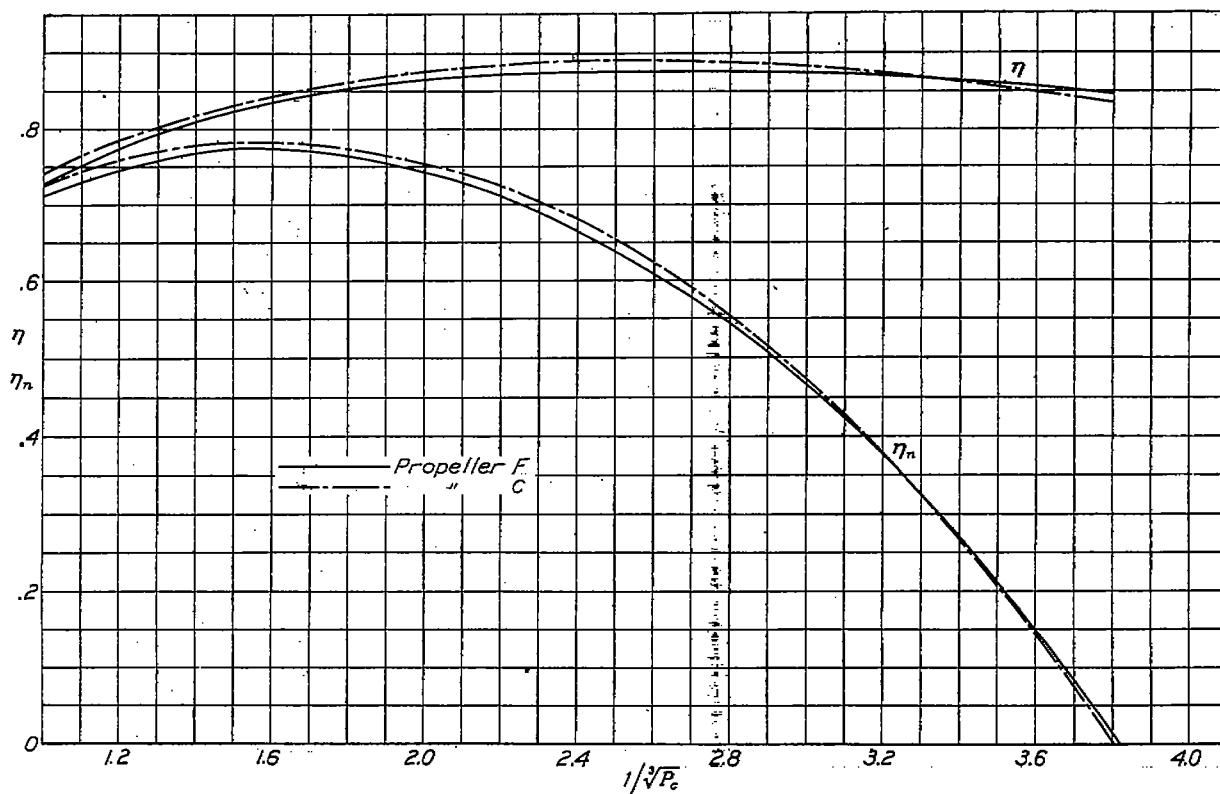
FIGURE 36.—Propulsive-efficiency and net-efficiency envelopes against 1/\sqrt{P_0} for propellers F and C on nose 1.
