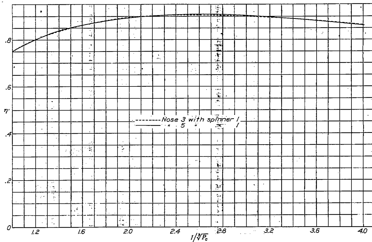
FIGURE 35.—Propulsive-efficiency envelopes against 1/\sqrt{P_0} for propeller F on noses 3 and 5. (Spinner is considered as part of body.)
