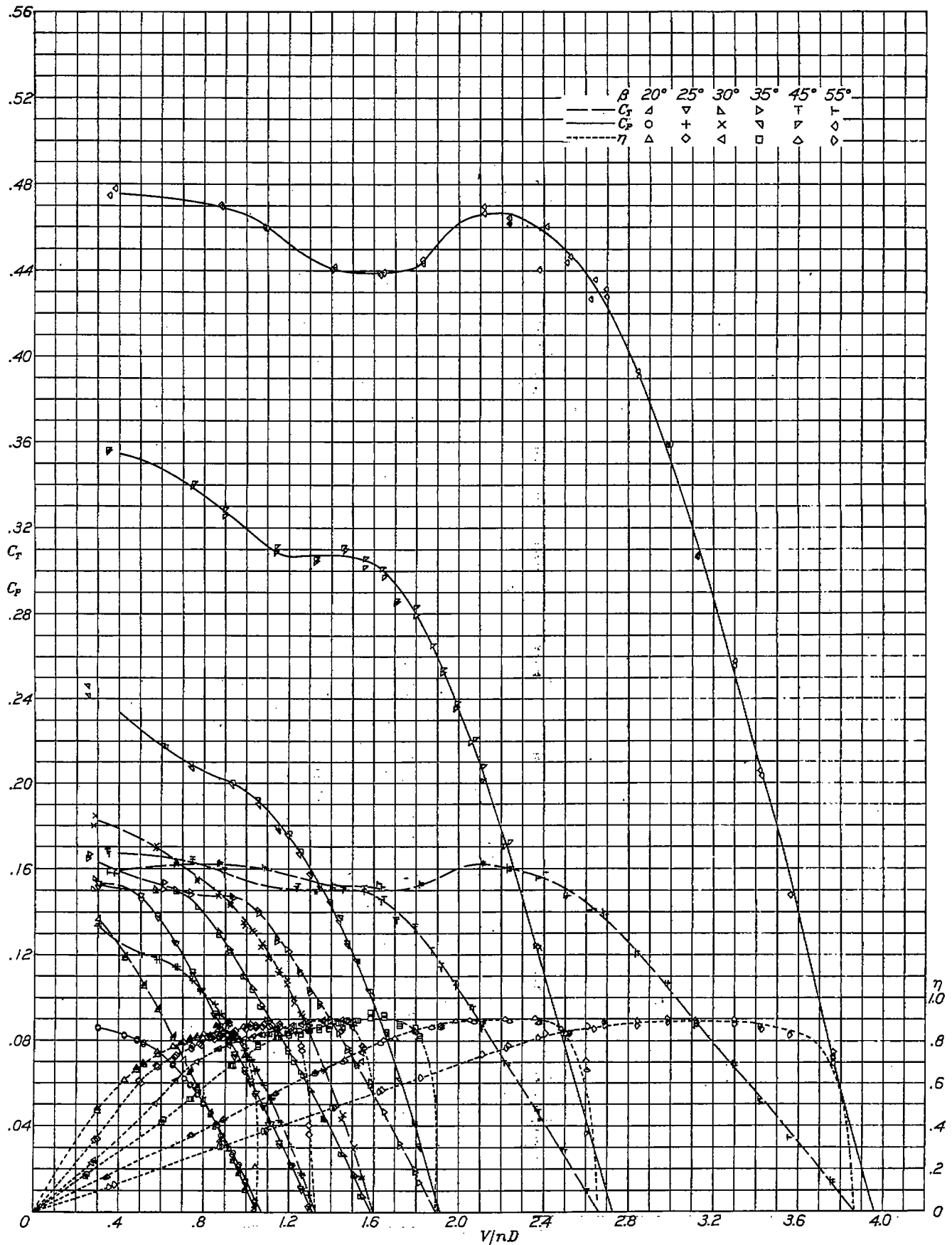
FIGURE 11.—Curves of C_r , C_p , and \eta against V/nD for propeller C on nose 3 with spinner 1.
