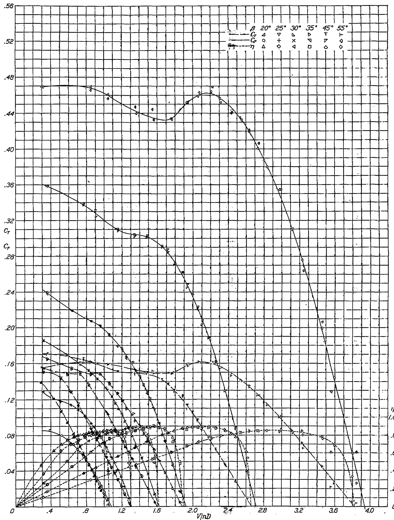
FIGURE 17.—Curves of C_T , C_P , and \eta against V/nD for propeller C on nose 5 with spinner 1.
