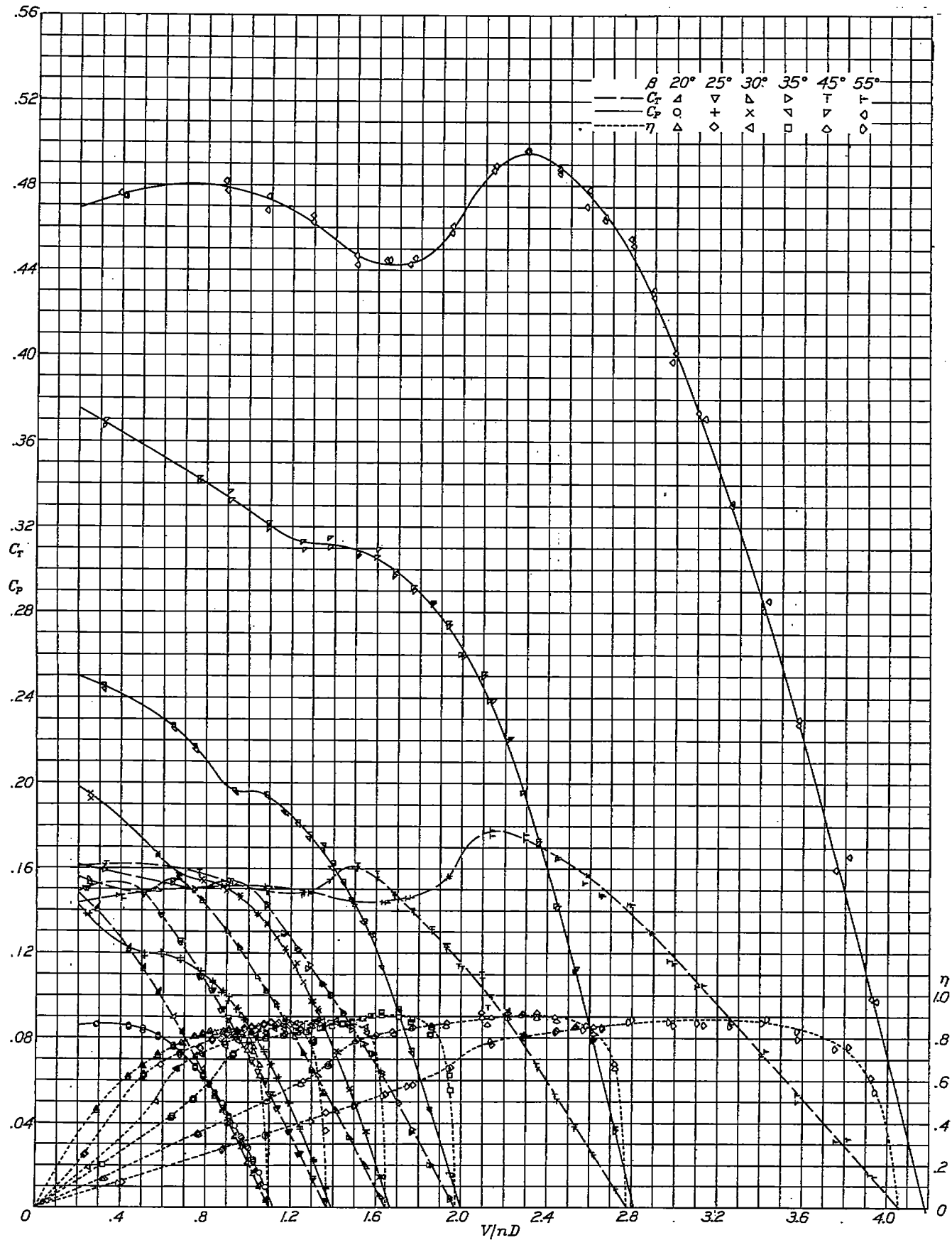
FIGURE 12.—Curves of C_T , C_P , and \eta against V/nD for propeller C_2 on nose 3 with spinner 1.
