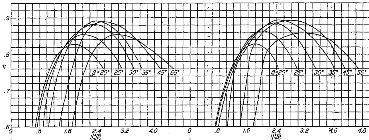
FIGURE 32.—Curves of propulsive efficiency against 1/\sqrt{P_c} for propeller C on nose 5 with spinner 1. FIGURE 33.—Curves of propulsive efficiency against 1/\sqrt{P_c} for propeller C1 on nose 5 with spinner 1.
