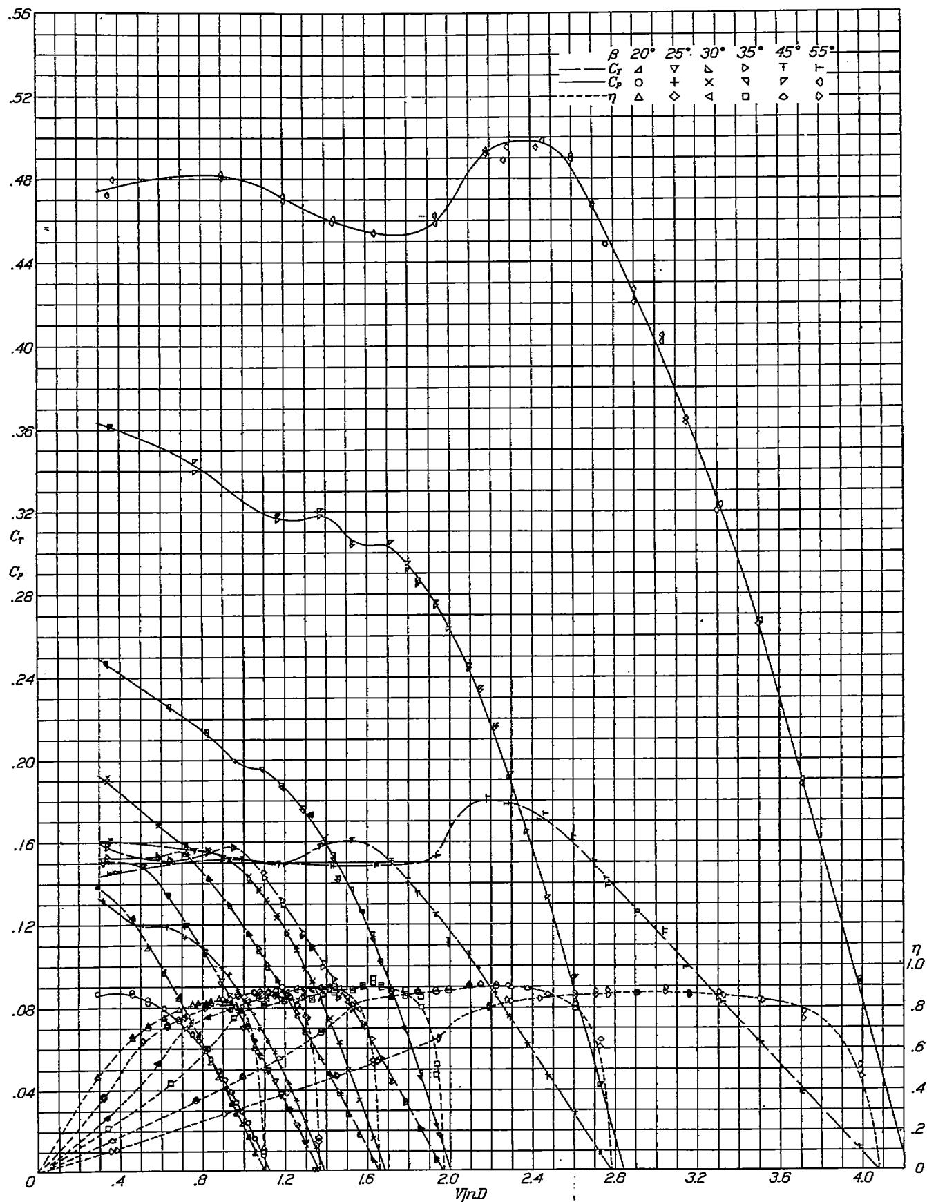
FIGURE 14.—Curves of C_T , C_P , and \eta against V/nD for propeller C_2 on nose 4.
