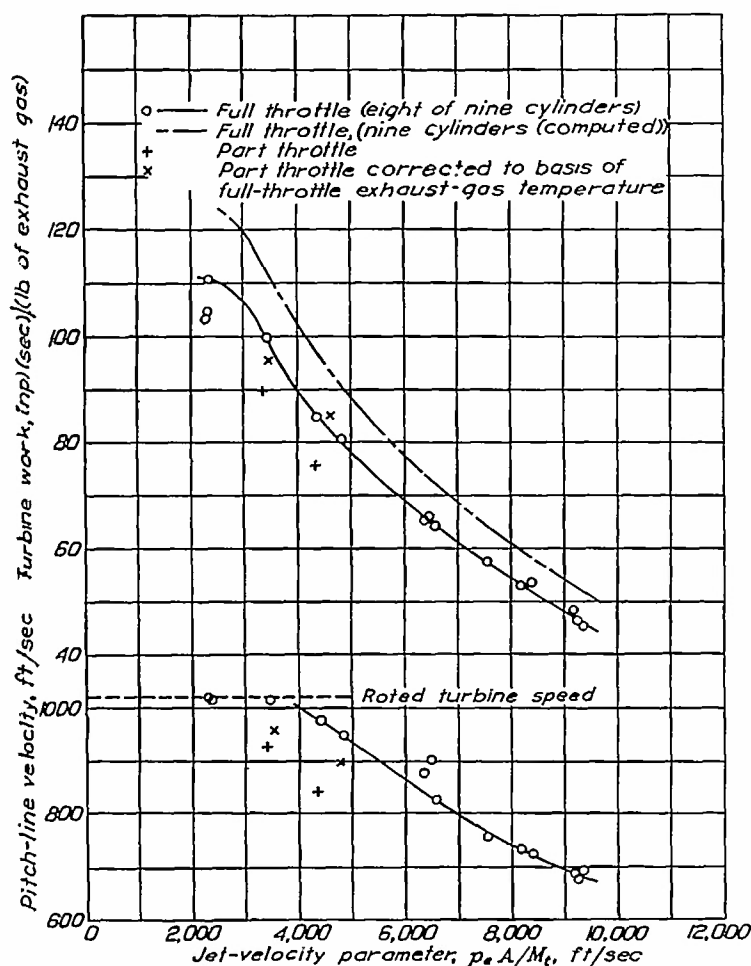
FIGURE 8.—Variation of maximum turbine work output per pound of exhaust gas and optimum turbine speed with jet-velocity parameter p_e A/M_t . Engine speed, 2000 rpm.
