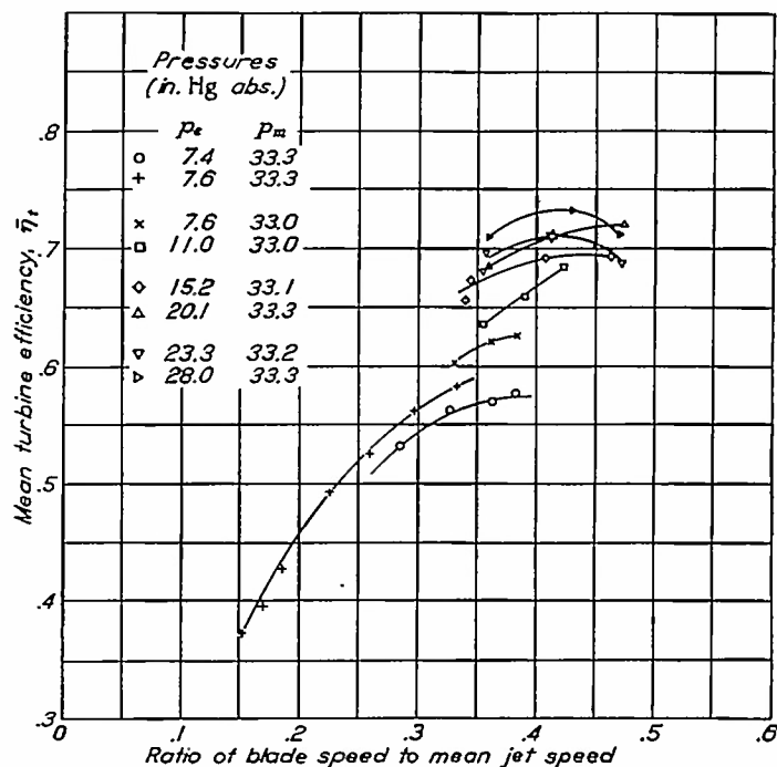
FIGURE 6.—Variation of mean turbine efficiency with ratio of blade speed to mean jet speed. Engine speed, 2000 rpm; full throttle.
