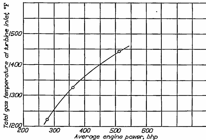
FIGURE 10.—Effect of engine power on exhaust-gas temperature. Engine speed, 2000 rpm; fuel-air ratio, 0.075.
