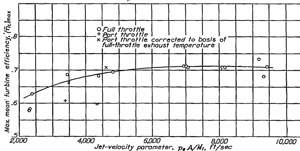
FIGURE 7.—Variation of maximum mean turbine efficiency with jet-velocity parameter p_e A/M_t .
