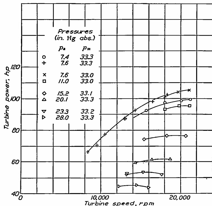
FIGURE 5.—Variation of turbine power with turbine speed. Engine speed, 2000 rpm; full throttle.
