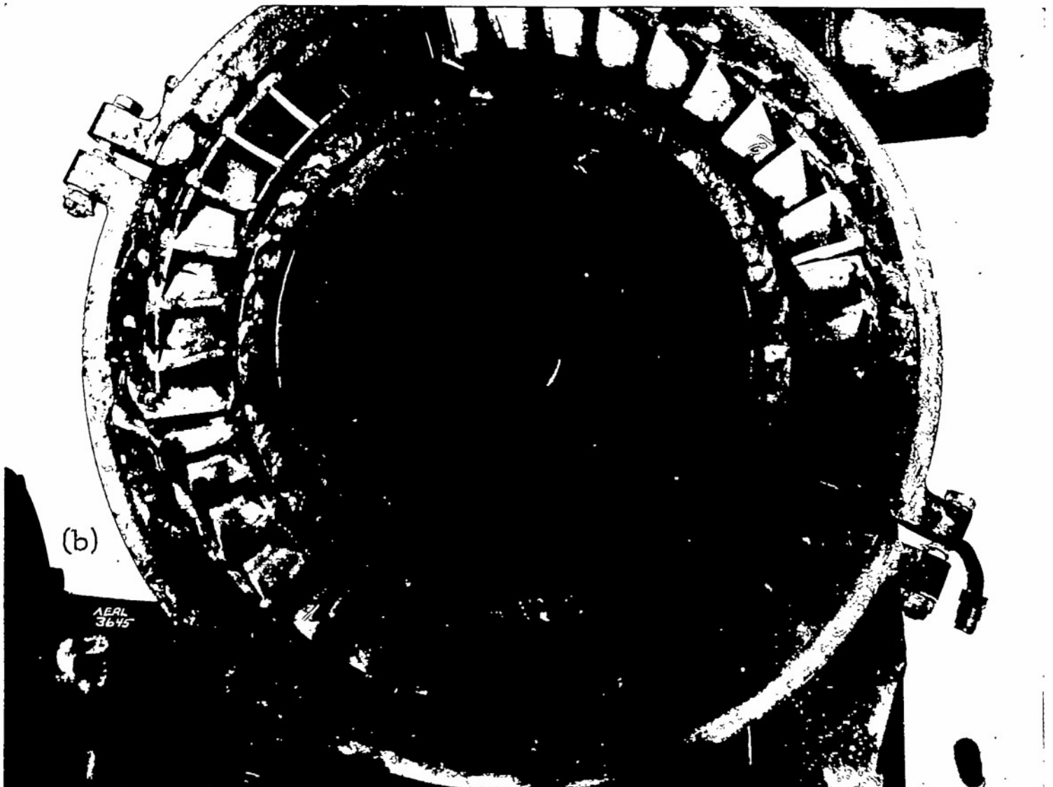
(b) Diaphragm assembly of four nozzle boxes.
