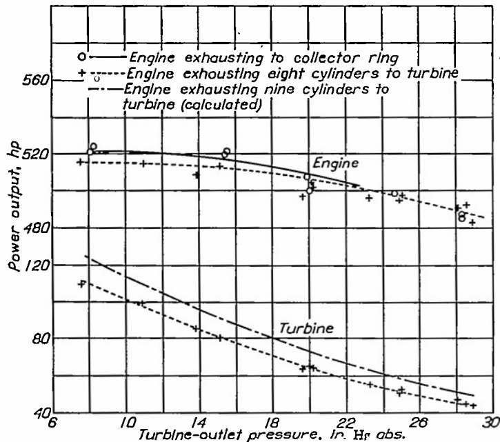
FIGURE 4.—Power output of engine and blowdown turbine. Engine speed, 2000 rpm. Data corrected to carburetor-air temperature of 90° F and inlet-manifold pressure of 33.5 inches of mercury absolute.
