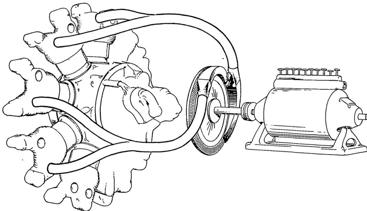
FIGURE 1.—Diagrammatic drawing of blowdown turbine for nine-cylinder radial engine with dynamometer load showing two of four nozzle boxes.
