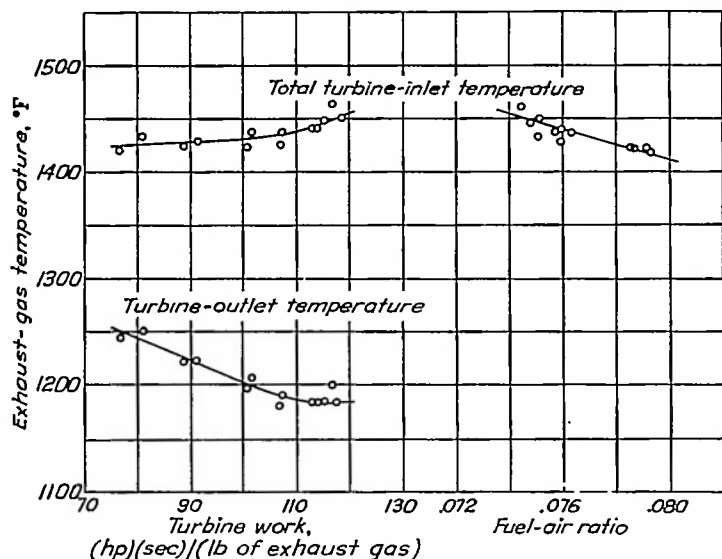
FIGURE 9.—Variation of exhaust-gas temperature with turbine work and fuel-air ratio. Average engine power, 513 horsepower; engine speed, 2000 rpm; exhaust pressure, 7.5 inches of mercury absolute.
