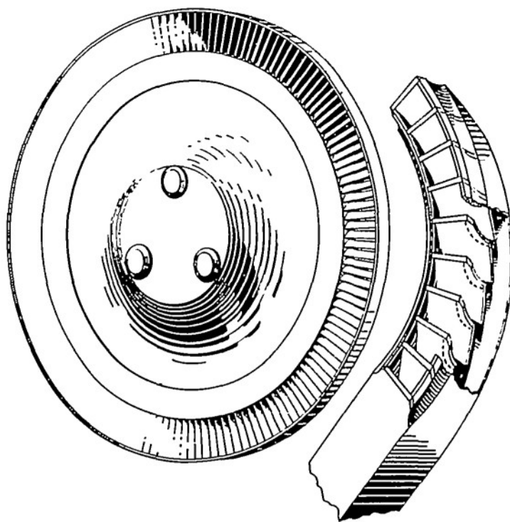
FIGURE 2.—Arrangement of guide vanes in blowdown-turbine nozzle box.
