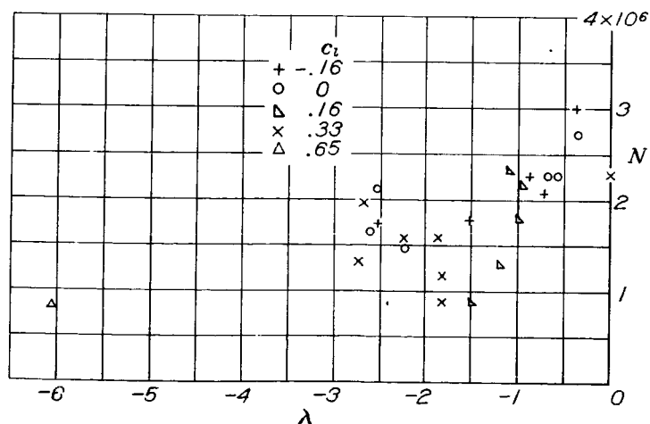
Figure 15.- Values of N and \lambda at the transition point for the 5-foot-chord N.A.C.A. 0012 metal-covered airfoil.
