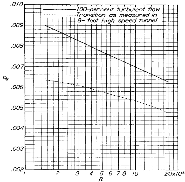
Figure 21.- Variation with Reynolds Number of the skin-friction drag coefficient for the N.A.C.A. 0012 airfoil. (From computations based on the 8-foot high-speed-tunnel transition measurements.) c_l = 0 .
