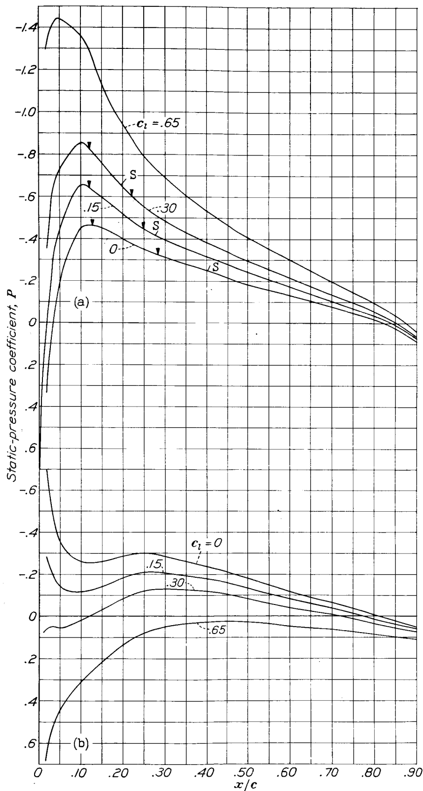
(a) Upper surface. The ticks indicate the location of the transition points for the extreme test Reynolds Numbers. Estimated laminar separation points are denoted by S. (b) Lower surface.
