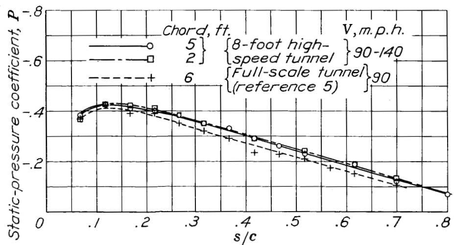
Figure 11 - The static-pressure distribution over the N.A.C.A. 0012 airfoils (corrected for constriction) compared with the results obtained in the full-scale wind tunnel. c_1 , 0.
