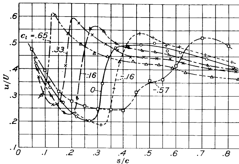
Figure 4.- Velocity in the boundary layer of the 5-foot-chord N.A.C.A. 0012 metal-covered airfoil 0.008 inch above the upper surface at a Reynolds Number of 6,550,000, showing transition at several lift coefficients.
