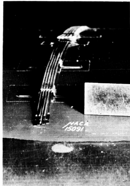
Figure 2.-Static and total-pressure tubes used in surveying the boundary layer of the 5-foot-chord N.A.C.A. 0012 airfoils.
