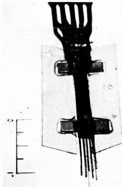
Figure 3.-Static and total-pressure tubes used in surveying the boundary layer of the 2-foot-chord N.A.C.A. 0012 airfoil. The tubes are approximately two-fifths the size of those used on the 5-foot-chord airfoils.
