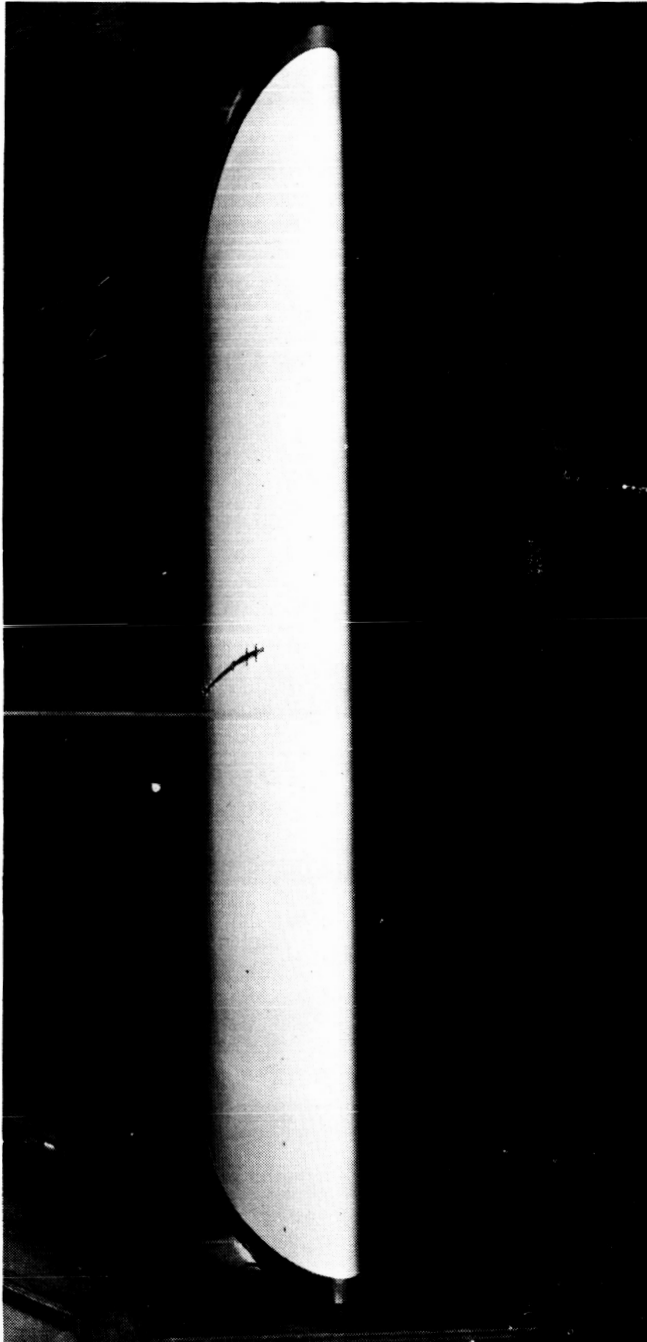
Figure 1.-The 5-foot-chord N.A.C.A. 0012 solid-wood airfoil mounted in the 8-foot high-speed wind tunnel, showing the method of installing the survey tubes.
