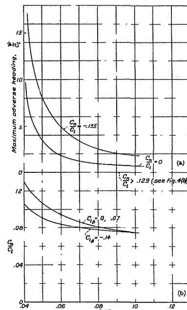
(a) \Gamma = 5^\circ . (b) \psi/C_l = 0 .
