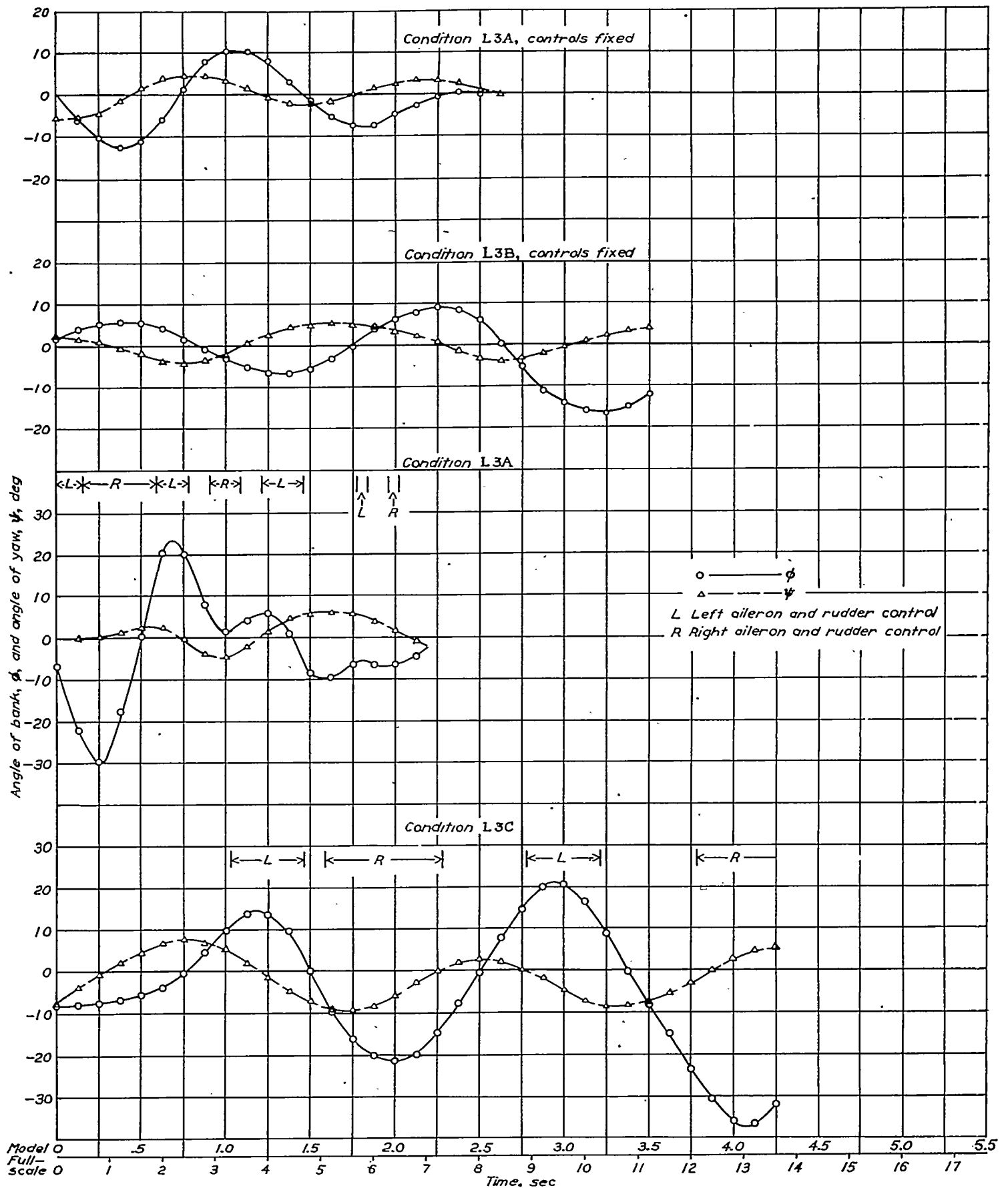
FIGURE 10.—Time histories of banking and yawing motions of model showing effect of increased moments of inertia on damping of lateral oscillation. Large positive dihedral. Vertical tail 3. C_L=1.0 .
