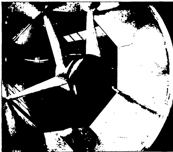
FIGURE 1.—Test section of NACA free-flight tunnel showing powered model in flight.
