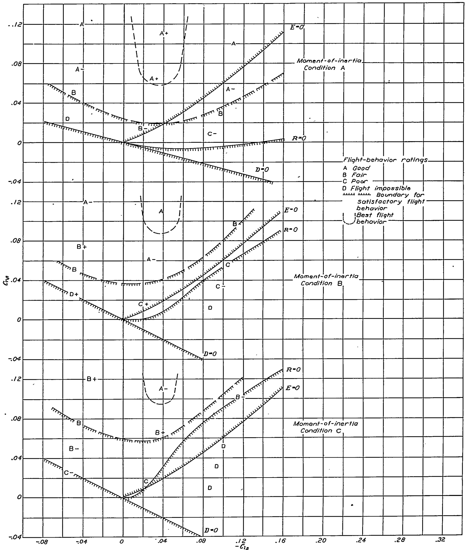
FIGURE 12.—Flight-behavior ratings for different test conditions. C_L=1.0 .
