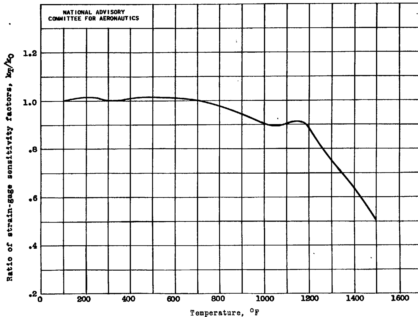
Figure 1. - Average variation with temperature of ratio of strain-gage sensitivity factor at elevated temperatures to strain-gage factor at room temperature for form-wound strain gages cemented with Sauereisen No. 78 cement.
