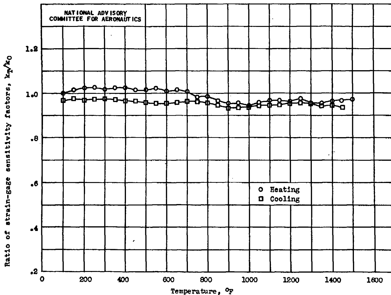
Figure 12. - Variation of ratio of strain-gage sensitivity factor at elevated temperatures to factor at room temperature with temperature for strain gages without winding forms cemented with Sauerbrey No. 1 cement.
