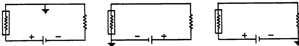
(a) Battery polarity in grounded circuits that operated satisfactorily at 1500° F.
