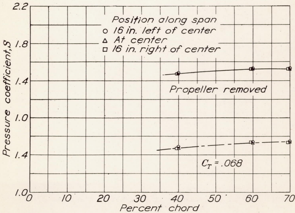
Figure 3.- Effect of pusher propeller on pressure distribution. N.A.C.A. 27-212 airfoil; C_L , approximately 0.2; R , 5,000,000
