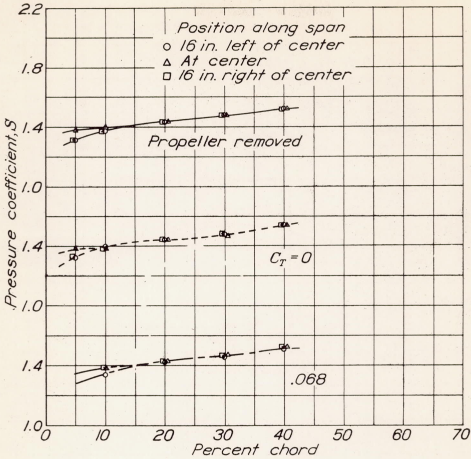
Figure 2.- Effect of tractor propeller on pressure distribution. N.A.C.A. 27-212 airfoil; C_L , approximately 0.2; R , 5,000,000
